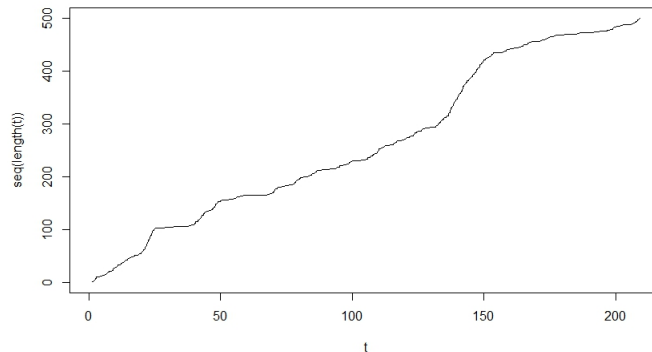
Figure 5.6: Empirical compensator for the Hawkes process with parameters \mu = 0.5 , \alpha = 0.8 , \beta = 1
