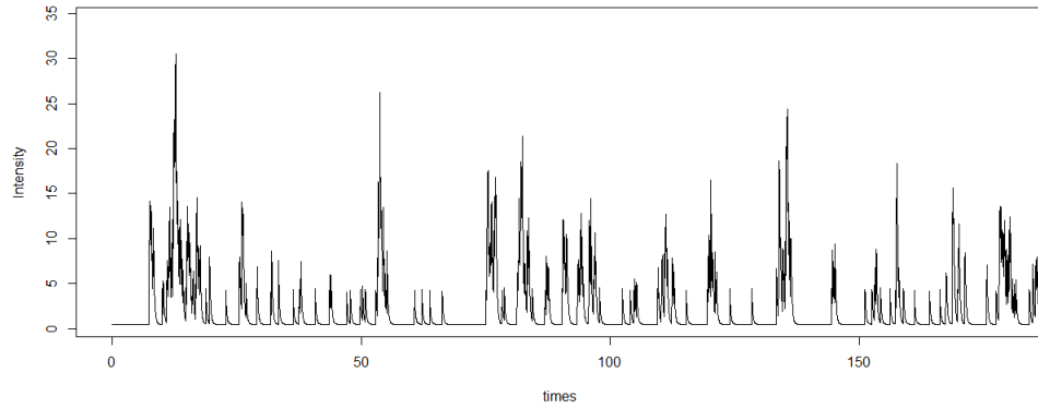
Figure 5.4: Representation of the intensity for \mu = 0.8 , \alpha = 0.5 and \beta = 1 .
