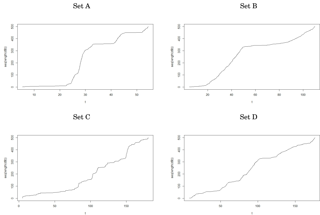
Figure 5.8: Empirical compensators of the PLC-SEPP for the different set of parameters values from table 5.2
