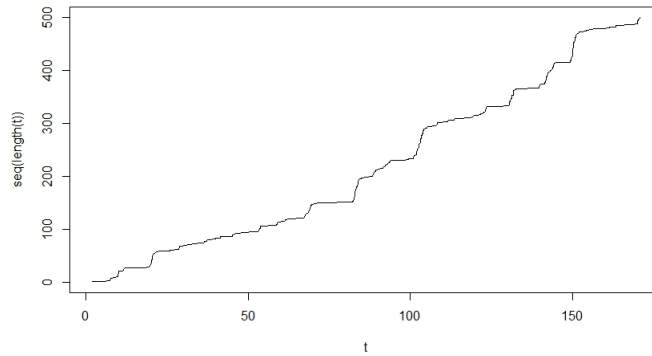
Figure 5.5: Empirical compensator for the Hawkes process with parameters \mu = 0.5 , \alpha = 4 , \beta = 5
