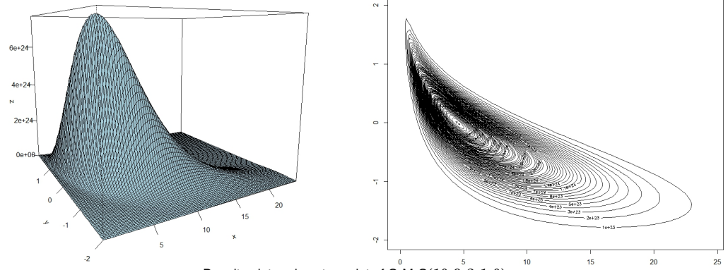
Density plot and contour plot of G-M-G(10, 9, 2, 1, 0)
