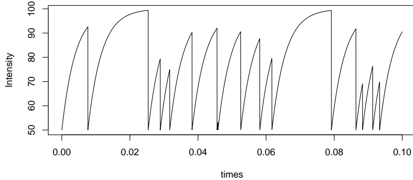
Figure 5.2: Intensity of a Mino process (inhibited) : \mu = 100 , \alpha = -0.5 , \beta = 250 et T = 0.1 ms
