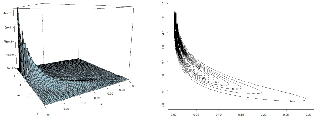
Density plot and contour plot of G-M-G(10, 17, 2, 1, 0)
