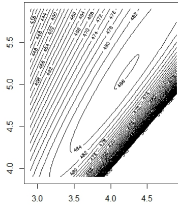
Contour plot of Hawkes log-likelihood
