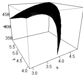
Density plot of Hawkes log-likelihood
