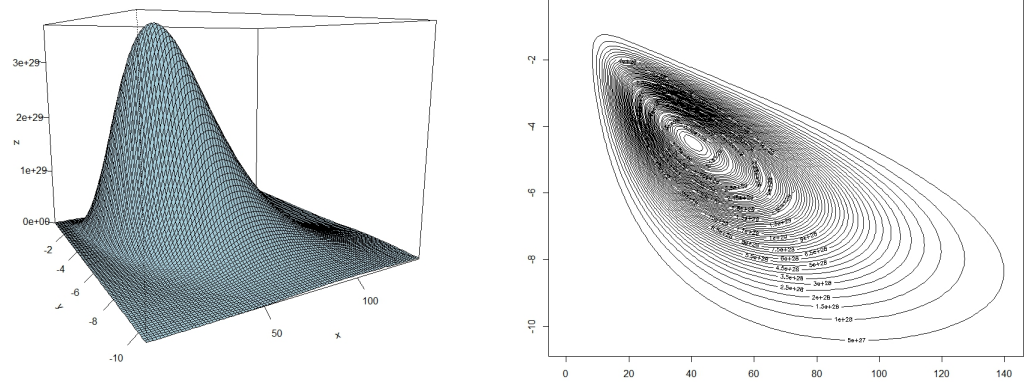
Density plot and contour plot of G-M-G(10, 2, 2, 1, 0)
