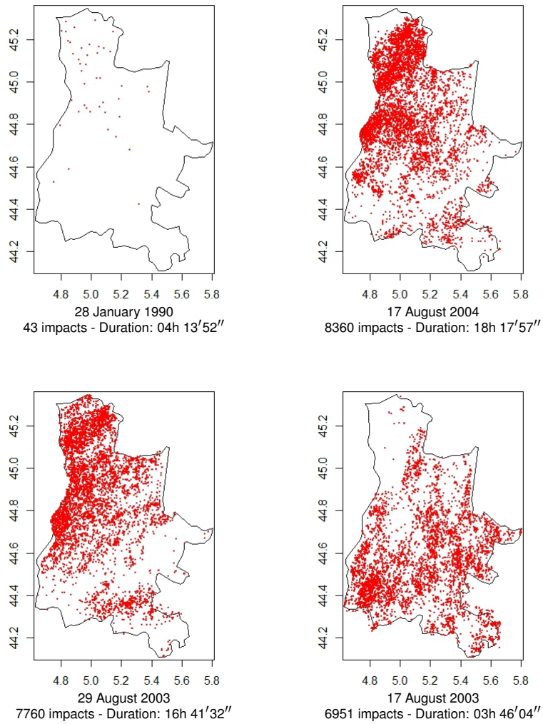
Figure 6.4: Impacts localization for groups in table 6.8
