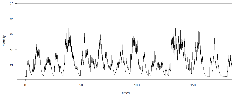
Figure 5.3: Representation of the intensity for \mu = 0.5 , \alpha = 4 and \beta = 5 .
