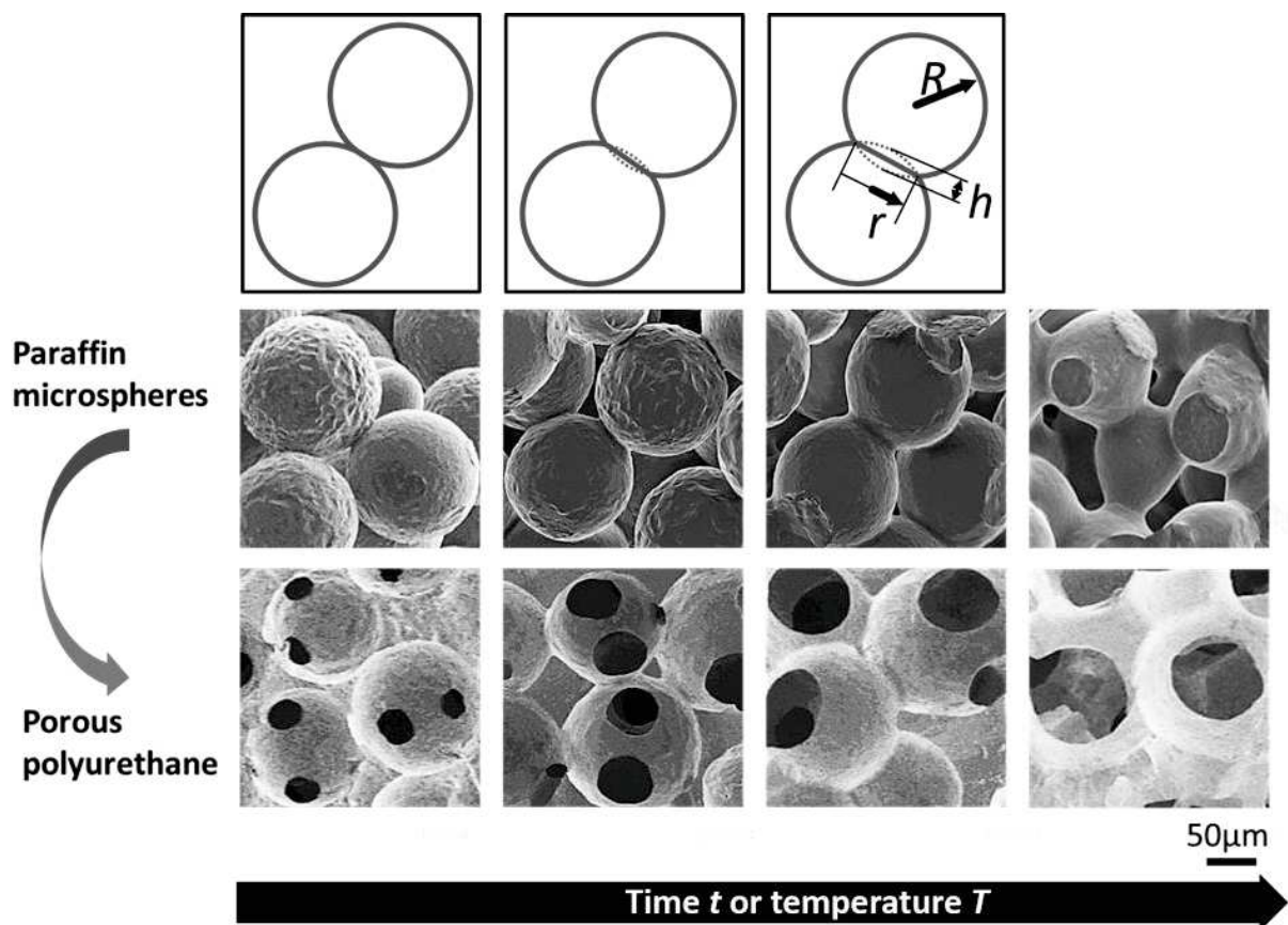
Figure 3-1: Examples of SEM images of paraffin beads (central row) showing the increase of interconnection radius r with increasing sintering time t or temperature T . The bottom row shows the macroporous polyurethanes obtained from moulding the sphere template. The top row sketches the deformation of two contacting spheres together with the variables used in this article.
