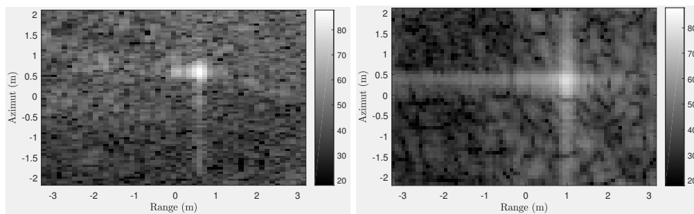
Figure 1.9: Left: SAR image amplitude (dB). Right: Coefficient amplitude of a 3 \times 3 decomposition using STFT (dB).
