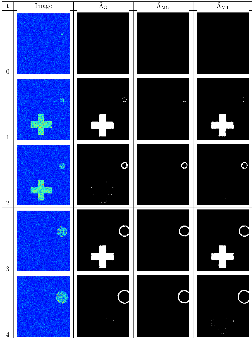
Figure 4.5: Estimation/Detection results at P_{FA} = 10^{-3} for synthetic Gaussian data ( p = 5 , N = 25 , T = 5 ). A change-point detected and estimated corresponds to non-zero value on the resulting image.
