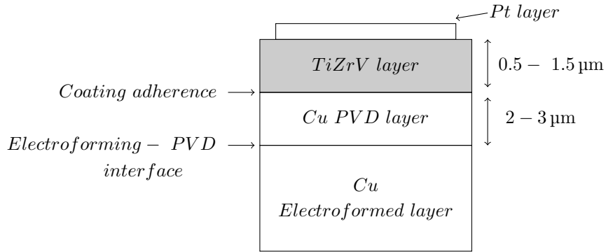
Figure 4.20. Schematic of coating layers analyzed with FIB combined with SEM.
