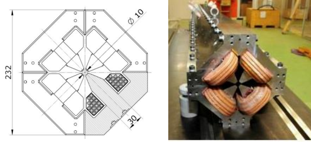
Figure 1.11. CLIC main beam quadrupole magnet [35].
