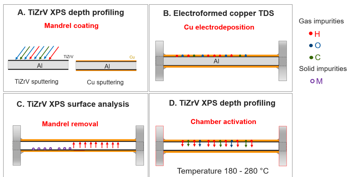
Figure 5.1. Diagram of the possible sources of impurities. Gas impurities (C, O and H) and solid impurities (M) are represented in each respective color. The different methods used for the characterization are highlighted for each step of the process (A: Coating of the mandrel, B: Electroforming step, C: Mandrel etching, D: Chamber activation).
