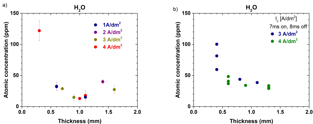
Figure 5.12. \text{H}_2\text{O} concentration (at. ppm) versus electroplated thickness for the (a) DC electroformed copper and (b) PC electroformed copper, at different current densities (for the pulse plated with t_{on}=7\text{ms} , t_{off}=8\text{ms} and given peak current density J_c ).
