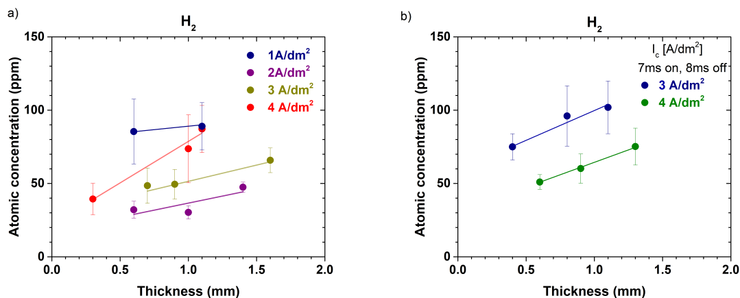
Figure 5.11. \text{H}_2 concentration (at. ppm) versus electroplated thickness for the (a) DC electroformed copper and (b) PC electroformed copper, at different current densities (for the pulse plated with t_{on}=7\text{ms} , t_{off}=8\text{ms} and given peak current density J_c ).
