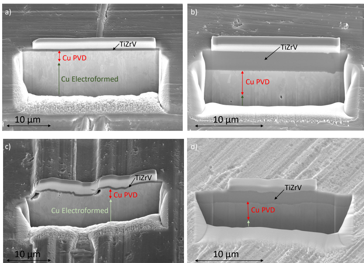
Figure 4.21. FIB combined with SEM pictures of TiZrV thin films on copper electroplated substrate after aluminum etching with NaOH 5 M. In (a) 0.5 \mu\text{m} TiZrV film and in (b) 1.5 \mu\text{m} TiZrV film. FIB pictures of TiZrV thin films on copper electroplated substrate after interlayer copper etching with ammonium persulfate. In (c) 0.5 \mu\text{m} TiZrV film and in (d) 1.5 \mu\text{m} TiZrV film.
