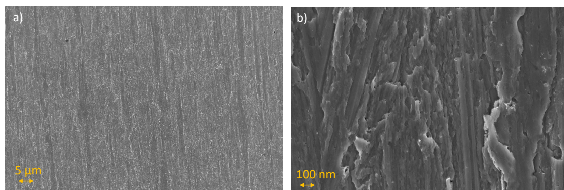
Figure 4.18. SEM pictures of TiZrV thin films prepared with the Cu/NEG/mandrel scheme after aluminium etching with NaOH 5 M and acidic rinsing at (a) lower magnification (b) higher magnification.
