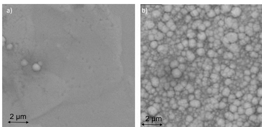
Figure 1.8. SEM micrographs of TiZrV coatings sputtered on a smooth copper surface at 100 °C (a) and at 250 °C (b). From Prodromides [24].
