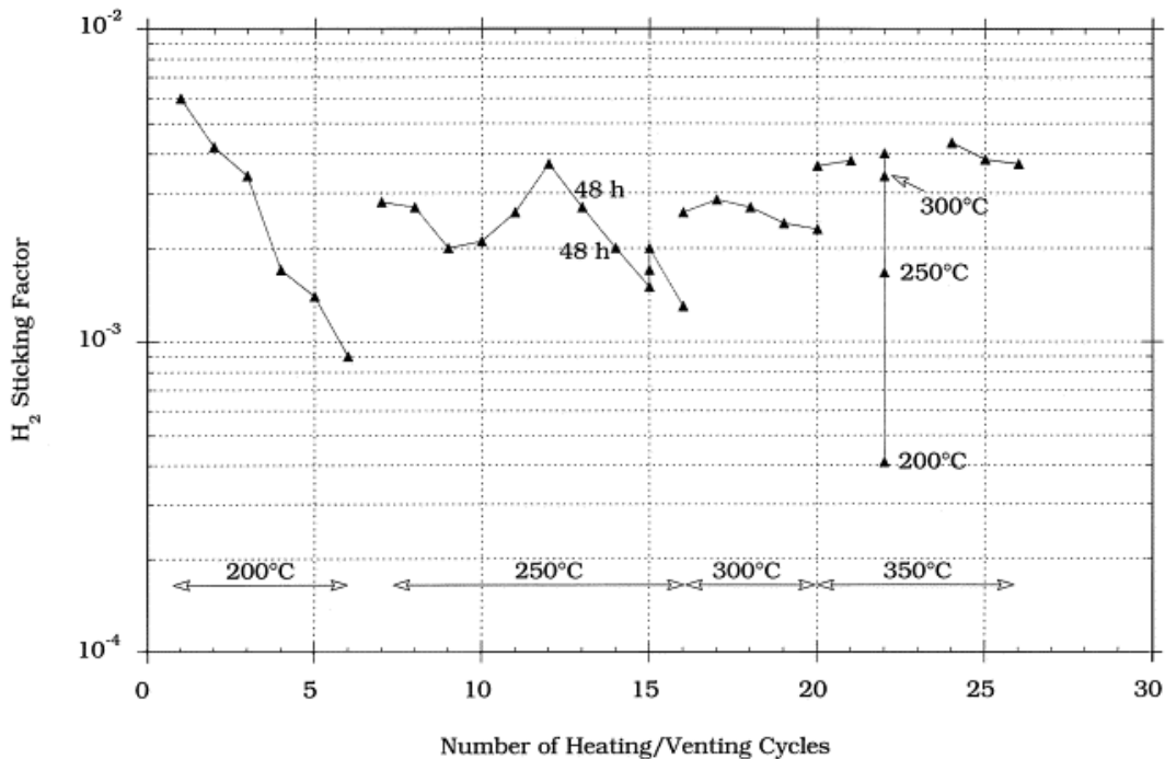
Figure 1.10. Variation of the H_2 sticking factor for a 5\ \mu\text{m} thick TiZrV coating as a function of the number of activation-air venting cycles. The activation applied during 24 hours progressively increased to compensate for the decrease of sticking factor. From Benvenuti et al. [26].
