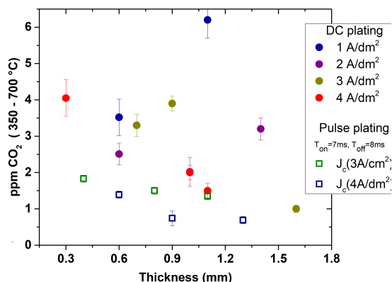
Figure 5.14. Concentration of \text{CO}_2 (at. ppm) which are outgassed between (350 - 700 °C) versus electroplated thickness for the DC electroformed copper (represented as a circle) and PC electroformed copper (represented as a square), at different current densities (for the pulse plated with t_{on}=7\text{ms} , t_{off}=8\text{ms} and given peak current density J_c ).
