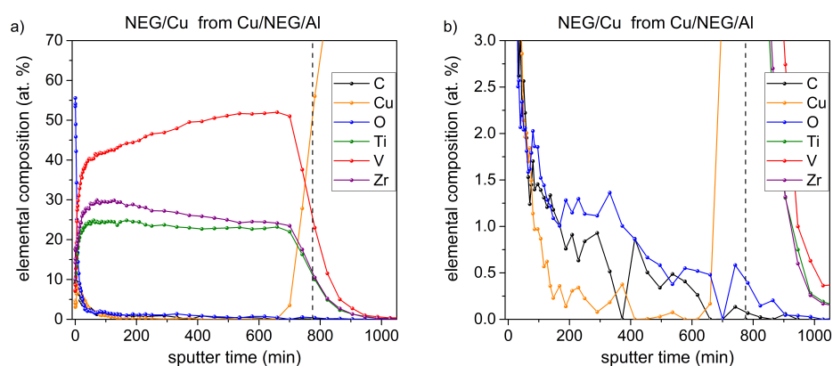
Figure 5.6. Elemental composition as a function of sputtering time, for the reverse NEG sample after mandrel removal. In (a) full scale is represented and in (b) the scale is enlarged for the comparison of impurities.
