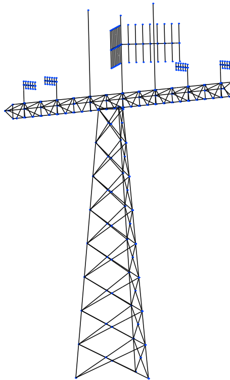
Fig. 4.9.: Wire-discretized antenna structure.
