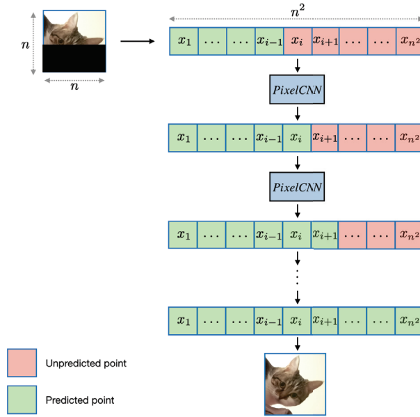
Fig. 2.10 Illustration of the generation procedure for PixelCNN. An n \times n image is reashedaped to an n^2 vector, and each predicted pixel is fed back as input for predicting the next pixel.
