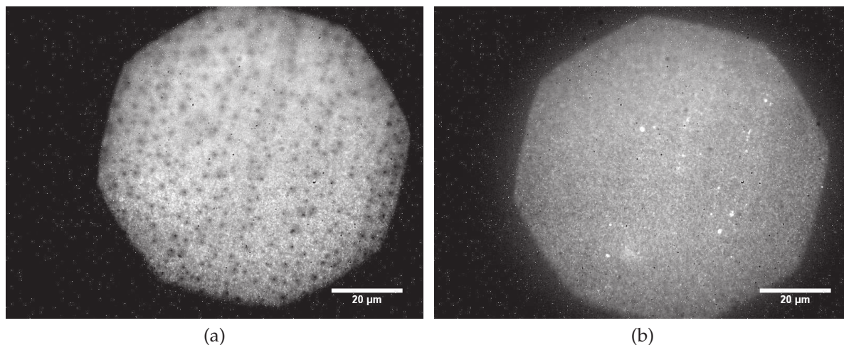
Figure III.2.32 – Fluorescence microscopy images of a DPPC single bilayer after BR reconstitution at room temperature: (a) lipids visualised, (b) proteins visualised. A 1 \mu\text{g/ml} BR in 0.05 \text{ mM} DDM PBS buffer solution was used for the BR reconstitution.
