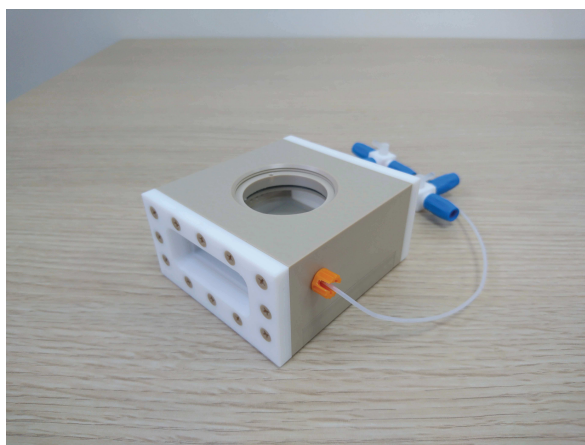
Figure II.2.13 – Solid/liquid cell for X-ray reflectometry experiments at the synchrotron.
