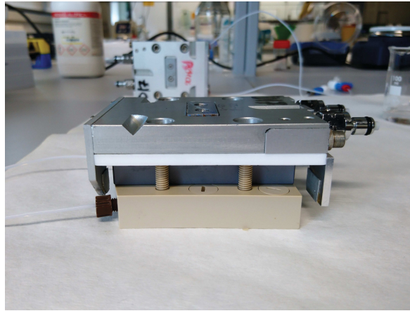
Figure II.2.24 – Solid/liquid cell used for the neutron reflectivity measurements.
