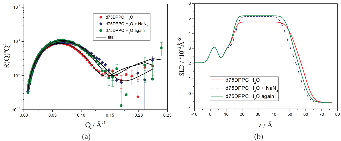
Figure III.3.14 – (a) Reflectivity curves for the d_{75} DPPC bilayer in H_2O contrast; in H_2O contrast with 1 mM NaN_3 and after rinsing with H_2O again. A clear change of the structure of the bilayer is observed due to the presence of NaN_3 . (b) SLD profiles obtained from the fits.
