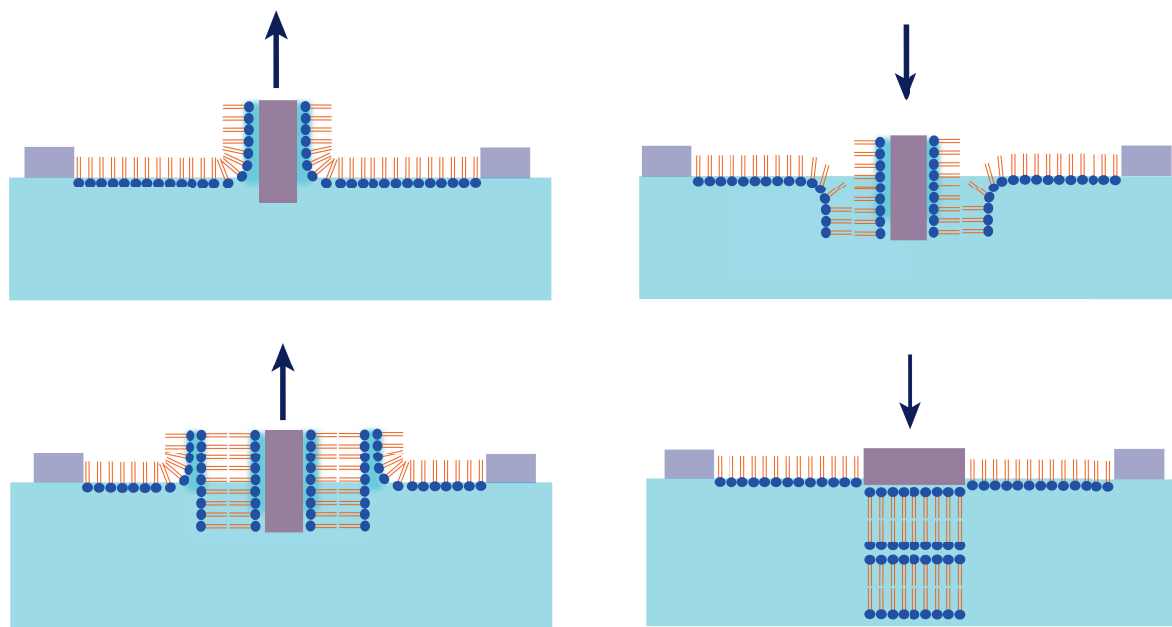
Figure II.1.8 – Schematic illustration of Langmuir-Blodgett, Langmuir - Schaefer (LB/LS) deposition techniques.
