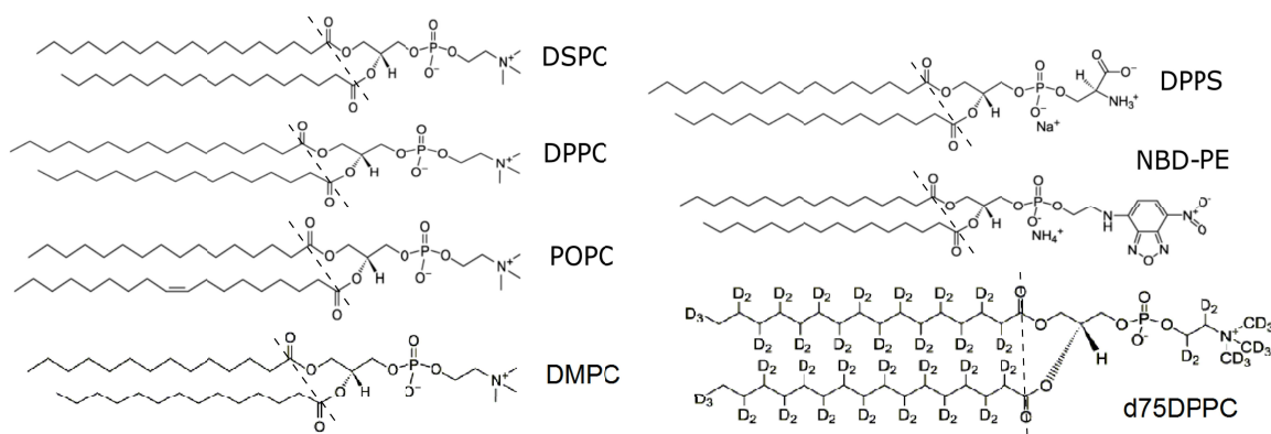
Figure II.1.2 – Chemical structure of phospholipids used in this thesis. The hydrophobic and hydrophilic regions are defined by the dotted lines [51].
