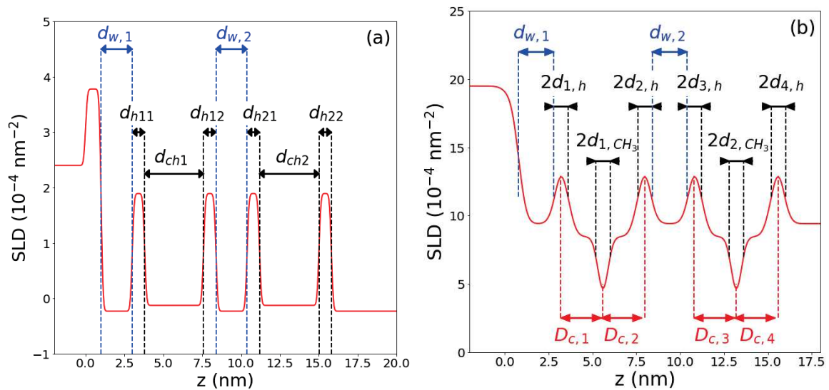
Figure VII.B.1 – (a) Definition of the parameter used for SLD profile in case of NR. For sake of clarity we used artificial values for \sigma_{i,j} , d_{w,1} and d_{w,2} ( \sigma_{i,j} = 0.1 \text{ nm} , d_{w,1} = 2 \text{ nm} , d_{w,2} = 2 \text{ nm} ). (b). Definition of the parameter used for SLD profile in case of XR (1G-hybrid model). For sake of clarity we used artificial values for d_{w,1} and d_{w,2} ( \sigma_{i,j} = 0.1 \text{ nm} , d_{w,1} = 2 \text{ nm} , d_{w,2} = 2 \text{ nm} )
