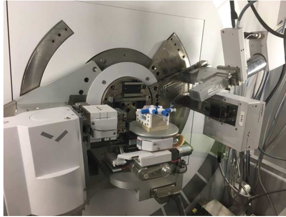
Figure II.2.32 – In-house Empyrean X-ray bench available at the ILL.
