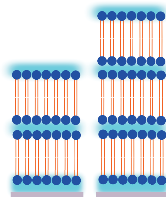
Figure IV.2.1 – Schematic illustration of the double (a) and triple (b) lipid bilayer systems investigated within this project.
