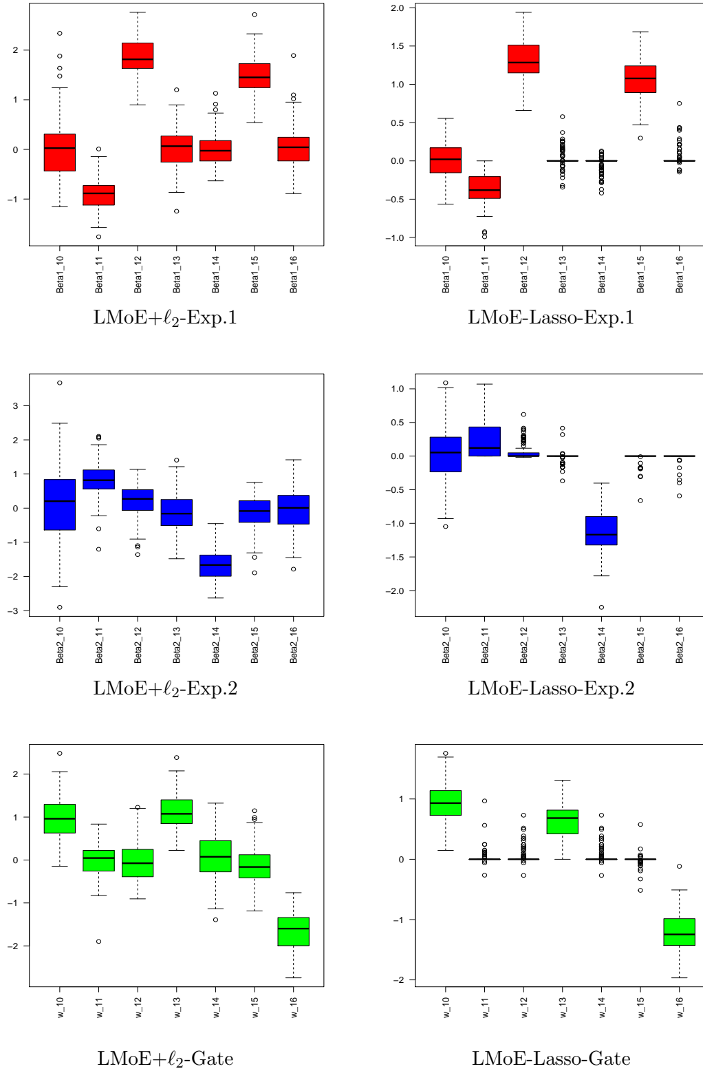
Figure 4.3: Boxplots of \ell_2 regularized MoE model (LMoE+l 2 ) and the proposed Lasso penalized MoE model (LMoE-Lasso) for logistic case.
