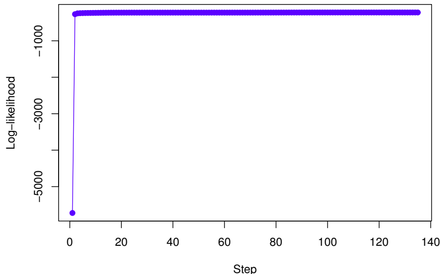
Figure 4.10: The penalized log-likelihood during the EM iterations when fitting the LMoE-Lasso model to the Musk-1 data.
