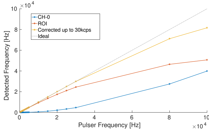
Figure 7.9: Dead-time correction.
