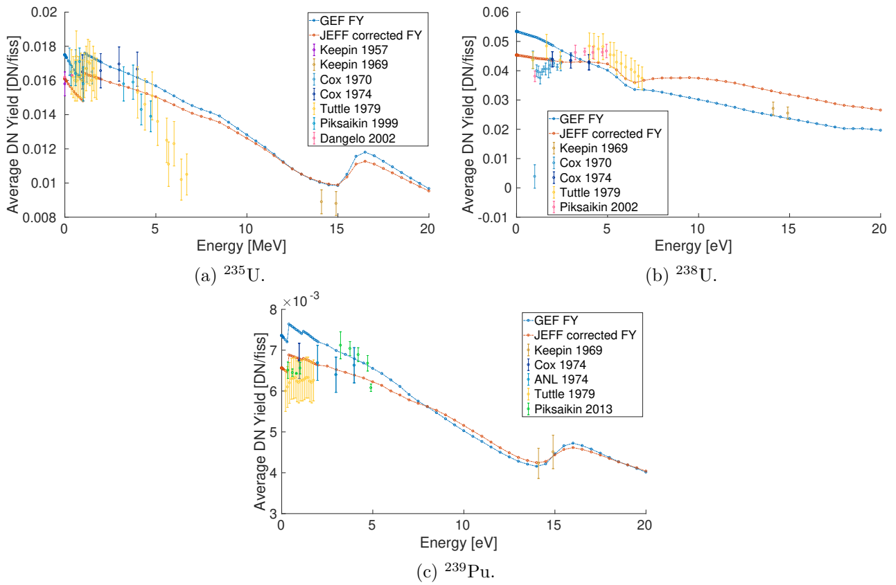
Figure 3.13: Energy dependence of average delayed-neutron yield computed with GEF-6.1 FY and with JEFF-3.1.1 FY modified with GEF-6.1 energy dependence. Experimental values are reported for comparison.
