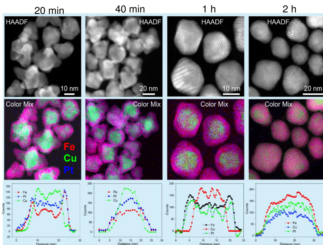
Fig. 5.5 STEM-HAADF image and elemental mapping image of FePtCu nanoparticles prepared at 20 min, 40 min, 1 h and 2 h, respectively. In the middle, it is according colour-mix image of STEM-EELS mapping, red colour is Fe, green colour is Cu and blue colour is Pt. The bottom spectra are line profiles crossing the single FePtCu nanoparticle at various reaction time.
