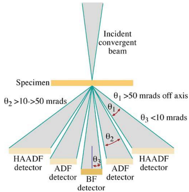
Fig. 2.8 The various electron detectors in a STEM. 151
