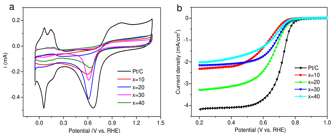
Fig. 4.3 a) CV curves of (\text{FePt})_{100-x}\text{Cu}_x and commercial Pt/C at 50 mV/s in \text{O}_2 saturated 0.5\text{ M H}_2\text{SO}_4 electrolyte, and (b) ORR polarization curves.
