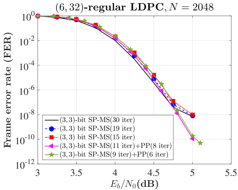
Fig. 5.15 FER performance of the (3,3)-bit SP-MS decoder with post-processing obtained by FPGA emulation for the IEEE 802.3 LDPC code.
