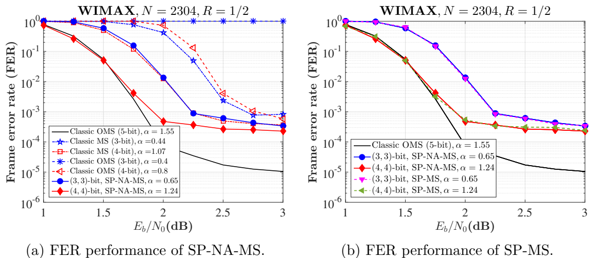
Fig. 4.10 FER performance for the WIMAX LDPC code with R = 1/2 .
