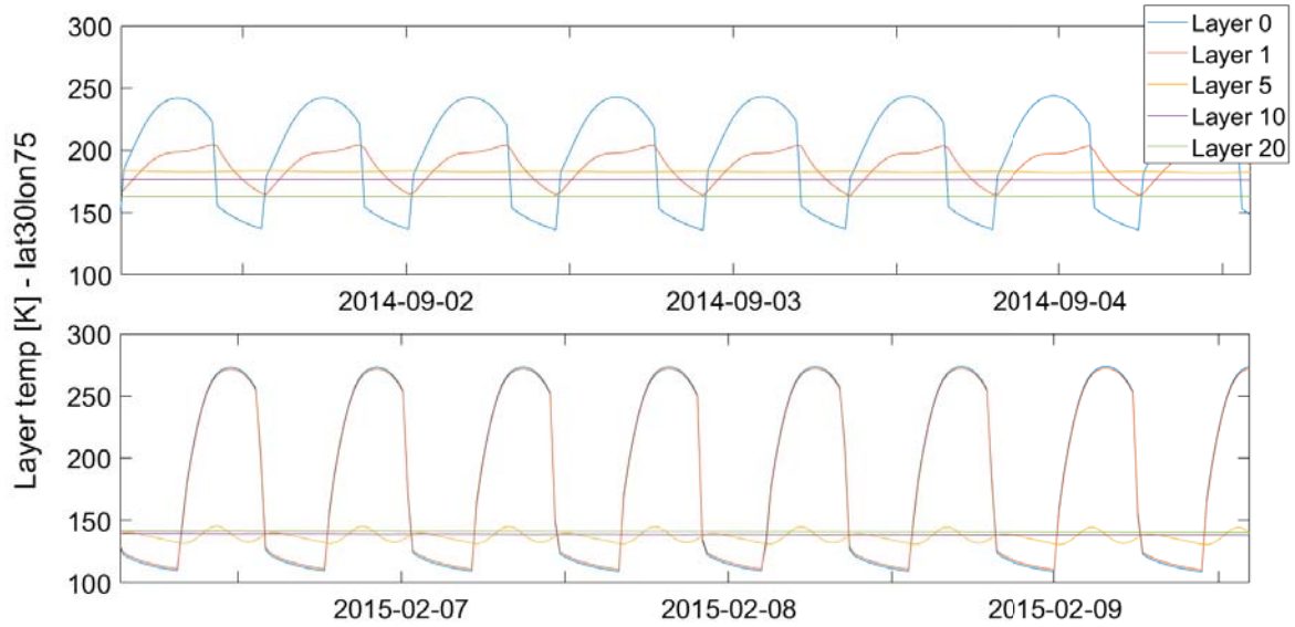
Figure 12.6: Temperatures at different depths for the point of latitude 30 and longitude 75 during 5 days at 3.4 AU (upper panel) and 5 days at 2.3 AU (lower panel) in case dust 1.
