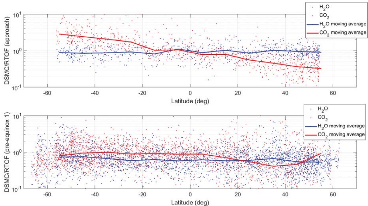
Figure 10.5: DSMC/RTOF ratio for \text{H}_2\text{O} and \text{CO}_2 for the approach (upper panel) and pre-equinox 1 (lower panel), with their corresponding sliding average (solid lines).
