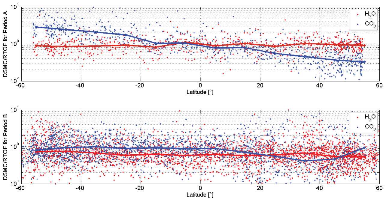
Fig. A.2. DSMC/RTOF ratio for H 2 O and CO 2 for Period A ( upper panel ) and Period B ( lower panel ).
