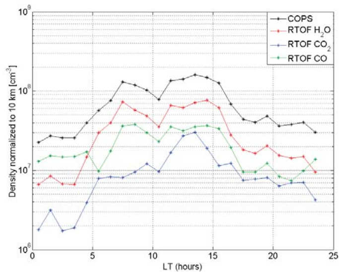
Figure 7.4: Total density from COPS, as well as the \text{H}_2\text{O} , \text{CO}_2 , and \text{CO} densities from RTOF during the approach as a function of the local time. Densities were normalised at a constant 10 km altitude.
