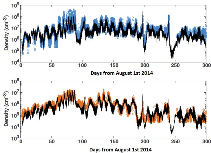
Figure 10.2: Density measured by DFMS (H 2 O in blue and CO 2 in orange) and the DSMC density extracted at the location of spacecraft (in black) (Fougere et al., 2016).
