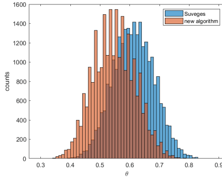
Figure 2: Comparison on the distribution of \theta with the two estimates. The blue distribution is obtained using the Süveges estimate and the red one using \hat{\theta}_5 (taking for both as a threshold the 0.99-quantile of the observable distribution).
