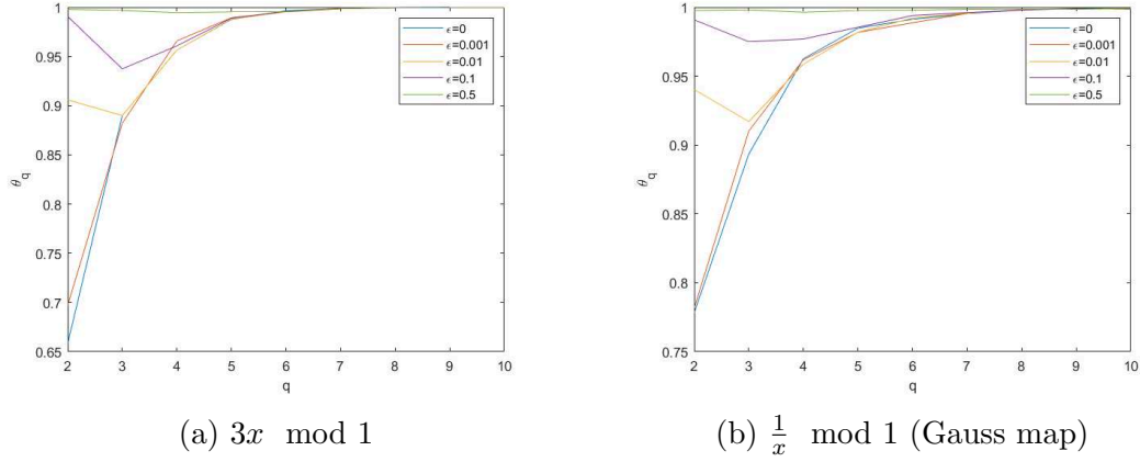
Figure 19: Influence of the intensity of noise \epsilon on the \theta_q spectrum for maps of the circle perturbed by uniform noise. We used the Süveges estimate, as mentioned in the text.
