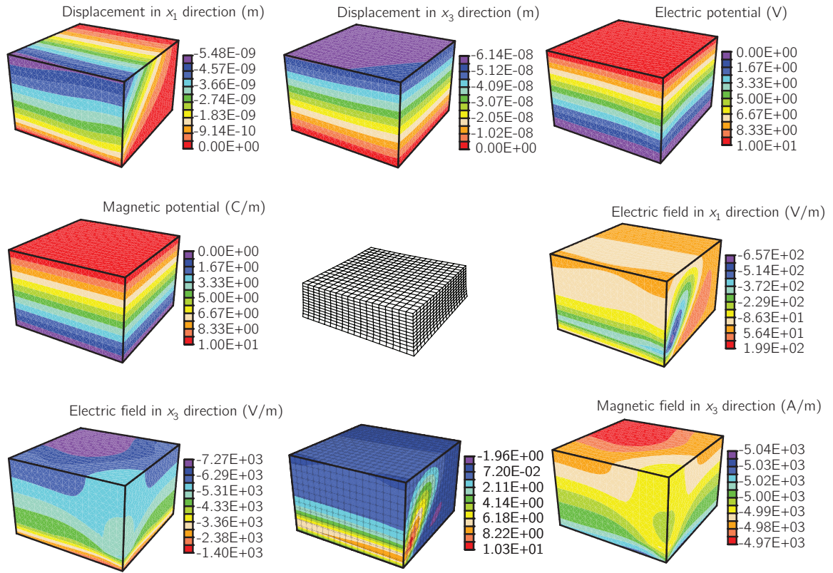
Figure 2.7: Displacement in directions x_1 and x_3 and deformed configuration amplified 10^5 .
