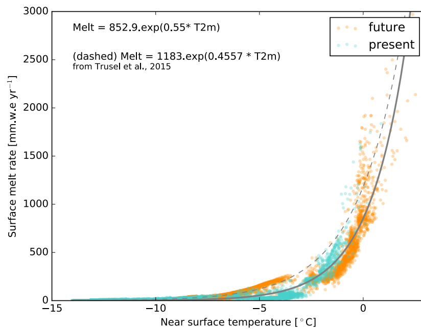
Figure 7 : Relationship between mean summer surface air temperature (T2m) and surface melt rate over the seven ice shelves from Getz to Abbot. The solid line represents the corresponding exponential fit. The dashed line represents the exponential fit found by Trusel et al., (2015) for 48 Antarctic ice shelves.
