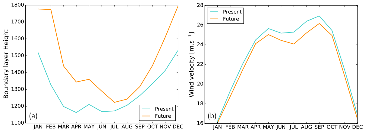
Figure 13 : (a) Boundary layer height (meter) (b) and wind velocity (m s -1 ) for the present simulation (blue) and the future (orange) simulation, over the seven major ice shelves from Getz to Abbot.
