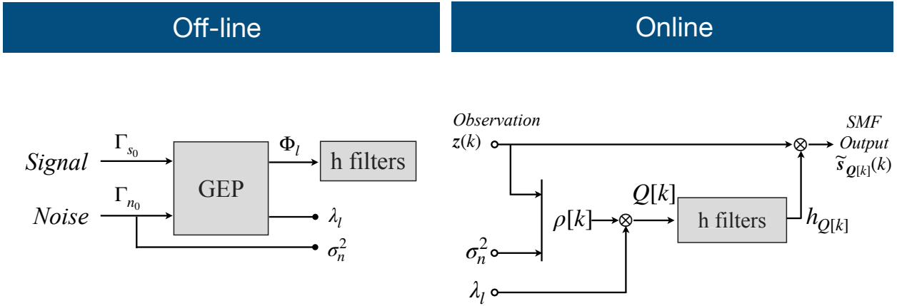
Figure 3.2: Scheme of classical SMF processing, as a succession of offline and online processes.
