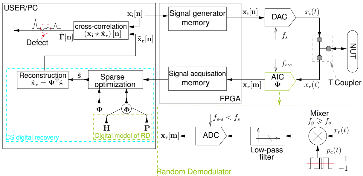
Figure 4.1: The proposed compressive sampling architecture of reflectometry with RD. Where in the digital model of RD, P represents the \pm 1 values of PRBS and H represents the impulse response of the low-pass filter as well as the sub-sampling. Not that m \in \{1 \dots M\} and n \in \{1 \dots N\} .
