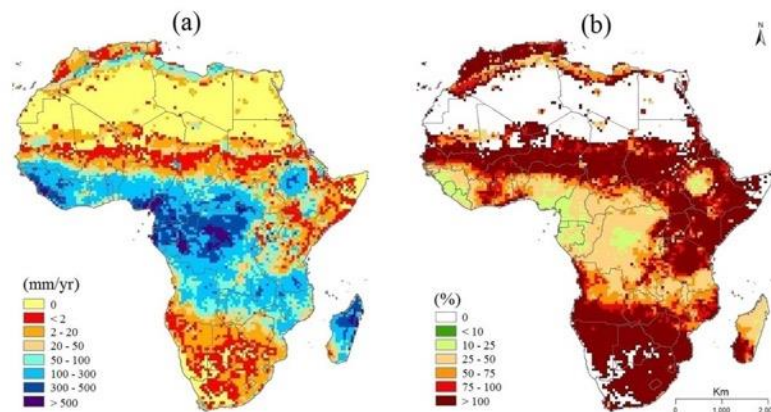
Figure 8. Average annual recharge ( \text{mm year}^{-1} ) and (b) its coefficient of variation (%), both over the period 1960–2000 (data from Van Beek et al., 2011).
