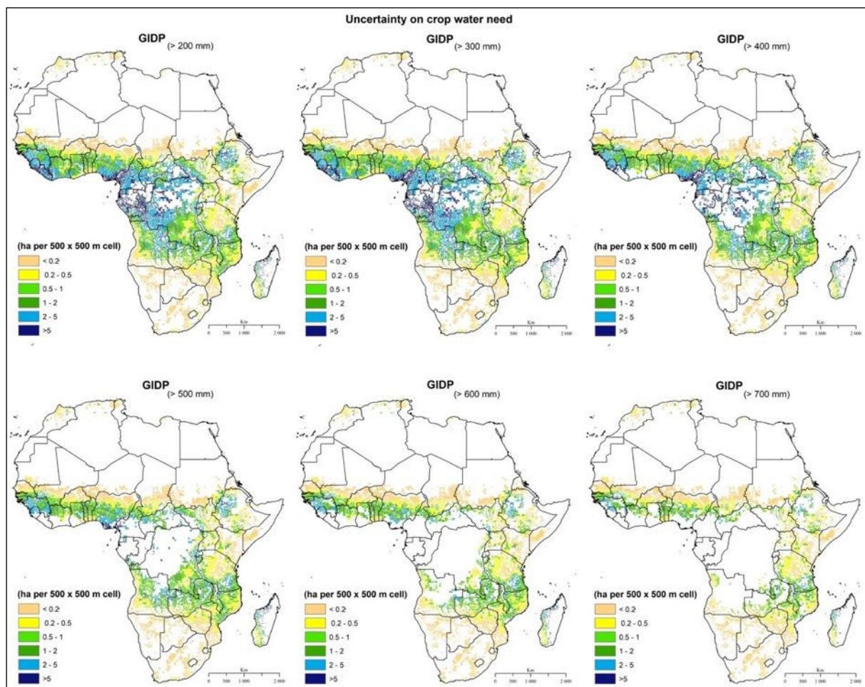
Figure A.3.1: Sustainable groundwater irrigation development potential (GIDP) expressed in hectare per cell at a resolution of 0.005° (cell area about 25 ha) and estimated from several threshold value for the crop water need starting from 200 mm to 700 mm with 100 mm incrementation.
