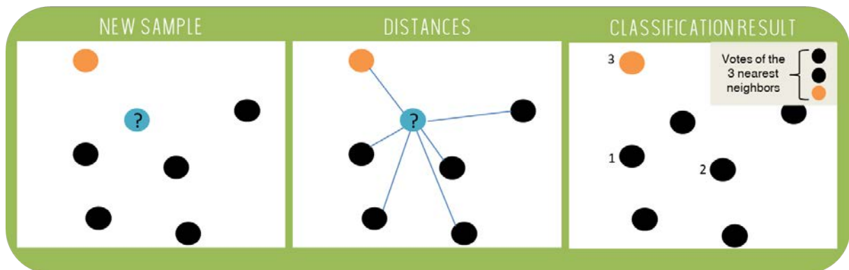
Figure 3.10 – Example of K-nearest neighbors classification with k = 3 .
