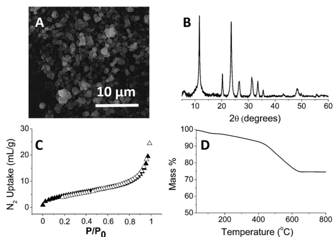
Figure 1. Characterizations of Fe-BTP by SEM (A), PXRD analysis (B), N 2 -uptake (Adsorption is represented with filled triangles and desorption with open triangles) (C) and TGA (D)
