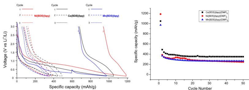
Fig. 3. (left) Charge-Discharge profiles (right) and cycling performance (reduction) at 300 \text{ mA}\cdot\text{g}^{-1} .
