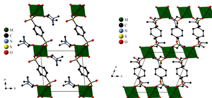
Fig. 2. (left) Projection of the \text{Mn}(\text{BDS})(\text{DMF})_2 crystal structure down the c axis. (right) View of the \text{Mn}(\text{BDS})(\text{DMF}) structure down the b axis.
