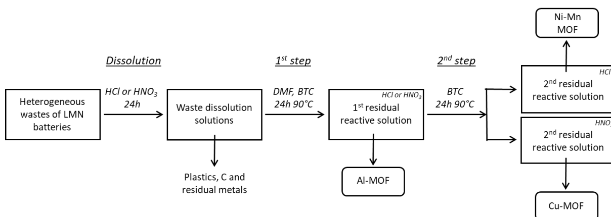
Figure 6 : Flow chart of the recycling method of Li-ion batteries
