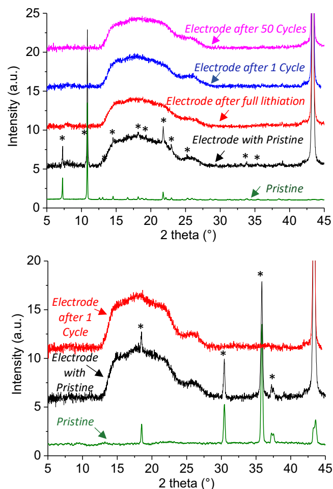
Fig. 3 Ex situ XRD patterns of MOF (top) and oxide (bottom). Asterisks highlight the MOF and oxide diffraction peaks
