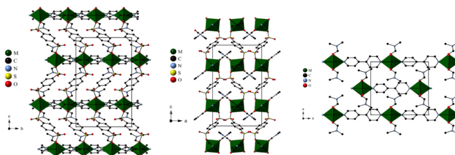
Fig. 1. left – Projection of the M(\text{BDS})(\text{bpy})(\text{DMF})_2 crystal structure down the a axis, middle – crystal structure down the b axis, right – Arrangement of the isolated \text{MO}_4\text{N}_2 octahedra viewed perpendicular to the [001] direction.
