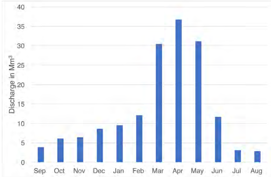
FIGURE 4.2 – Mean monthly discharge of the Ourika river at Aghbalou (1970-2003 (Agence Japonaise de coopération internationale, 2008)).
