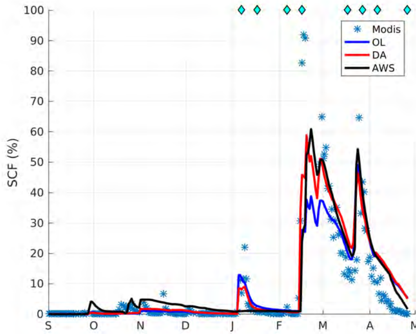
FIGURE 5.12 – Comparison of the simulated and observed snow covered fraction of the Rheraya catchment (cSCF) at the daily time step. The blue diamonds in the upper part of the figure indicate the date of the assimilated Sentinel-2 observations.
