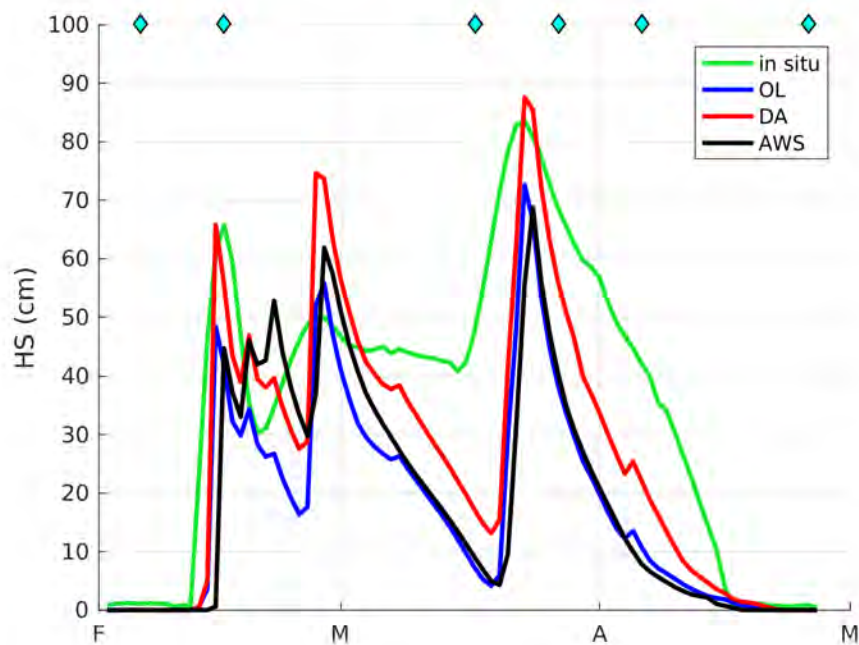
FIGURE 5.11 – Comparison of the simulated and observed in situ snow height in Oukaimeden at the daily time step. The blue diamonds in the upper part of the figure indicate the date of the assimilated Sentinel-2 observations.
