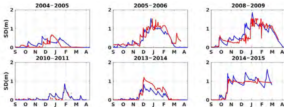
FIGURE 4.5 – Time series of the simulated (blue) and observed (red) daily snow depth (SD) at Oukaimeden.
