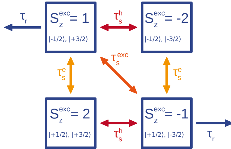
Figure 1.12: The four different exciton states (denoted S_{exc}^z ). Notations |\pm 1/2\rangle , |\pm 3/2\rangle spell out the spin state of the electron and the hole in each cases. The different spin relaxation mechanisms within an exciton are represented by double arrows. Radiative recombination of bright states is represented by blue arrows.
