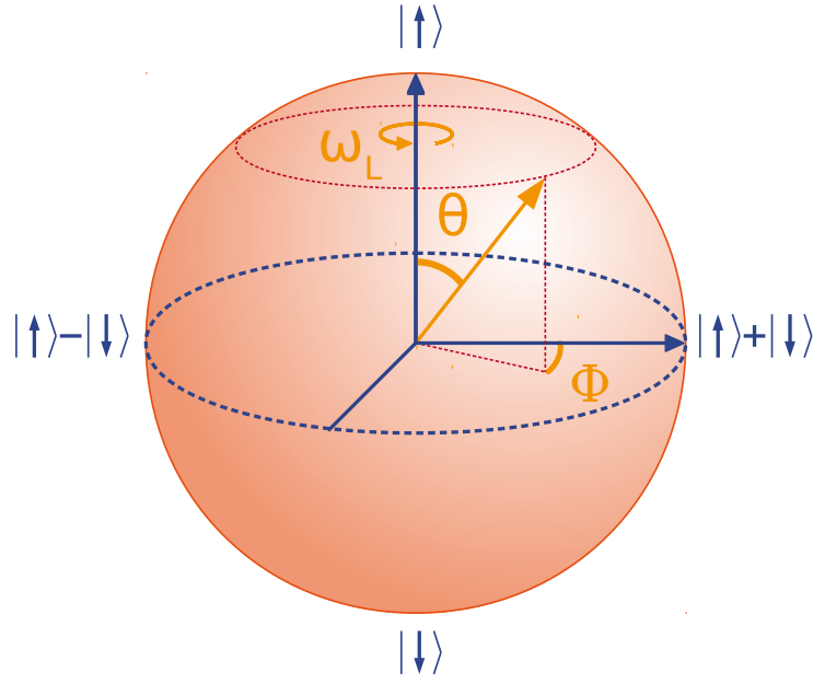
Figure 1.3: Larmor precession of an arbitrary spin state visualised on the Bloch sphere. The magnetic field is vertical. The two eigenstates |\uparrow\rangle and |\downarrow\rangle are respectively at North and South pole and two other remarkable states are shown to browse the Bloch sphere.
