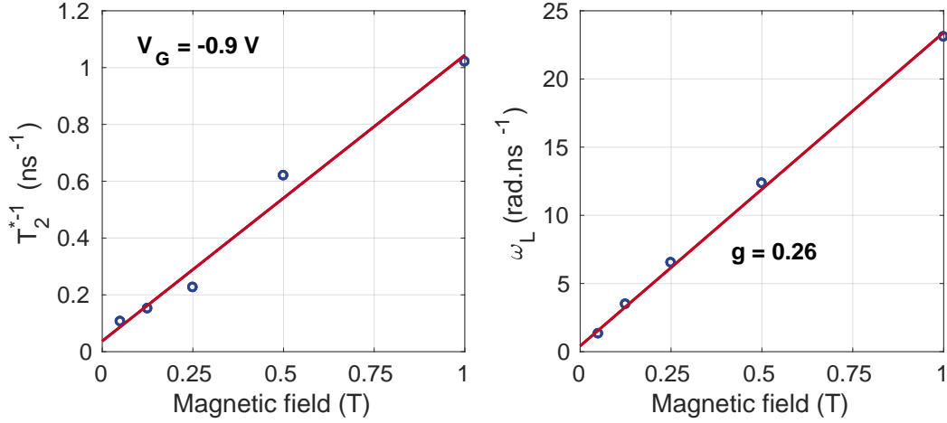
Figure 4.21: Determination of T_2^* and g -factor from field dependence of T_2^* and \omega_L . Blue circles are Larmor frequencies (right panel) and inverse of T_2^* decay times (left panel) from fits for all values of B at V_G = -0.9 \text{ V} . Red solid lines are linear fits.
