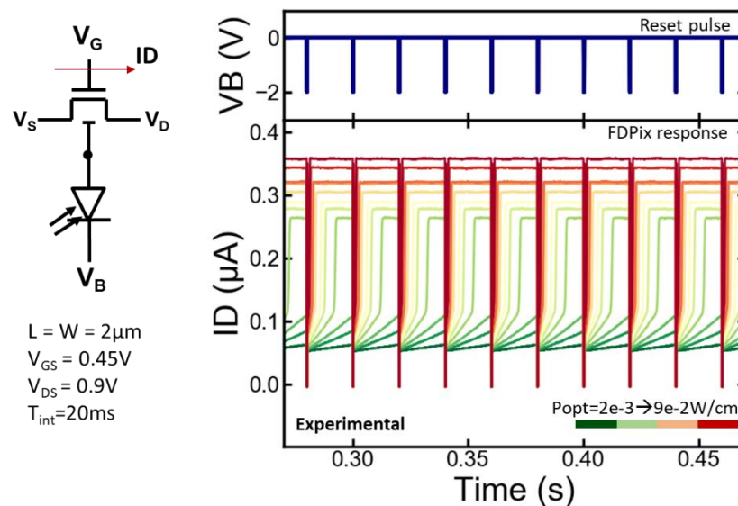
Figure 3-24: FDPix drain current monitoring while applying constant light at different intensities at 50 fps
