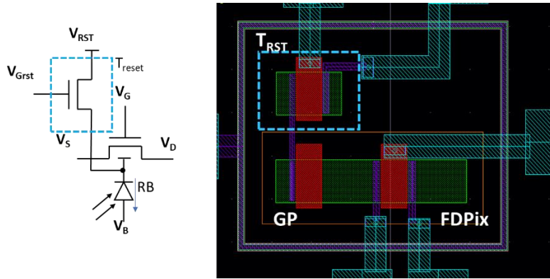
Figure C-1: schematic and layout of 2T FDPix w/ reset transistor
