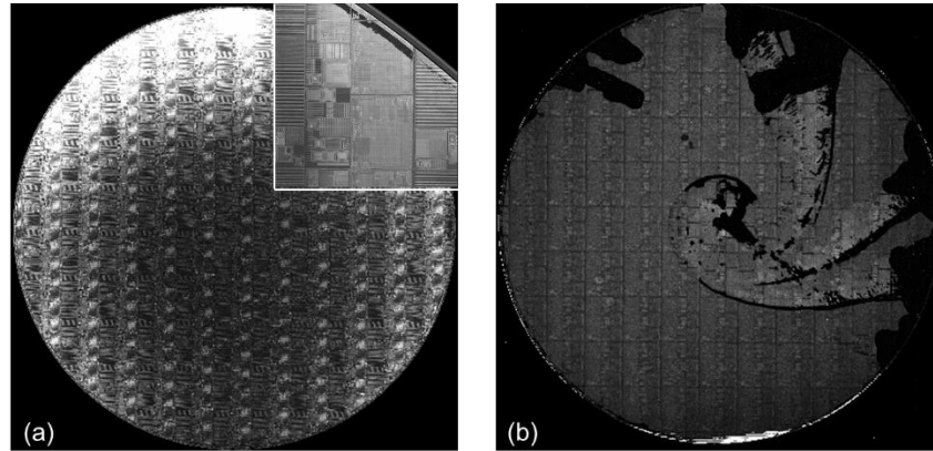
Figure 4-19: back thinning using grinding on FDSOI wafers a) after bonding of handle wafer b) after back thinning (target 150 \mu\text{m} )
