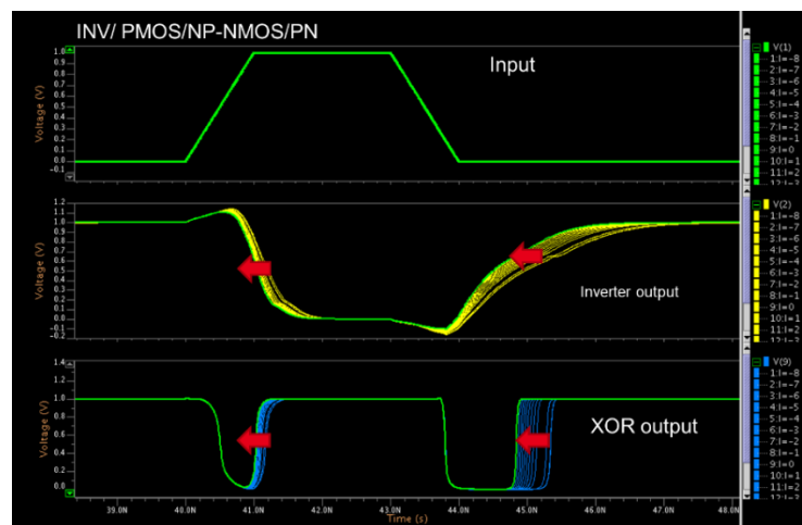
Figure C-4: single inverter PWM-based FDPix SPICE simulation results
