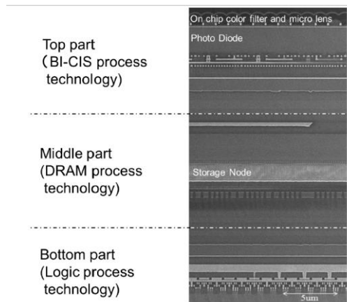
Figure 1-17: 3-level stack image sensor [HARUTA 2017]
