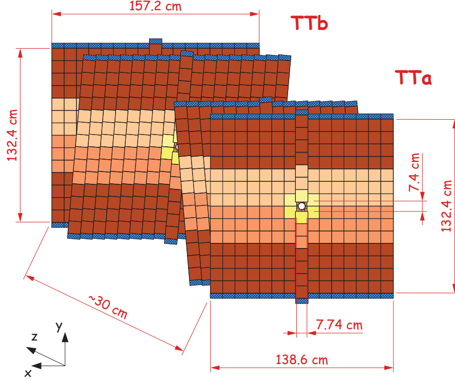
Figure 2.6: Scheme of the four TT stations.
