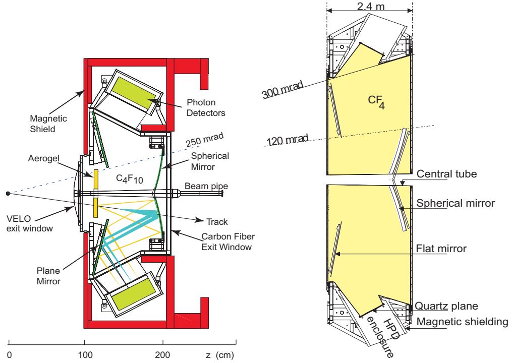
Figure 2.13: Schematic view of the RICH1 (left) and RICH2 (right) detectors. The different radiators and the optical systems are also shown.
