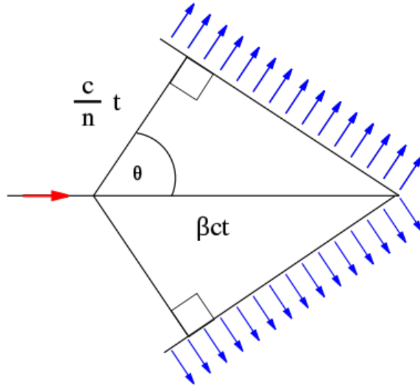
Figure 2.12: Geometric representation of the Cherenkov emission.
