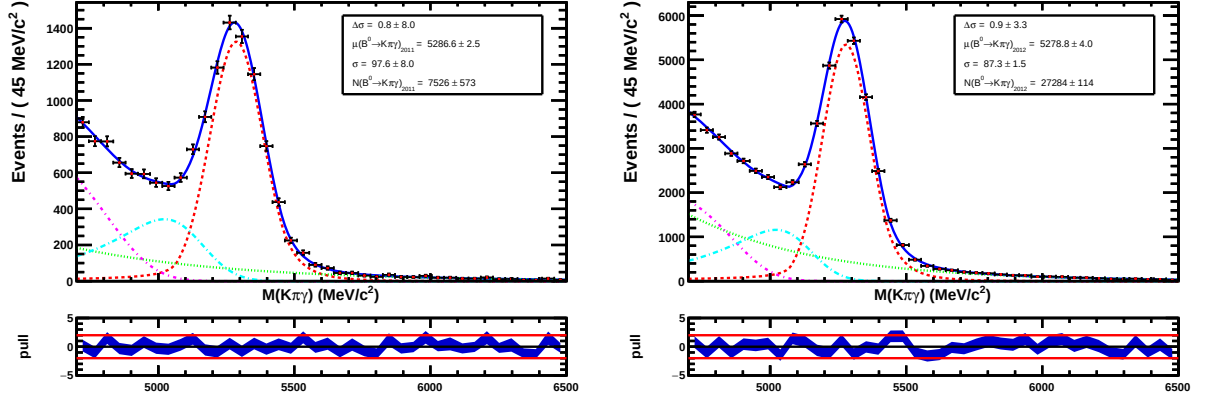
Figure 3.17: Final B^0 \rightarrow K^\pm \pi^\mp \gamma mass fits for 2011 and 2012 data.
