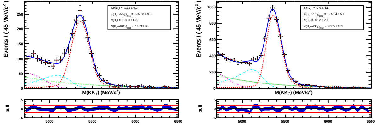
Figure 3.18: Final B_s \rightarrow K^+ K^- \gamma mass fits for 2011 and 2012 data.
