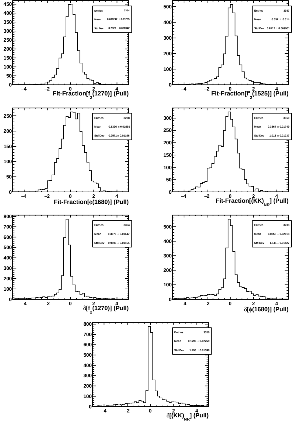
Figure 4.14: Pull distributions of the moduli and the phases of the complex amplitude coefficients c_R for the model components from 3.6 \times 10^3 toy experiments produced according to the \mathcal{B}_1 minimum.
