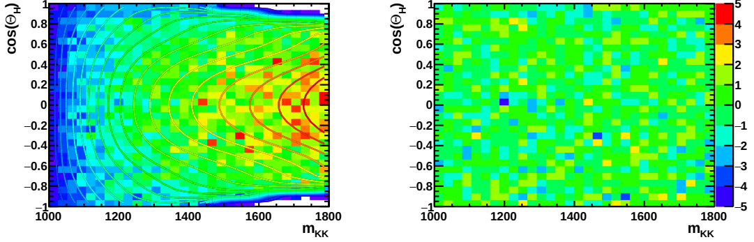
Figure 4.8: Acceptance function on top of the phase-space MC (left) and corresponding pulls (right).
