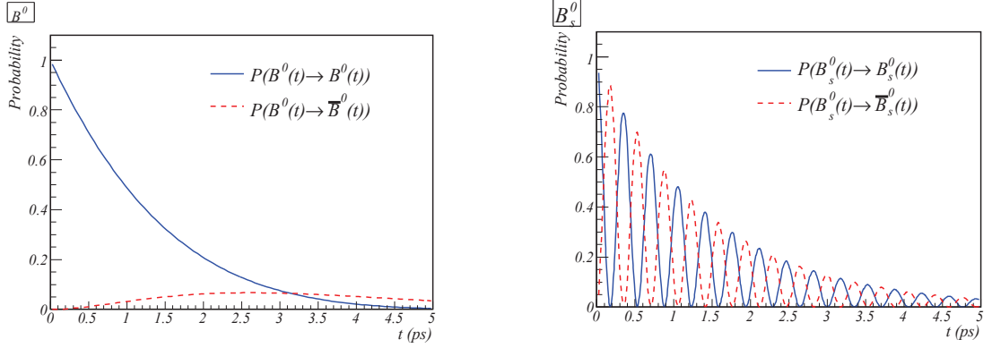
Figure 1.8: Time evolution of the B^0 - \bar{B}^0 (left) and B_s - \bar{B}_s^0 (right) systems.
