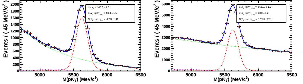
Figure 3.4: \Lambda_b \rightarrow p^\pm K^\mp \gamma mass fits for 2012 and 2016 data at the preselection level. The data distribution (black dots), signal (red line), combinatorial (green line), one-missing-pion part. reco. (light blue line) and inclusive part. reco. models (pink line) are displayed.
