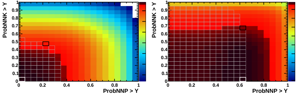
Figure 3.8: \Lambda_b \rightarrow p^\pm K^\mp \gamma FoM for 2012 (left) and 2016 (right).
