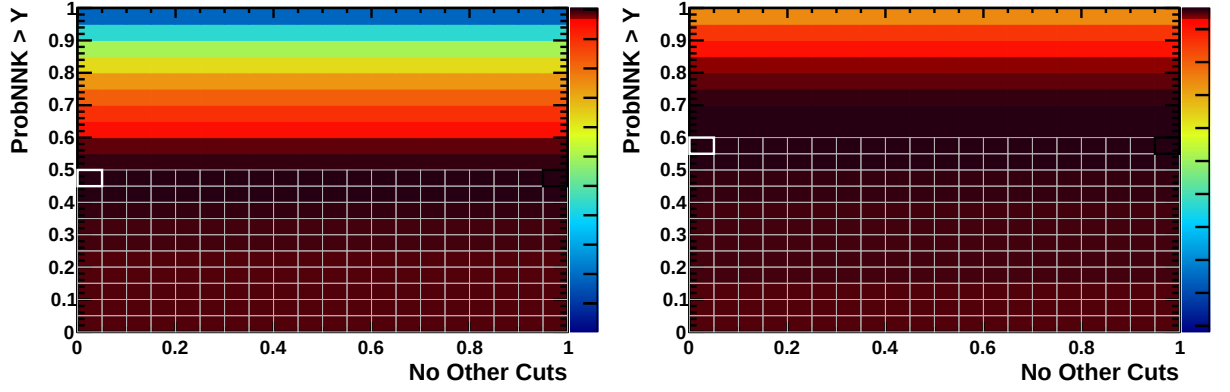
Figure 3.7: B_s \rightarrow K^+ K^- \gamma FoM for 2012 (left) and 2016 (right).
