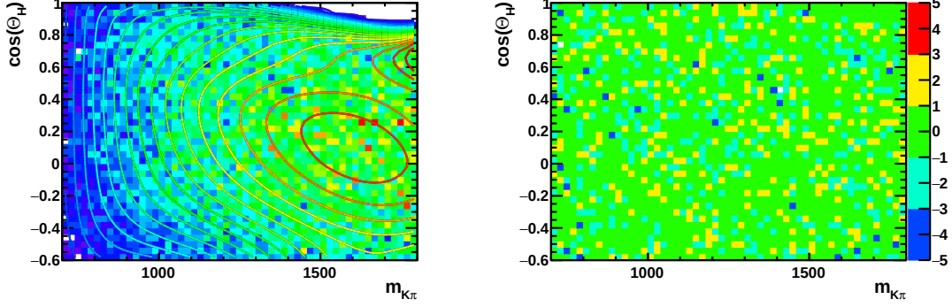
Figure 5.5: Acceptance function on top of the phase-space MC (left) and corresponding pulls (right).
