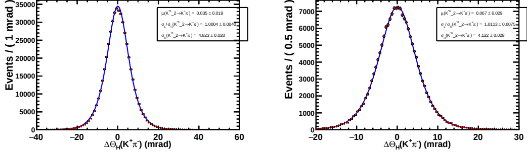
Figure 5.3: \Delta\theta = \theta_{K\pi}^{sim} - \theta_{K\pi}^{rec} distribution in the K^{*0} region (left) and K_2^{*0} region (right).
