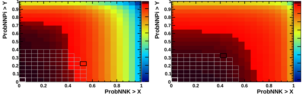
Figure 3.6: B^0 \rightarrow K^\pm \pi^\mp \gamma FoM for 2012 (left) and 2016 (right).
