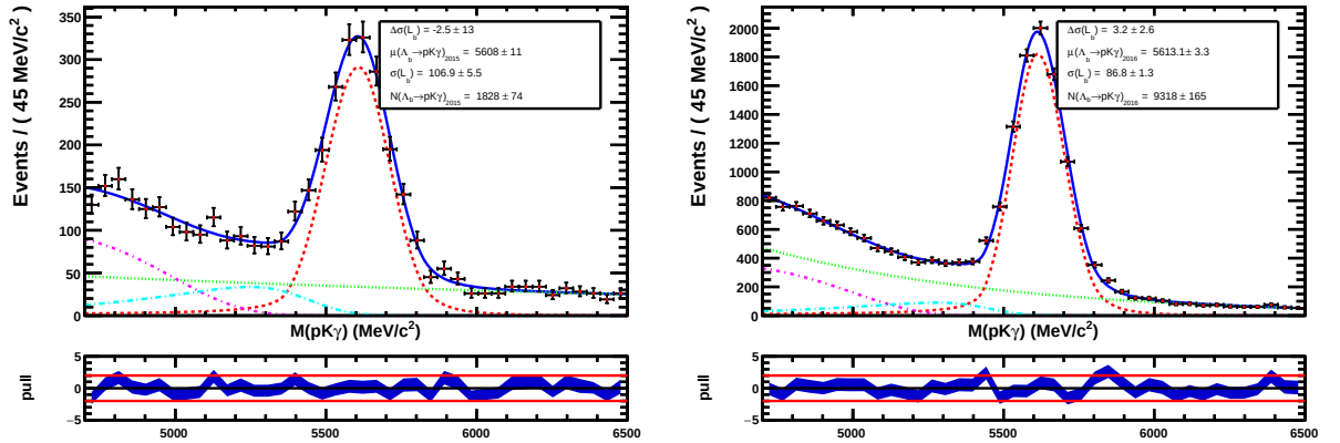
Figure 3.22: Final \Lambda_b \rightarrow p^\pm K^\mp \gamma mass fits for 2015 and 2016 data.
