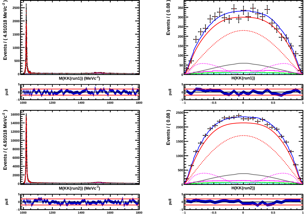
Figure 4.17: Projection of the simultaneous fit of Run 1 (top) and Run 2 (bottom) data on the m_{KK} observable (left) and \cos(\theta_{KK}) observable (right).
