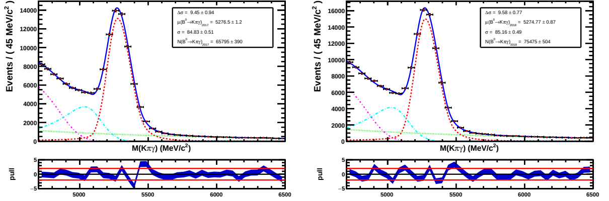
Figure 3.23: Final B^0 \rightarrow K^\pm \pi^\mp \gamma mass fits for 2017 and 2018 data.
