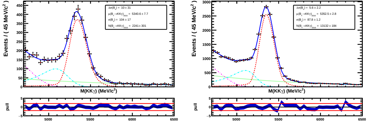
Figure 3.21: Final B_s \rightarrow K^+ K^- \gamma mass fits for 2015 and 2016 data.
