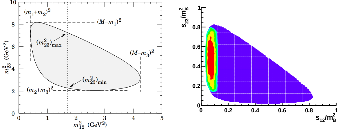
Figure 4.1: Kinematical boundaries of a typical Dalitz plot [88](left), and the actual phase space region of the selected data (right).
