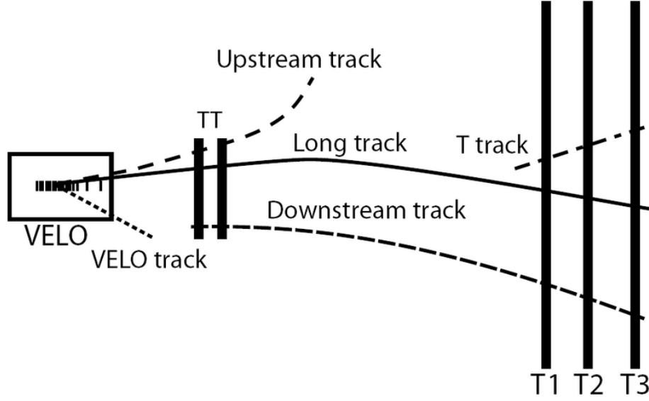
Figure 2.11: Illustration of the different track types: long, upstream, downstream, VELO and T tracks.
