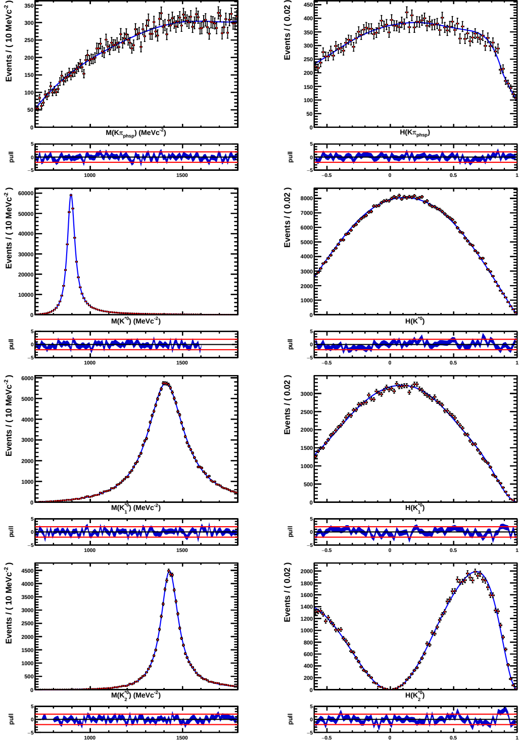
Figure 5.6: Projection of the simultaneous fit to MC data on the m_{K\pi} (left) and \cos(\theta_{K\pi}) (right) observables for the phase-space K\pi\gamma (top line), the two vector resonances K^{*0}(892)\gamma (second line) and K^{*0}(1410)\gamma (third line), and the tensor resonance K^{*0}(1430)_2\gamma (bottom line) sample < s .
