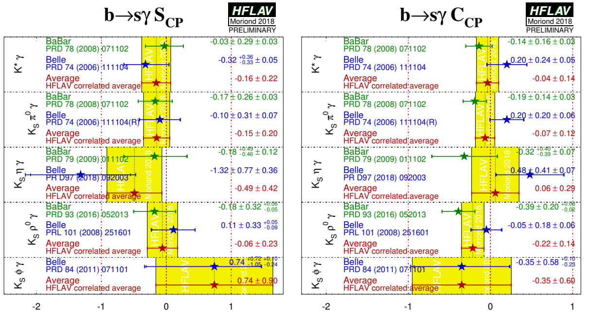
Figure 1.10: Experimental status on the measurements of S (left) and C (right) [18].
