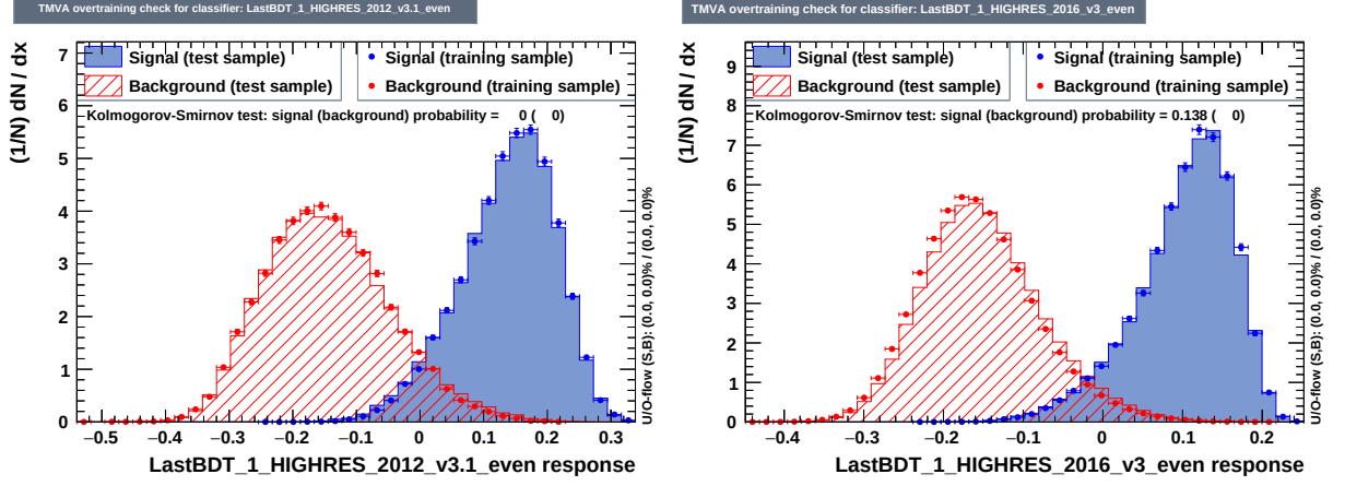
Figure 3.12: B^0 \rightarrow K^\pm \pi^\mp \gamma BDT outputs for 2012 and 2016 selection.
