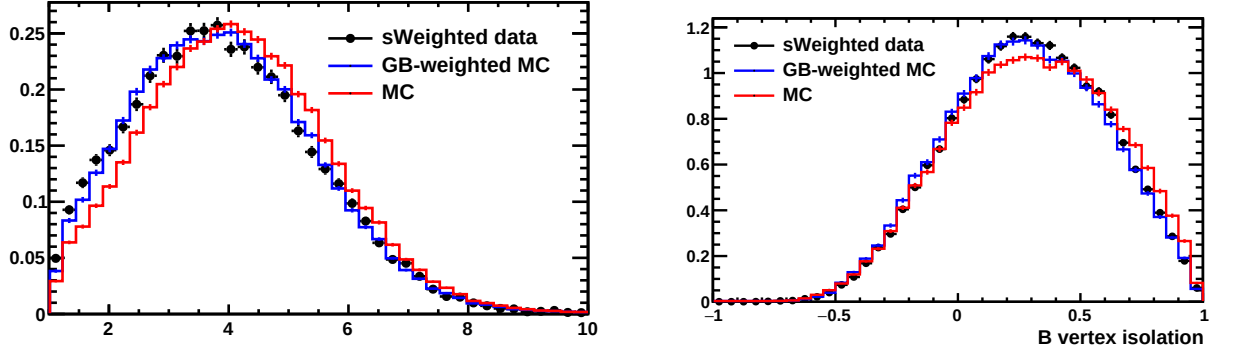
Figure 3.10: Results of the GB-weighting procedure on B^0 \rightarrow K^{*0} \gamma MC ( \log(\text{Smallest } \Delta \chi^2_{vtx}(B)) on the left, B vertex isolation on the right).
