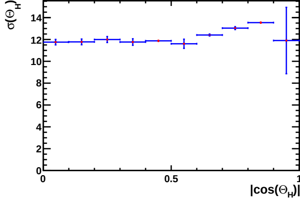
Figure 4.6: Resolution of the \Delta\theta = \theta_{\text{KK}}^{\text{sim}} - \theta_{\text{KK}}^{\text{rec}} distribution as a function of |\cos\theta_{\text{KK}}| in the \phi region.
