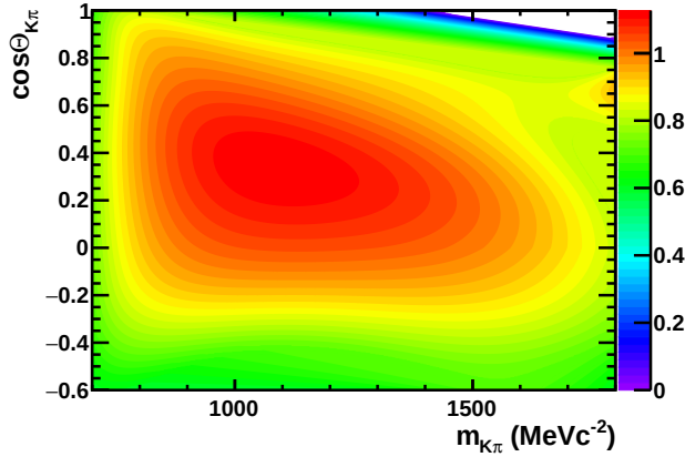
Figure 5.4: Selection acceptance in the (m_{K\pi}, \cos(\theta_{K\pi})) plane. The absolute normalisation is arbitrarily set near the K^{*0} pole: \varepsilon(896.5, 0) = 1 .
