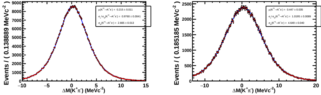
Figure 5.2: \Delta M = m_{K\pi}^{\text{sim}} - m_{K\pi}^{\text{rec}} distribution in the K^{*0} region (left) and K_2^{*0} region (right).
