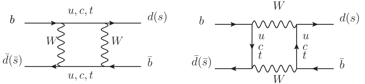
Figure 1.7: Box diagrams describing the B^0 - \bar{B}^0 and B_s^0 - \bar{B}_s^0 mixing.
