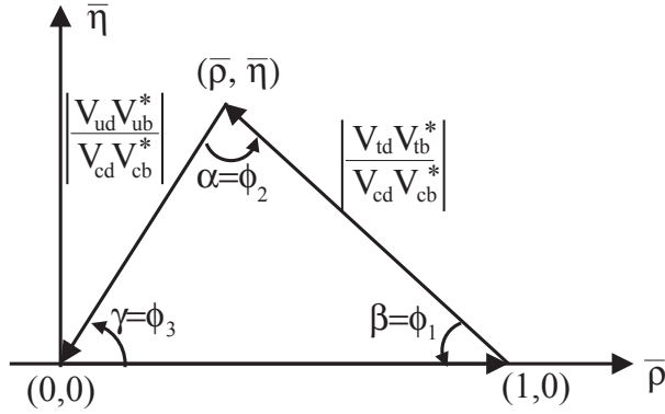
Figure 1.5: Graphical representation in the complex plane (\bar{\rho}, \bar{\eta}) of the unitarity triangle of Eq. 1.37 as normalized to V_{cd}V_{cb}^* : 1 + V_{ud}V_{ub}^*/V_{cd}V_{cb}^* + V_{td}V_{tb}^*/V_{cd}V_{cb}^* = 0 .
