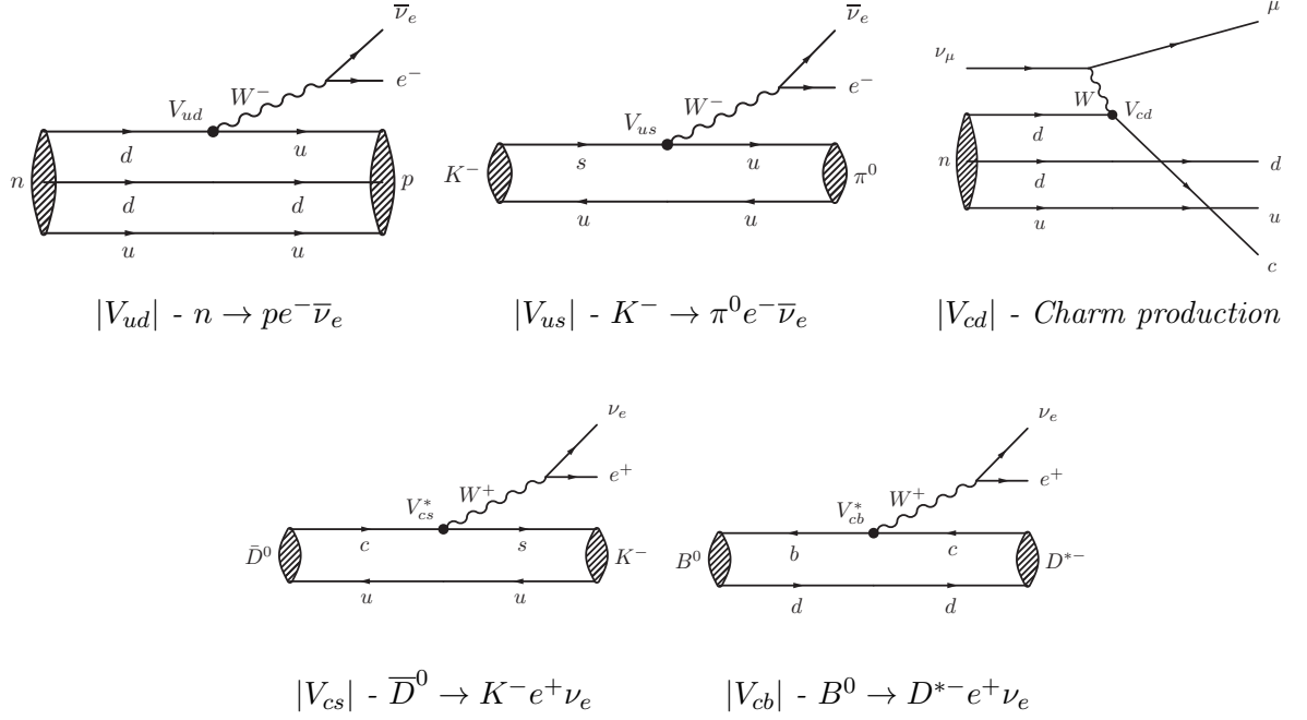
Figure 1.3: Feynman diagrams of some specific processes important for determining five of the |V_{ij}| matrix elements.
