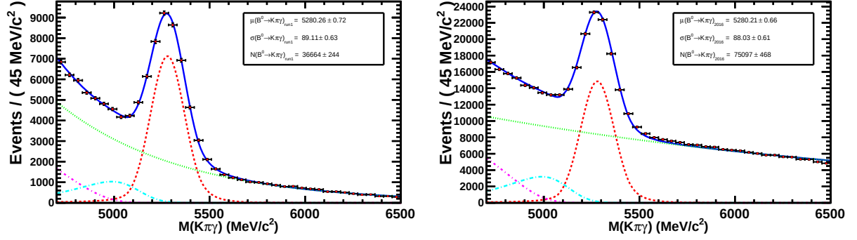
Figure 3.2: B^0 \rightarrow K^\pm \pi^\mp \gamma mass fits for 2012 and 2016 data at the preselection level. The data distribution (black dots), signal (red line), combinatorial (green line), one-missing-pion part. reco. (light blue line) and inclusive part. reco. models (pink line) are displayed.
