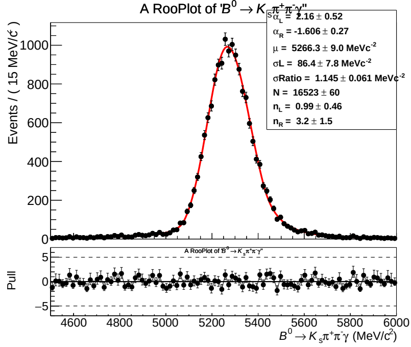
Figure A.3: Fit to the B mass distribution in the full B^0 \rightarrow K_S^0 \pi^+ \pi^- \gamma MC available.
