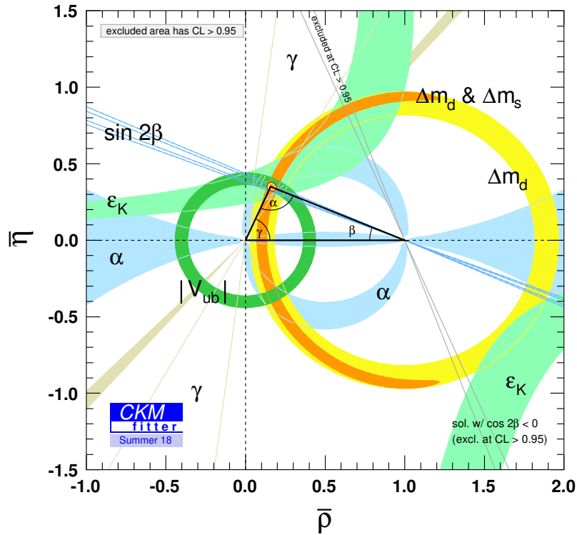
Figure 1.6: Constraints on the unitarity triangle at a 95% confidence level [15].
