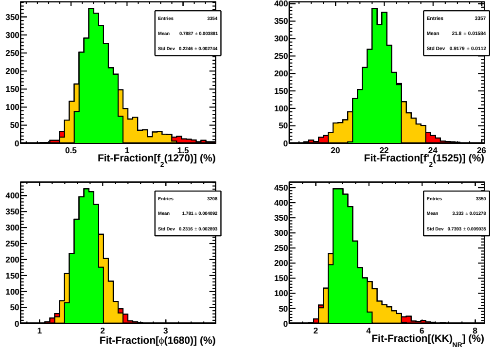
Figure 4.15: Distributions of the relative Fit-Fraction normalized to \phi(1020) , for f_2(1270) (top left), f_2'(1525) (top right), \phi(1680) (bottom left) and Non-Resonant (KK) NR (bottom right) from 3.6 \times 10^3 toy experiments produced according to the \mathcal{B}_1 minimum. The one, two and three \sigma asymmetric intervals, containing 68.27%, 95.45% and 99.73% of the toy population, respectively, are indicated.
