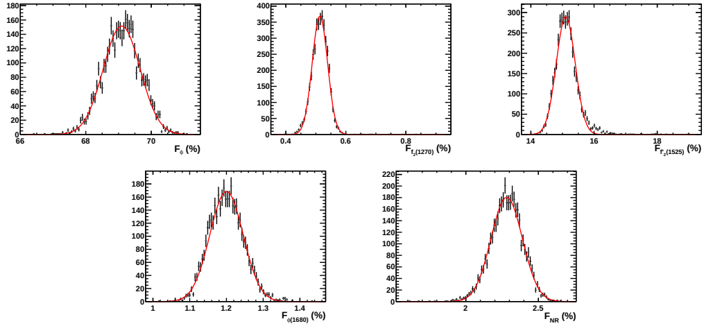
Figure 4.16: Distribution of the amplitude Fit-Fractions when the acceptance parameters are varied within their statistical uncertainty ( 3.6 \times 10^3 fits).
