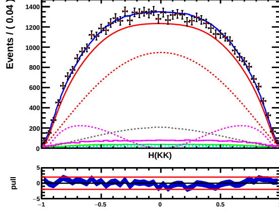
Figure 4.18: Projection on \cos(\theta_{KK}) of the fit with B_s/\bar{B}_s asymmetry allowed.
