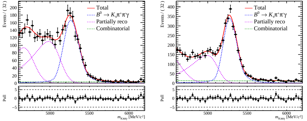
Figure A.4: Preliminary fit to the full (Run 1/Run2), data for B^0 \rightarrow K_S^0 \pi^+ \pi^- \gamma , with DD K_s^0 (left) and LL K_s^0 (right).
