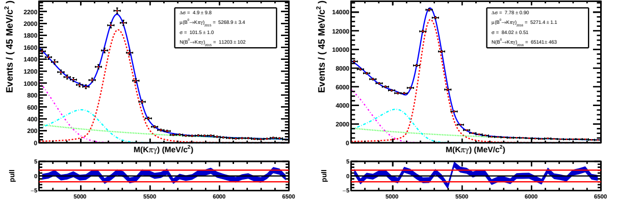
Figure 3.20: Final B^0 \rightarrow K^\pm \pi^\mp \gamma mass fits for 2015 and 2016 data.
