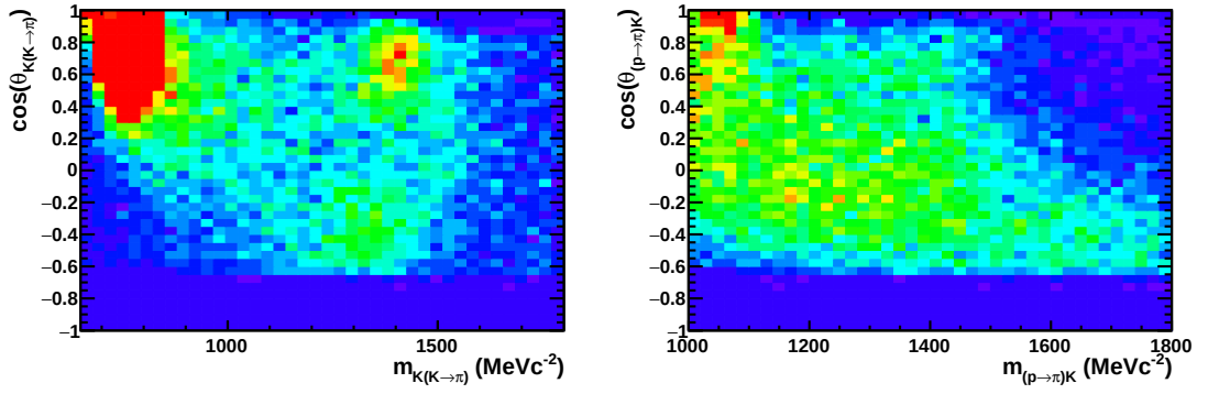
Figure 5.7: Projection in the (m_{K\pi}, \cos(\theta_{K\pi})) plane for the reconstructed and s Weighted B_s \rightarrow KK\gamma candidates (left) and \Lambda_b \rightarrow pK\gamma (right). The di-hadron mass and helicity are computed assigning a kaon (pion) mass to the pion (proton) candidate.
