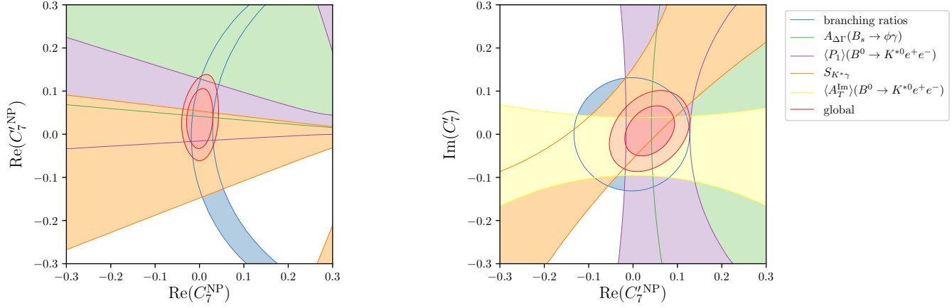
Figure 1.11: Constraints on NP contributions to the Wilson coefficients C_7 and C_7' . For the global constraints (in red), 1 and 2 \sigma contours are shown, while the individual constraints are shown at the 1 \sigma level. The SM expectation is (0,0).
