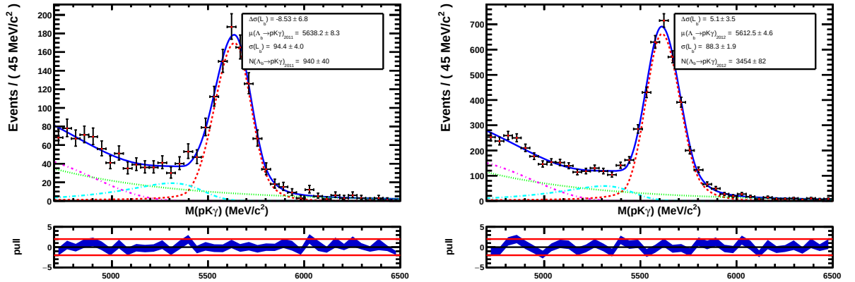
Figure 3.19: Final \Lambda_b \rightarrow p^\pm K^\mp \gamma mass fits for 2011 and 2012 data.
