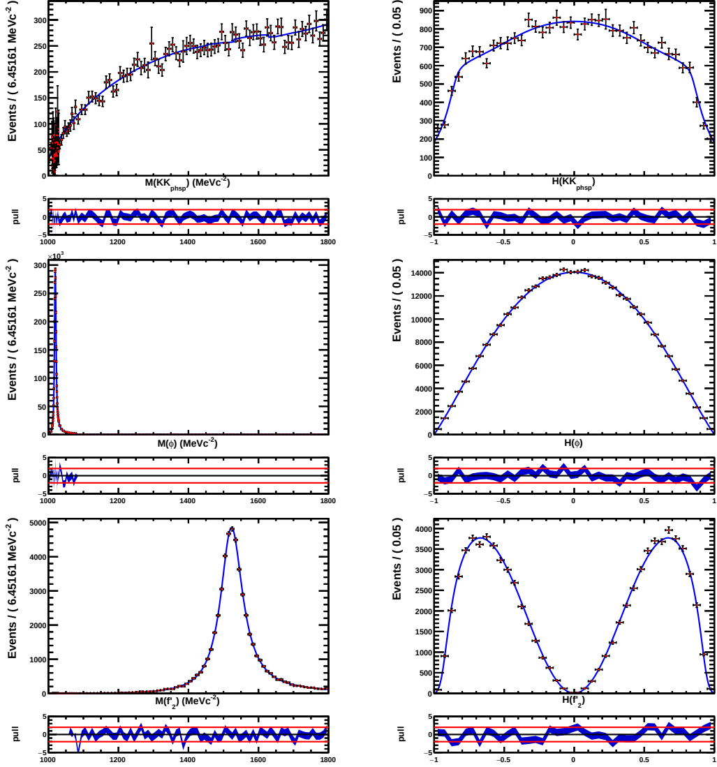
Figure 4.9: Projection of the simultaneous fit to MC data on the m_{KK} (left) and \cos(\theta_{KK}) (right) observables for the phase-space KK\gamma (top line), \phi(1020)\gamma (middle line), f'_2(1525)\gamma (bottom line) samples. An adaptative binning is applied on the m_{KK} observable, with a fine granularity in the region of the narrow \phi(1020) .
