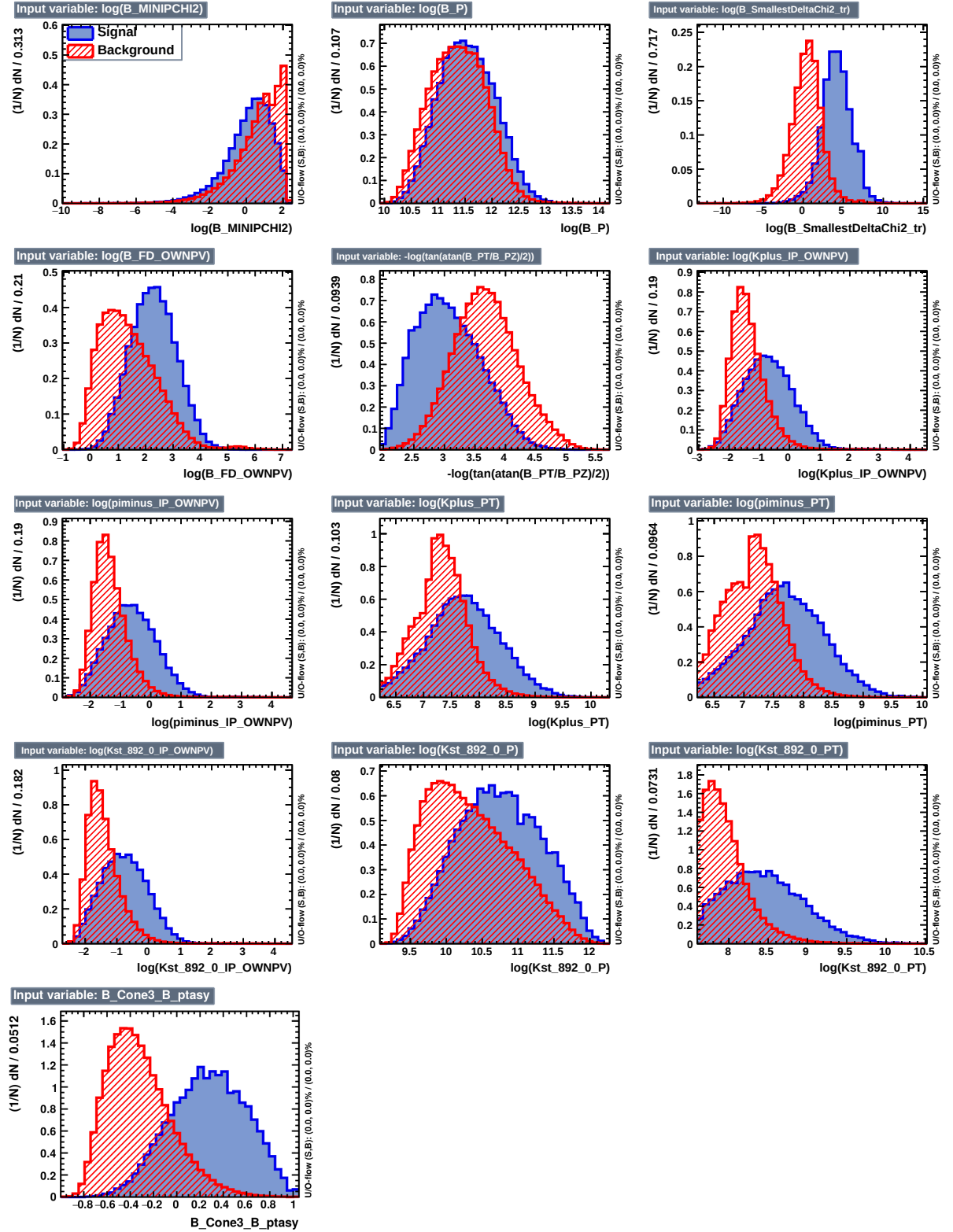
Figure 3.11: Training variables distributions for the B^0 \rightarrow K^\pm \pi^\mp \gamma 2016 MVA selection, with signal MC in blue and data side band in red.
