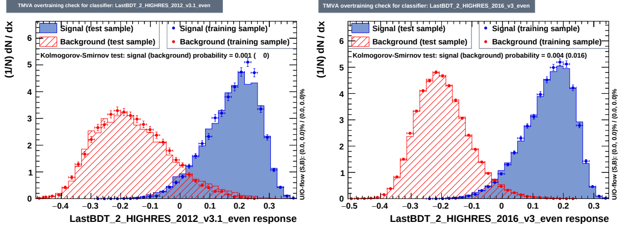
Figure 3.13: B_s \rightarrow K^+ K^- \gamma BDT outputs for 2012 and 2016 selections.
