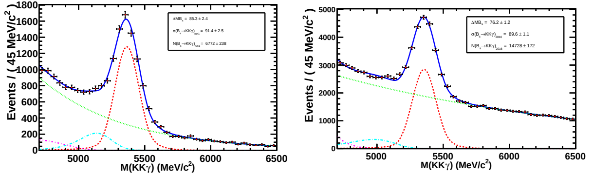
Figure 3.3: B_s \rightarrow K^+ K^- \gamma mass fits for 2012 and 2016 data at the preselection level. The data distribution (black dots), signal (red line), combinatorial (green line), one-missing-pion part. reco. (light blue line) and inclusive part. reco. models (pink line) are displayed.
