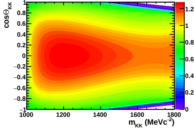
Figure 4.7: Selection acceptance in the (m_{\text{KK}}, \cos(\theta_{\text{KK}})) plane. The absolute normalisation is arbitrarily set near the \phi(1020) pole: \varepsilon(1019.5, 0) = 1 .
