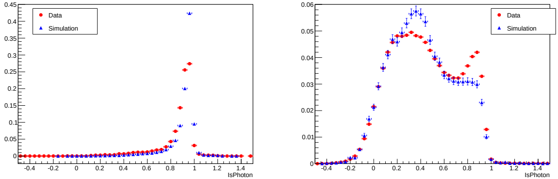
Figure 2.23: Data/MC comparison of the IsPhoton distributions for B^0 \rightarrow K^{*0} \gamma (left) and D^0 \rightarrow K^- \pi^+ \pi^0 (right) channels, in the Run 1 data. Red dots stand for background subtracted data while blue triangles are for MC events.
