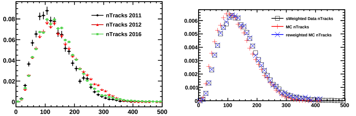
Figure 3.5: Track multiplicity distributions in 2011, 2012 and 2016 (left) and 2016 reweighting (right).
