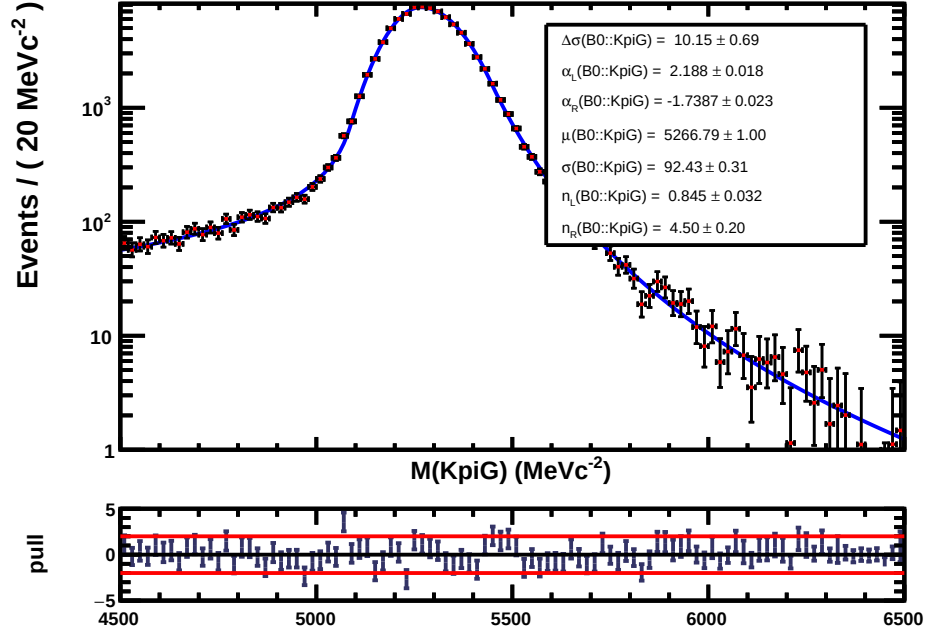
Figure 3.14: Fit to the reconstructed B mass in B^0 \rightarrow K^{*0} \gamma MC 2012 (log scale).
