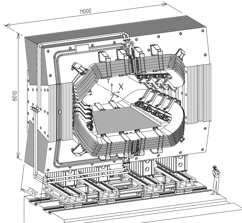
Figure 2.10: Sketch of the dipole magnet of LHCb.
