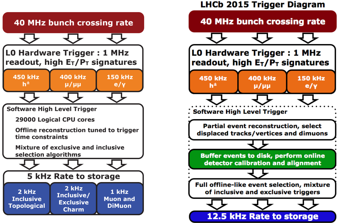
Figure 2.24: Flow-diagram of the different trigger stages in Run 1 (left) and Run 2 (right). Software High Level Trigger indicates HLT1 and HLT2 stages.
