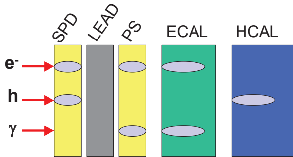
Figure 2.15: Energy deposited in the different parts of the calorimeter by an electron ( e ), a hadron ( h ) and a photon ( \gamma ).
