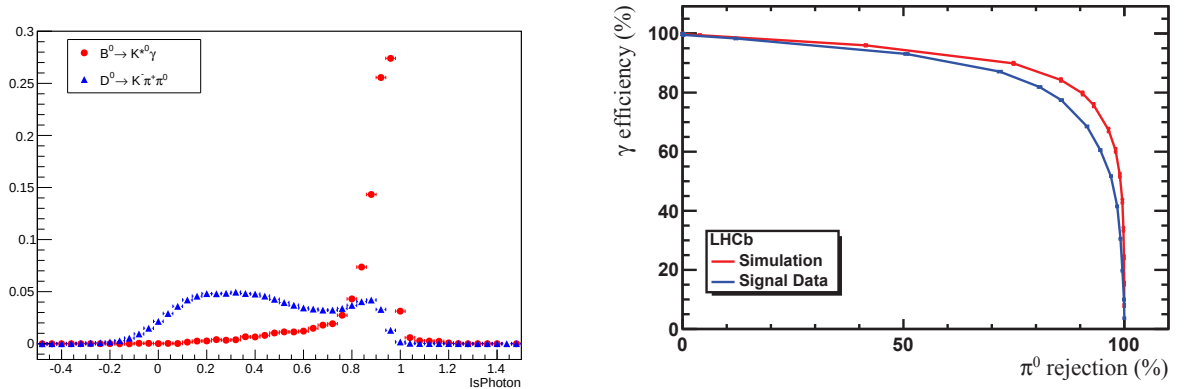
Figure 2.22: IsPhoton distributions (left) for B^0 \rightarrow K^{*0} \gamma (red dots) and D^0 \rightarrow K^- \pi^+ \pi^0 (blue triangles) background subtracted data. Photon identification efficiency as a function of \pi^0 rejection efficiency [62] (right) for the \gamma/\pi^0 separation tool for simulation (red curve) and data (blue curve).
