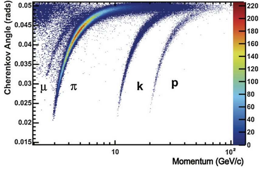
Figure 2.14: Reconstructed Cherenkov angle as a function of track momentum in the C_4F_{10} radiator [47].
