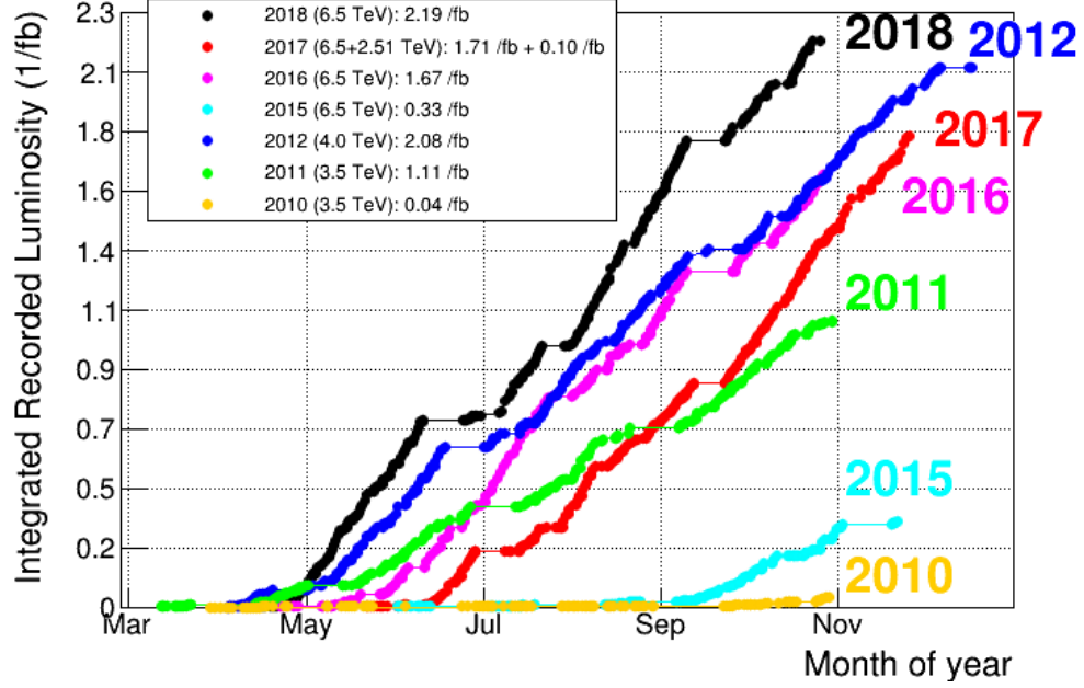
Figure 2.3: Integrated luminosities recorded by the LHCb experiment during Run 1 (2010-2012) and Run 2 (2015-2018) data taking periods, for p-p collisions. Corresponding beam energies are also displayed.
