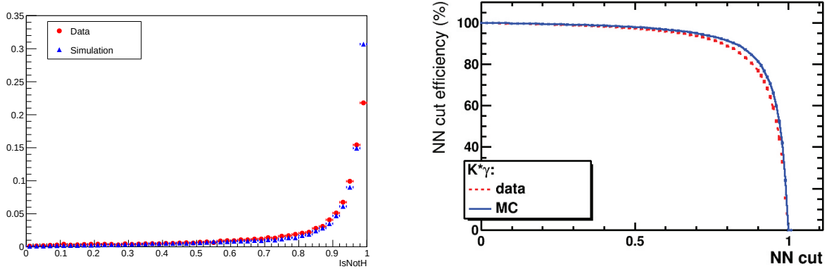
Figure 2.21: IsNotH distributions (left) and corresponding efficiencies [64] (right) for B^0 \rightarrow K^{*0}\gamma data (red dots/dashed line) and MC (blue triangles/solid line). Data points are background subtracted.
