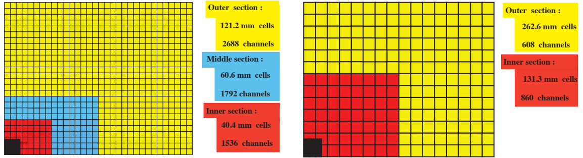
Figure 2.16: Left: frontal view of the SPD/PS and ECAL detectors where the three regions mentioned in the text are shown. Right: frontal view of the HCAL where there are only two regions.
