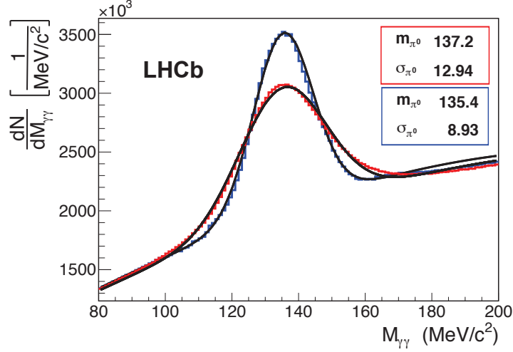
Figure 2.20: Invariant mass distribution for \pi^0 \rightarrow \gamma\gamma candidates before (red curve) and after (blue curve) applying the fine ECAL calibration procedure. Values in the red (blue) box are the mean and sigma of the signal peak distribution in \text{MeV}/c^2 before (after) applying the calibration.
