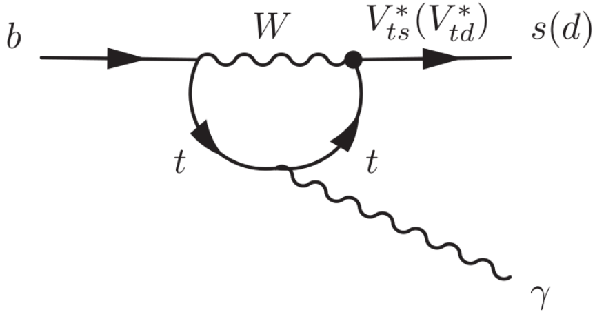
Figure 3.1: Feynman diagram for b \rightarrow s(d) \gamma transitions.
