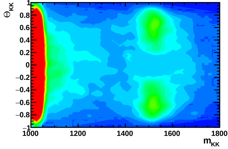
Figure 4.3: B_s \rightarrow K^+ K^- \gamma weighted candidates in the modified Dalitz plane ( m_{KK}, \cos(\theta_{KK}) ).
