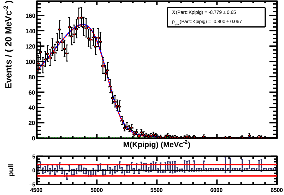
Figure 3.15: Fit to the B mass in B^+ \rightarrow K^{*0} \pi^+ \gamma MC 2012, reconstructed in the B^0 \rightarrow K^\pm \pi^\mp \gamma hypothesis.
