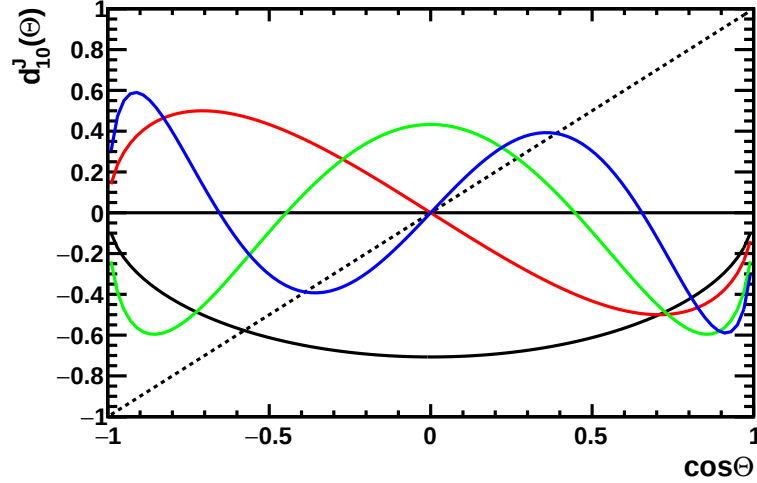
Figure 4.2: Wigner d-functions d_{10}^J(\theta) that describe the angular dependency in the B \rightarrow R_J \gamma decay amplitude, as a function of \cos(\theta) for J=1 (black curve), J=2 (red), J=3 (green) and J=4 (blue). The diagonal dashed line represents the d_{00}^1(\theta) = \cos(\theta) function, that appears in the Scalar to Vector-Scalar decays, S \rightarrow VS , e.g. B^0 \rightarrow K^{*0} \pi^0 .
