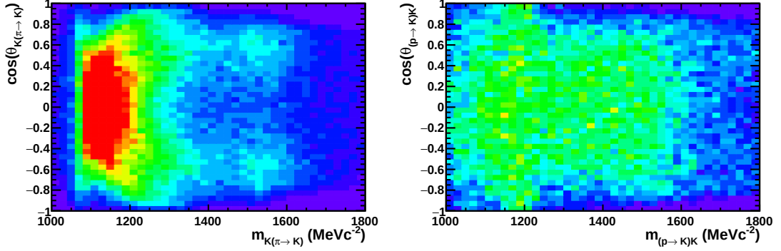
Figure 4.10: Projection in the (m_{\text{KK}}, \cos(\theta_{\text{KK}})) plane for the reconstructed and s Weighted B^0 \rightarrow K\pi\gamma candidates (left) and \Lambda_b \rightarrow pK\gamma (right). The di-hadron mass and helicity are computed assigning a kaon mass to the pion (proton) candidate.
