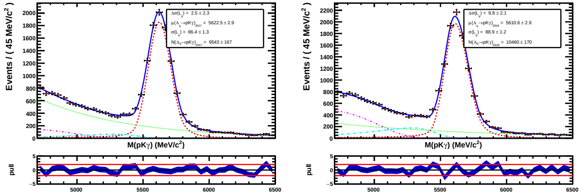
Figure 3.25: Final \Lambda_b \rightarrow p^\pm K^\mp \gamma mass fits for 2017 and 2018 data.
