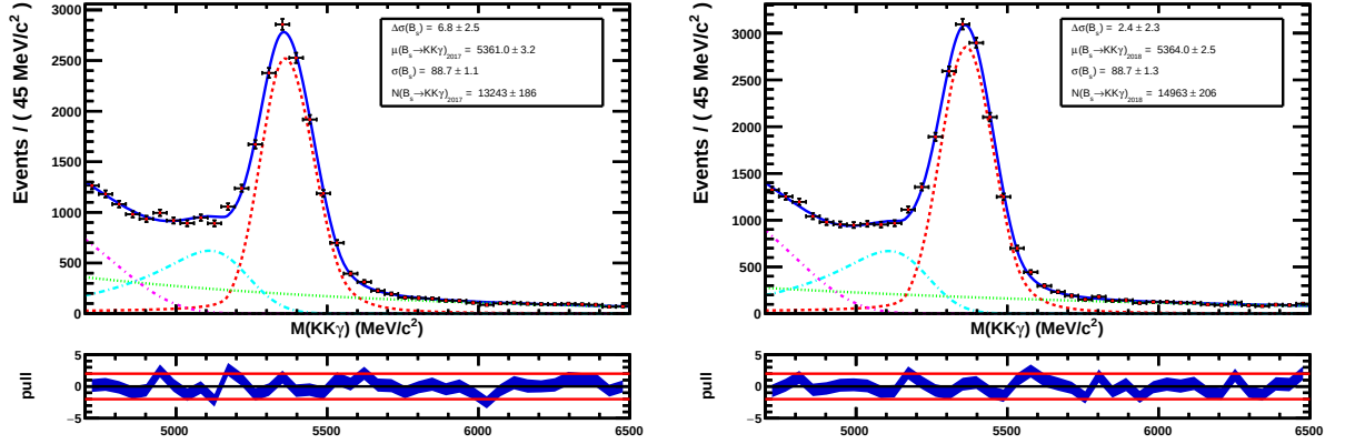
Figure 3.24: Final B_s \rightarrow K^+ K^- \gamma mass fits for 2017 and 2018 data.
