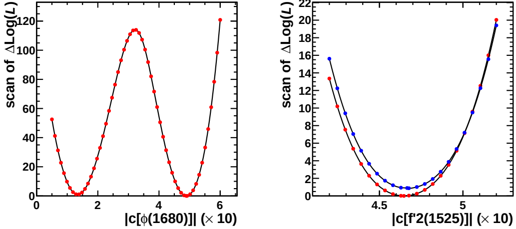
Figure 4.11: Left: log-Likelihood scan of the |c_{\phi(1680)}| parameter. The best-fit minimum, \mathcal{B}_0 , is found near |c_{\phi(1680)}| \times 10 \sim 5 . The second minimum, \mathcal{B}_1 , ( \Delta\mathcal{LL} = +0.78 ), is found at |c_{\phi(1680)}| \times 10 \sim 1.2 . Right: log-Likelihood scans of the |c_{f'_2(1525)}| parameters performed in the vicinity of \mathcal{B}_1 (red points) and \mathcal{B}_0 (blue points). The minimum of both scans is located around the same value |c_{f'_2(1525)}| \times 10 \sim 4.6 . Similar behaviour is observed when projecting the log-Likelihood on the other fit parameters.
