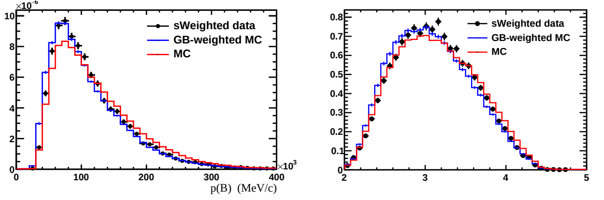
Figure 3.9: Results of the GB-weighting procedure on B^0 \rightarrow K^{*0} \gamma MC ( p(B) left, \eta(B) right).
