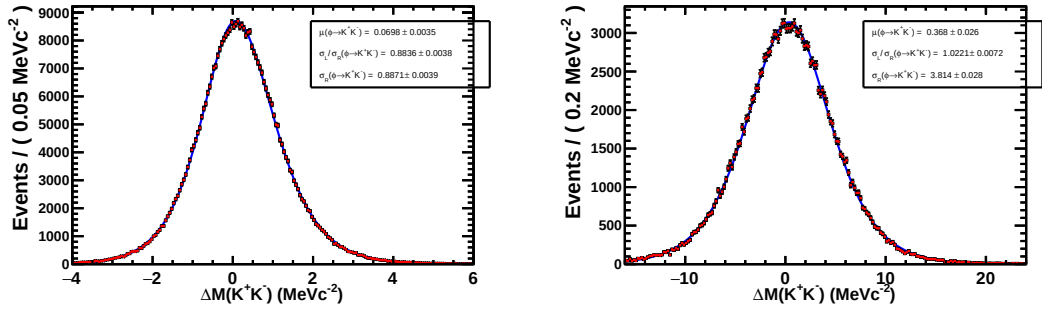
Figure 4.4: \Delta M = m_{KK}^{sim} - m_{KK}^{rec} distribution in the \phi (left) and f'2 (right) region.
