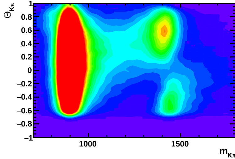
Figure 5.1: s Weighted distribution for K\pi candidates in the (m_{K\pi}, \cos(\theta_{K\pi})) plane.
