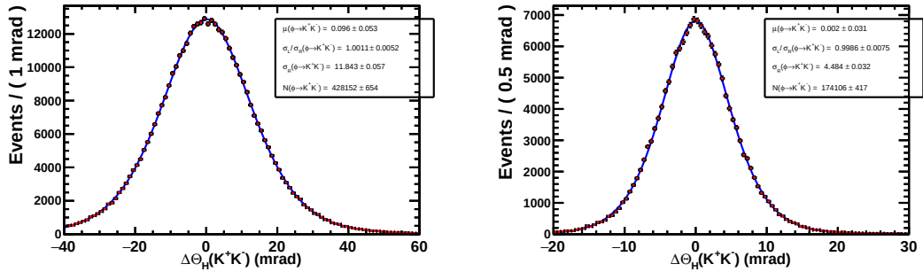
Figure 4.5: \Delta\theta = \theta_{KK}^{sim} - \theta_{KK}^{rec} distribution in the \phi(1020) (left) and f'_2(1525) (right) region.
