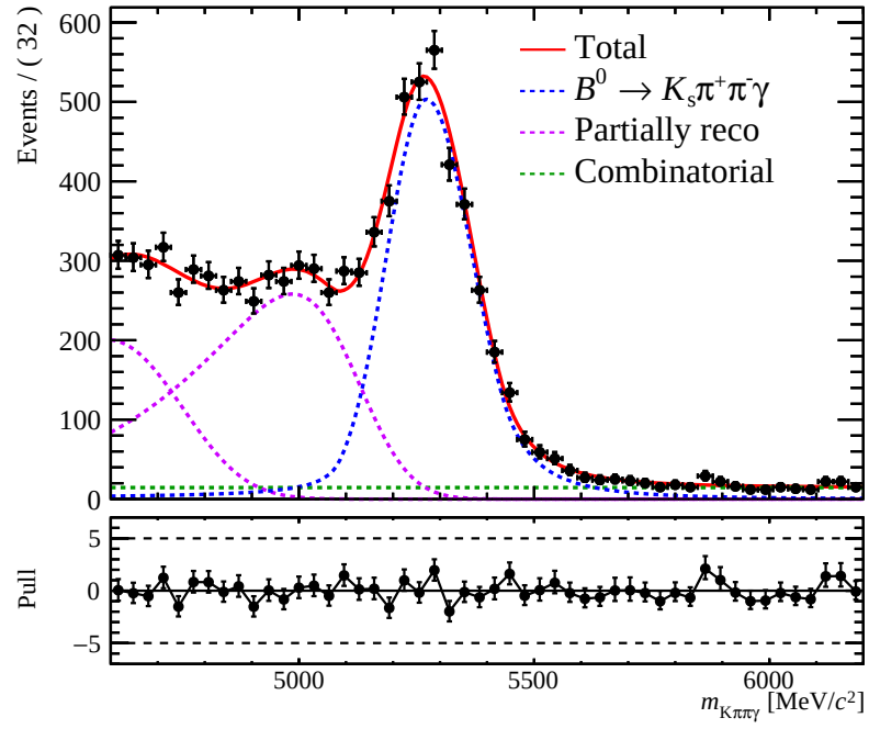
Figure A.5: Preliminary fit to the full (Run 1/Run 2, DD/LL) data for B^0 \rightarrow K_S^0 \pi^+ \pi^- \gamma .
