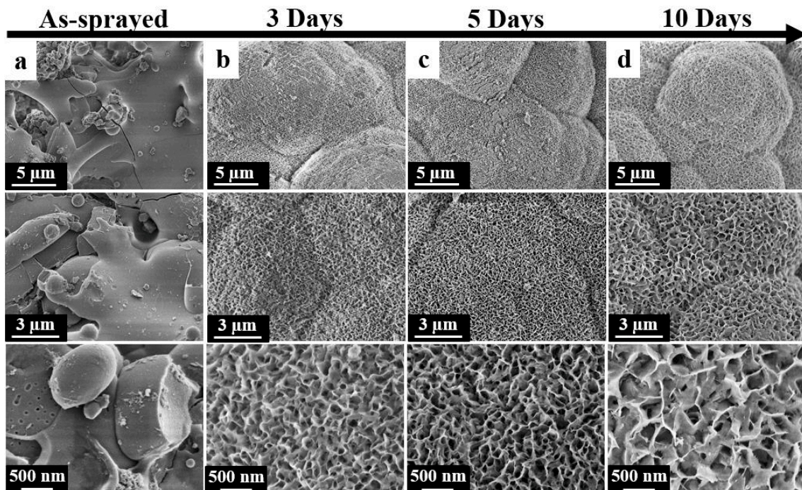
Figure 28. Apatite formation on the BHAp APS coating surface monitored by SEM after immersion in SBF at a) 0, b) 3, c) 5 and d) 10 days. Each surface is shown at three magnifications: 5000 x , 10000 x , and 35000 x .
