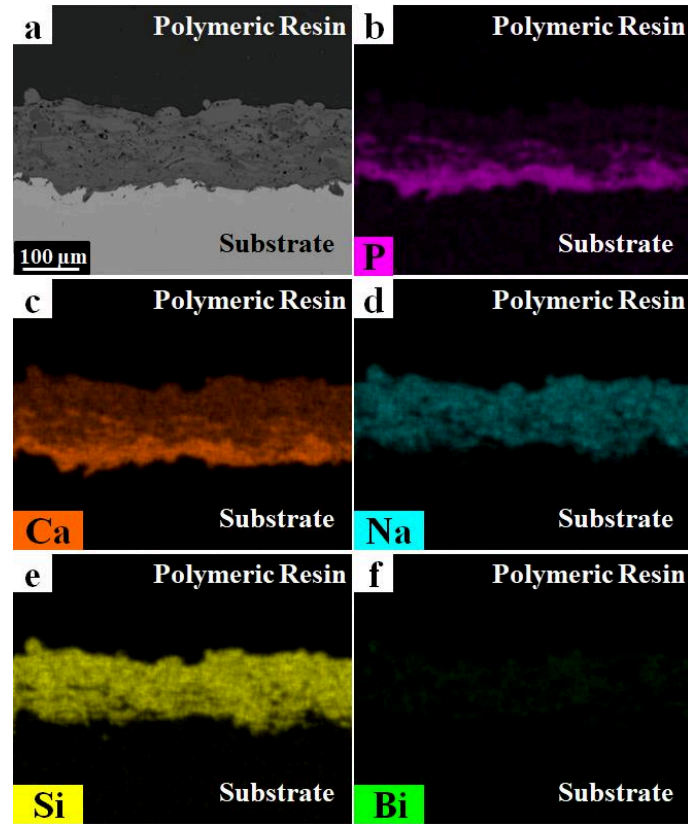
Figure 44. EDS Map analysis of graded BHAp/BG45SS+10Bi 2 O 3 APS coating cross-section: a) Secondary electron micrograph, b) Phosphorus, c) Calcium, d) Sodium, e) Silicon and f) Bismuth.
