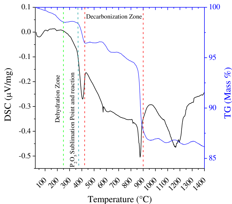
Figure 10. Thermal analysis of oxides and carbonate mixture by DSC during the glass melting.
