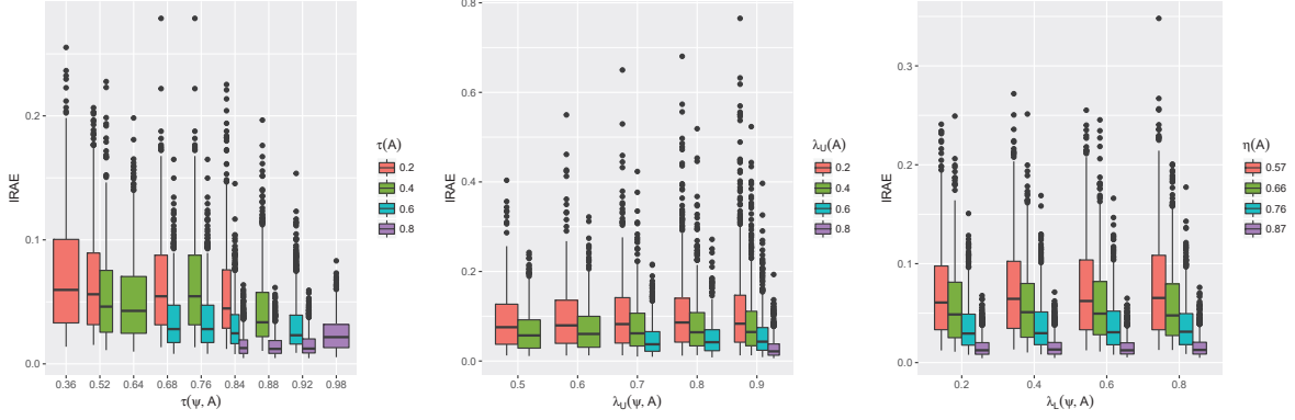
Figure 4.6: Boxplots of IRAE of A_{n,c}^{\text{CFG}} when n = 200 , d = 10 and the Pickands dependence function is LG for all panels. The Archimedean generators are Frank (left), Joe (middle) and Clayton (right). In the right panel, \eta_L(A) = 1/\{2A(1/2)\} = 2^{-1/\rho} is the lower tail dependence index of Ledford and Tawn (1996) .
