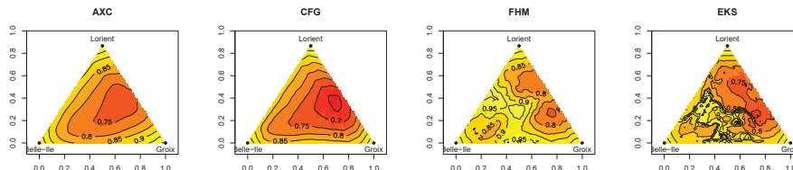
Figure 7.3: AXG: CFG-type estimator \hat{A}_{n,c}^{\text{CFG}} based on monthly maxima and the Clayton-Archimax model. CFG: Rank-based CFG estimator of Gudendorf and Segers (2011) based on seasonal maxima. FHM and EKS: Estimators of Fougères et al. (2015) and Einmahl et al. (2017) based on monthly maxima.
