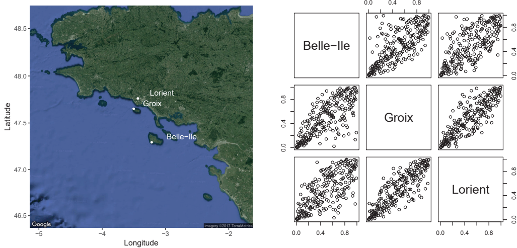
Figure 7.1: Satellite map of French Brittany, showing the sites Belle-Ile, Groix, and Lorient (left). Rankplots of monthly maximum precipitation for the months of September to February, from 1976 to 2016 (right).
