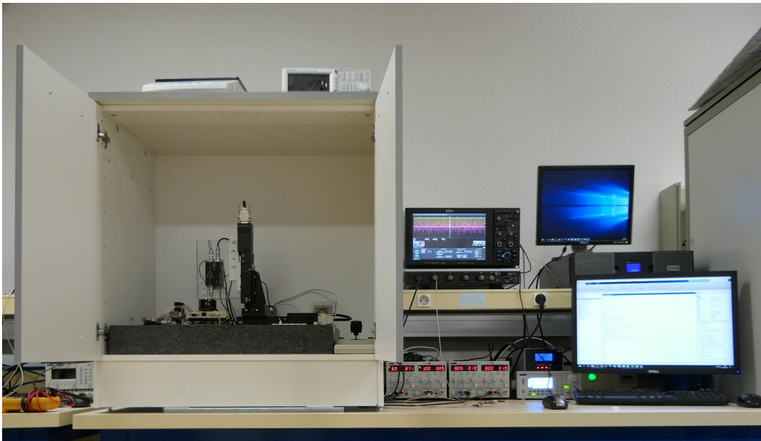
FIGURE 3.4: IR acquisition platform in its isolation container.
