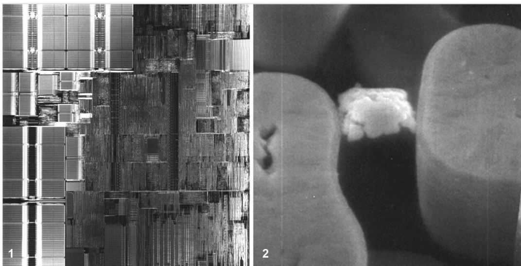
FIGURE 4.7: Investigation of a faulty micro-controller. 1. topological image of the IC measuring 196 \text{mm}^2 . 2. 0.2 \mu\text{m} \times 0.4 \mu\text{m} nickel particle contamination causing a short between two electrical nodes [SA95]
