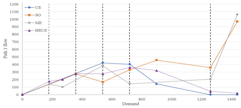
(a) Path 1 flow-demand diagram.
