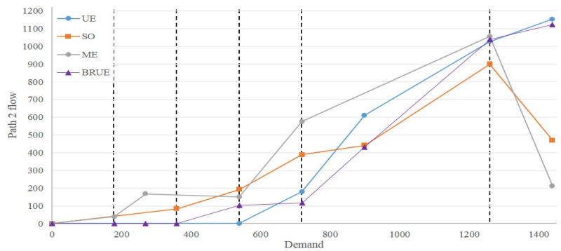
(b) Path 2 flow-demand diagram.
