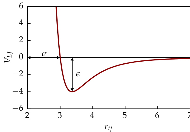
FIGURE 2.3: Example of the Lennard-Jones potential. All values are in arbitrary units.
