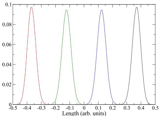
FIG. 10. Four localized orbitals having the largest occupation numbers for the case N = 4 . Pairs of corresponding orbitals having g and u symmetries have been combined in order to obtain completely localized combinations.
