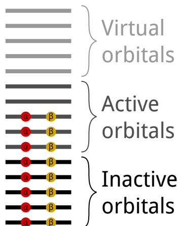
FIGURE 2.1: The CASSCF orbital spaces.
