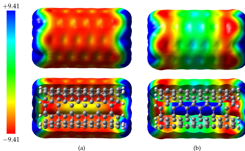
FIGURE 4.8: Molecular electrostatic potential of the unperturbed (5,5) CNT (a) and perturbed (b) by the presence of the azide ion. The isosurface value was set to 0.02. The energy scale is given in kcal/mol.
