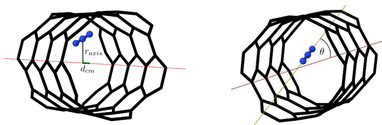
FIGURE A.2: Central starting geometry.
