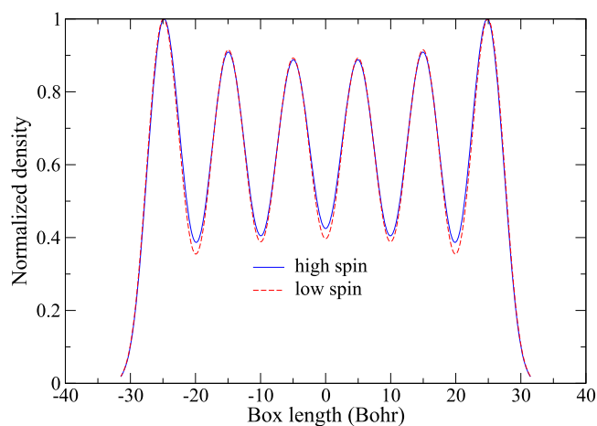
FIG. 5. The electron density for d = 10.0 Bohr.
