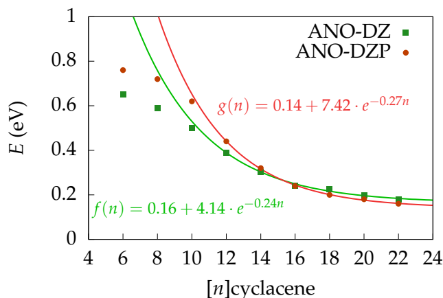
FIGURE 3.15: CASSCF( k, k ) singlet–triplet energy gaps calculated with the ANO-DZ (green squares) and the ANO-DZP (red circles) basis sets as a function of n .
