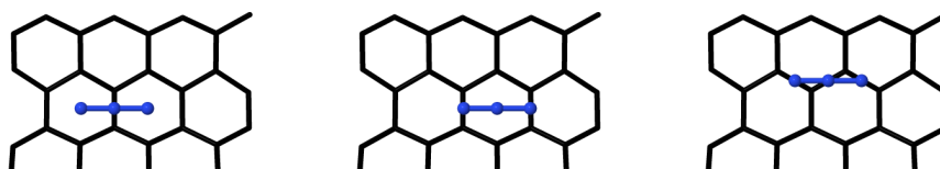
FIGURE A.1: Bond (left), hollow (center) and zigzag (right) starting sites.
