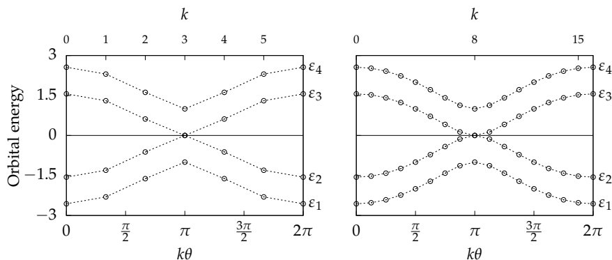
FIGURE 3.12: Hückel energy bands in t units for a [6]cyclacene (left) and for a [16]cyclacene (right). Note that the points at k\theta = 2\pi are the same as those at k\theta = 0 because of periodic boundary conditions.
