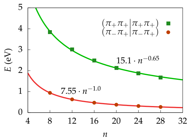
FIGURE 3.10: Two-electron integrals as a function of the system size n .
