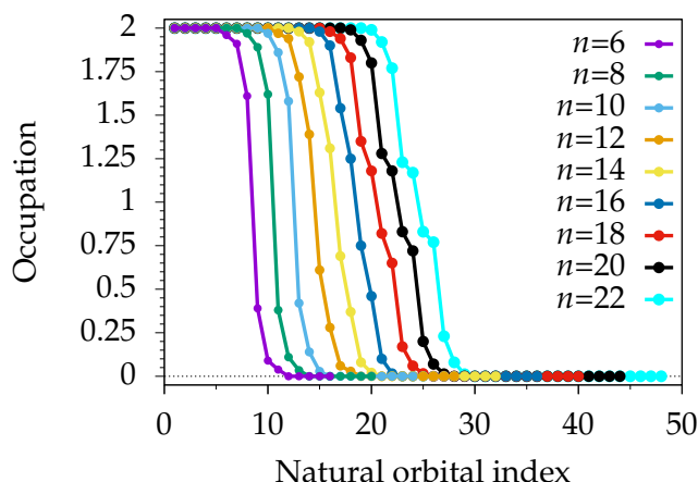
FIGURE 3.16: CASSCF NOONs. Note that all unique \pi orbitals are plotted, including those not included in the ASs.
