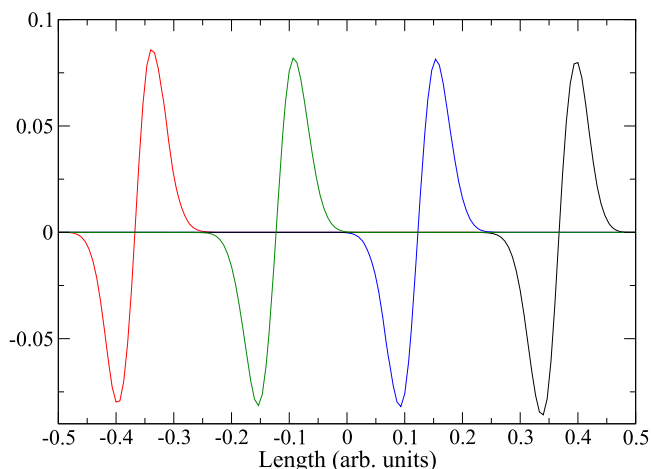
FIG. 11. Four localized orbitals having the 5th to 8th largest occupation numbers for the case N = 4 . Pairs of corresponding orbitals having g and u symmetries have been combined in order to obtain completely localized combinations.
