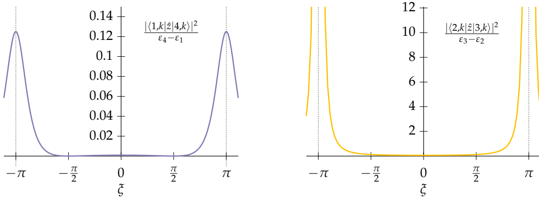
FIGURE 3.6: 1 \rightarrow 4 (left) and 2 \rightarrow 3 (right) contribution to \alpha_{zz} in \frac{b^2}{t} units.
