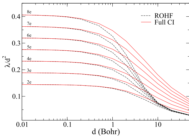
FIG. 7. The scaled HS localization tensor \lambda/d^2 as a function of the mean distance d (please note the logarithmic scale).
