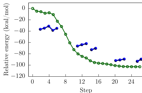
FIGURE 4.18: Relative energies with respect to step zero during the relaxation process. Geometries at steps 7, 11 and 26 are depicted along the curve without the surrounding nanotube for better representation.
