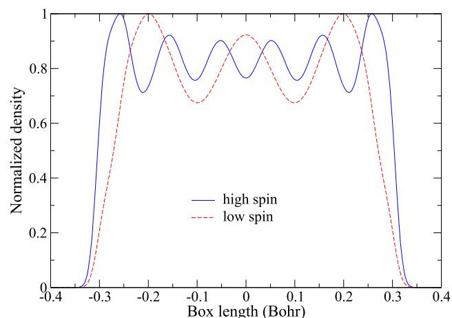
FIG. 3. The electron density for d = 0.1 Bohr.
