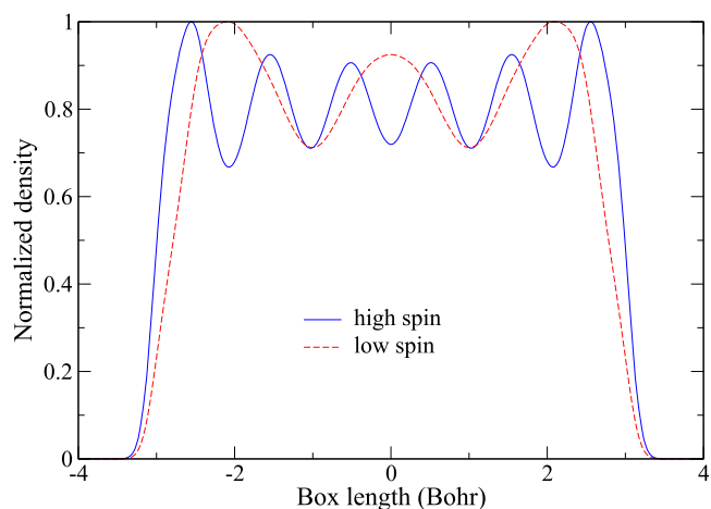
FIG. 4. The electron density for d = 1.0 Bohr.
