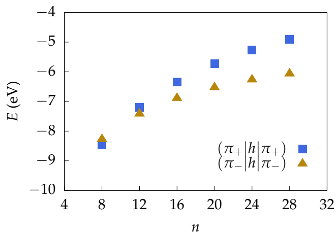
FIGURE 3.11: One-electron integrals as a function of the system size n .
