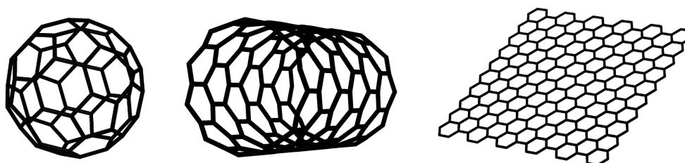
FIGURE 1.1: A C_{60} fullerene (left), a carbon nanotube (center) and graphene (right).
