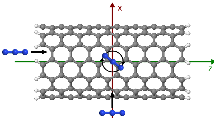
FIGURE 4.12: Scheme showing the three different ways in which the azide was moved to generate the energy profiles.
