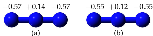
FIGURE 4.7: Partial atomic charges of the isolated (a) \text{N}_3^- fragment and confined (b) inside a CNT(5,5).
