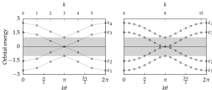
FIGURE 3.14: Hückel energy bands in t units for a [6]cyclohexene (left) and for a [16]cyclohexene (right).
