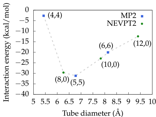
FIGURE 4.2: Unrelaxed interaction energies as a function of the nanotube diameter.
