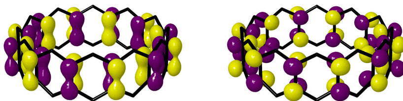
FIGURE 3.13: Symmetric (left) and antisymmetric (right) MO associated to the energies \varepsilon_1(k\theta = \pi) and \varepsilon_4(k\theta = \pi) for a [12]cyclacene. Hydrogen atoms are omitted.
