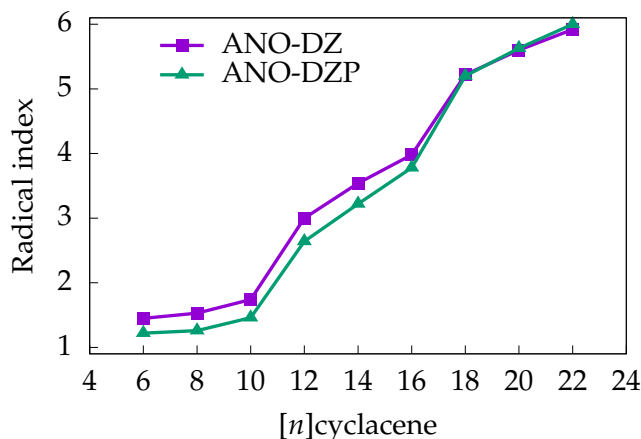
FIGURE 3.17: Effective number of unpaired electrons with respect to the system size.
