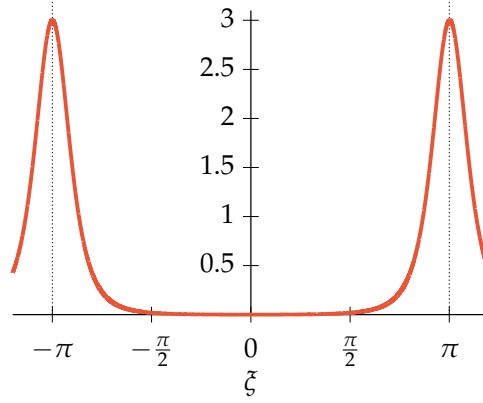
FIGURE 3.7: Squared integral in b^2 units contributing to the planar components of the TPS.
