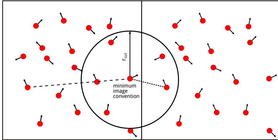
FIGURE 2.4: Example depicting the concept of cutoff radius and minimum image convention.
