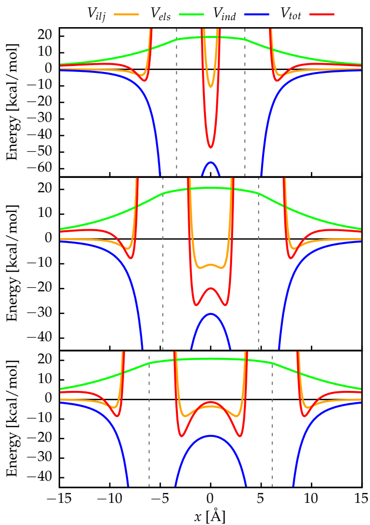
FIGURE 4.13: Potential energy profiles for (5,5), (7,7) and (9,9) CNTs from top to bottom. The dashed vertical lines show the position of the nanotube wall.
