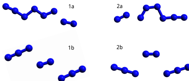
FIGURE 4.25: Transition state structures of the decomposition reactions in gas phase for the EEE conformer (1a and 1b) and the EZE conformer (2a and 2b).
