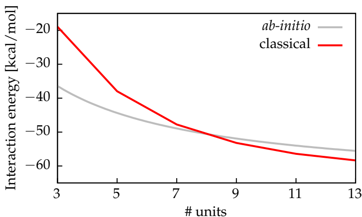
FIGURE 4.10: Comparison of classical and quantum-chemical interaction energies for \beta = 8 .
