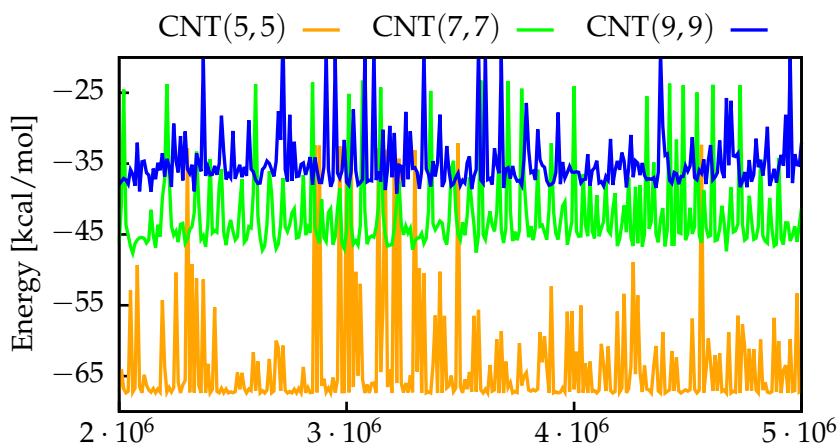
FIGURE 4.16: Adsorption energy of the azide anion inside different carbon nanotubes.
