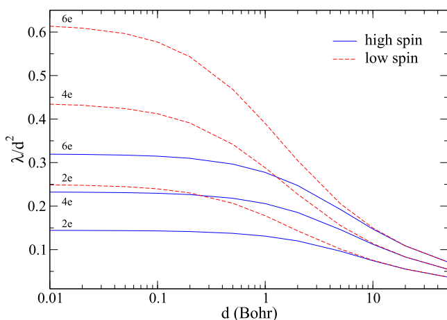
FIG. 8. The scaled FCI localization tensor \lambda/d^2 as a function of the mean distance d (please note the logarithmic scale).
