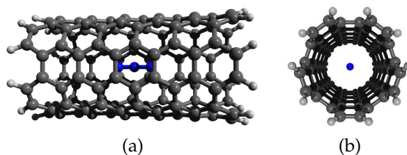
FIGURE 4.1: Side (a) and front (b) view of the geometry used for the unrelaxed interaction energy calculations.
