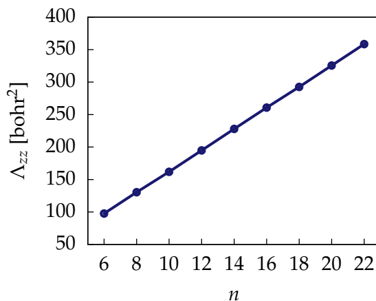
FIGURE 3.18: The total axial component of the TPS computed with the CASSCF wave function.
