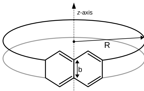
FIGURE 3.2: Simplified scheme of a cyclacene.
