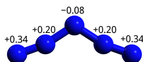
FIGURE 4.20: Partial atomic charges of the isolated N_5^+ cation.
