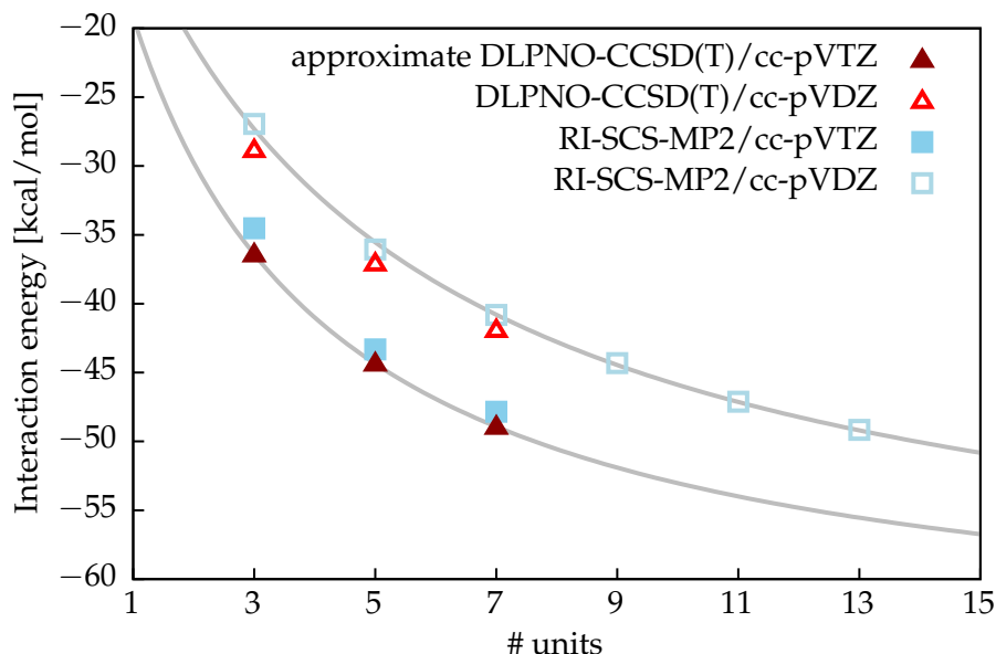
FIGURE 4.9: Interaction energy as a function of tube length. The solid lines are fits to the RI-SCS-MP2/cc-pVDZ and the approximate DLPNO-CCSD(T)/cc-pVTZ points.
