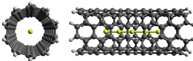
FIGURE 4.27: Front and side view of a Be_5 chain inside a CNT(5,5).
