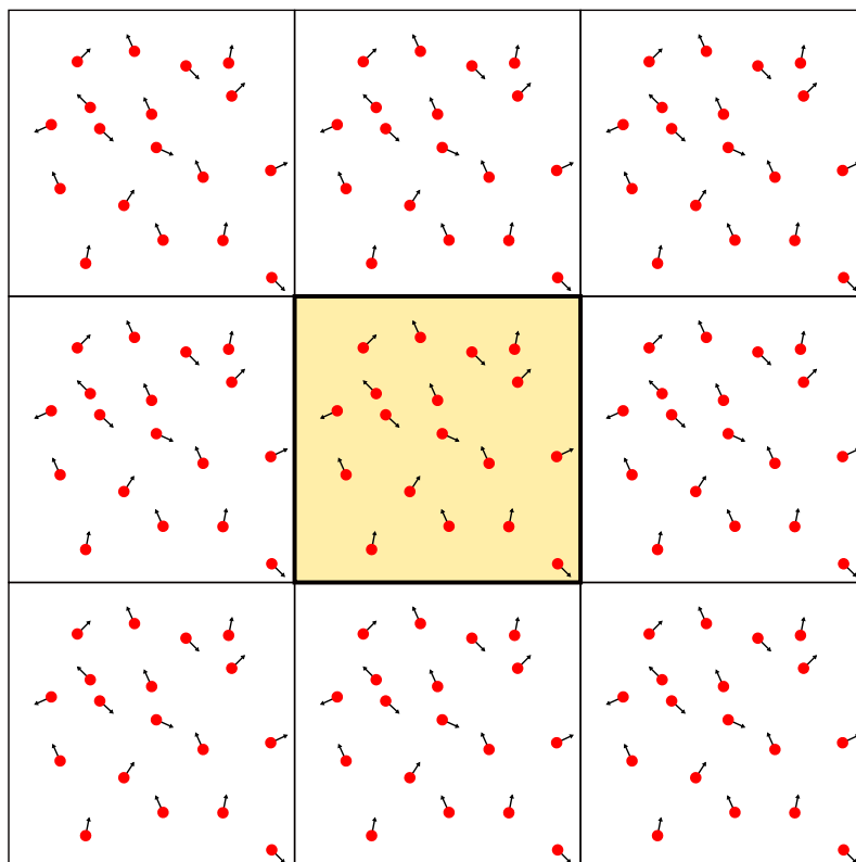
FIGURE 2.2: Model system example in a two-dimensional square box with periodic boundary conditions. Red discs represent the position of the particles, black arrows their velocity vector. As can be seen, the central highlighted box is replicated in both dimensions.
