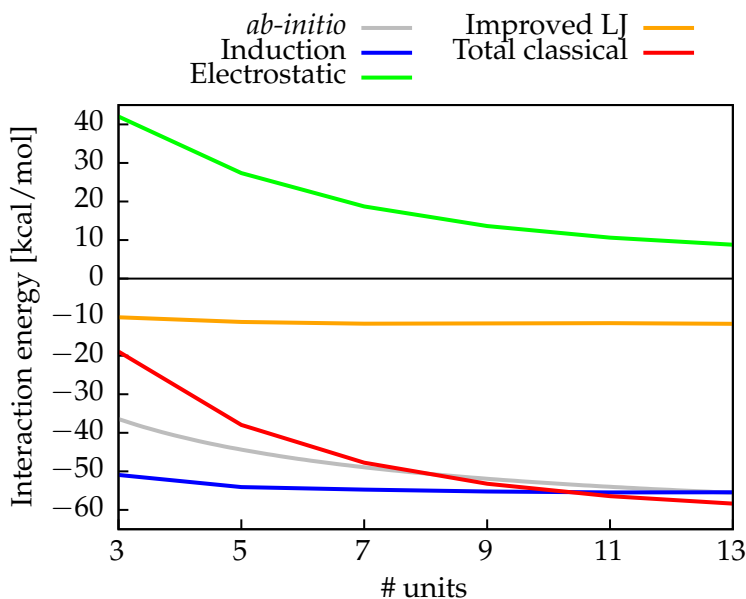
FIGURE 4.11: Individual potential contributions to the interaction energy.
