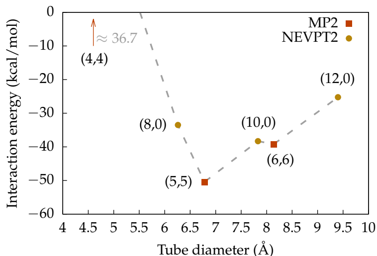
FIGURE 4.17: Unrelaxed interaction energies as a function of the CNT diameter.
