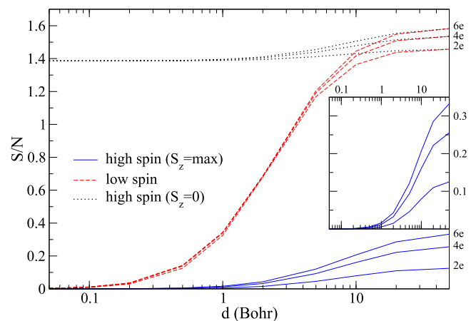
FIG. 9. The total electronic entropy per electron S/N as a function of the mean distance d (please note the logarithmic scale). Inset: a zoom of the entropy of the HS state ( S_z = \max ).
