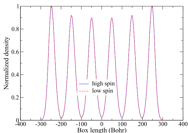
FIG. 6. The electron density for d = 100.0 Bohr.
