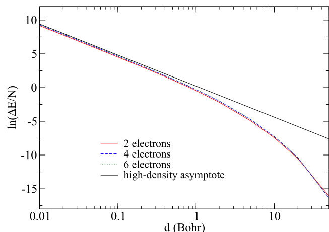
FIG. 2. The natural logarithm of the HS-LS energy-difference per electron obtained within FCI as a function of the mean distance d (please note the logarithmic scale).
