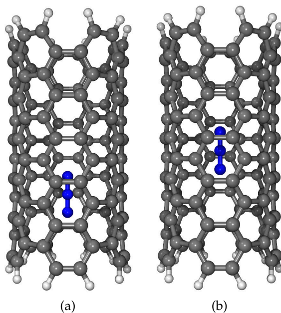
FIGURE 4.4: Starting (a) and final (b) position of the N_3^- ion inside the the (5,5)CNT.
