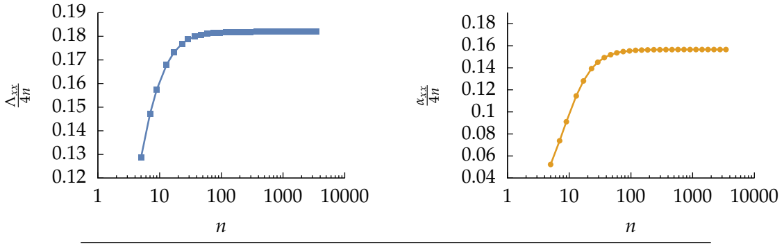
FIGURE 3.8: Planar component of the per-electron TPS (left) and per-electron polarizability (right) in b^2 units and \frac{b^2}{t} , respectively.
