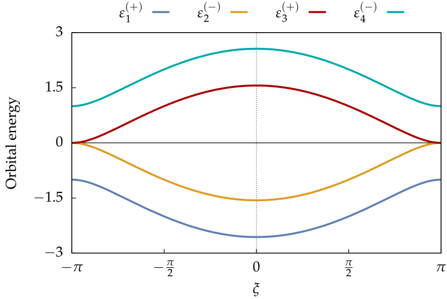
FIGURE 3.4: Energy bands (in t units) at Hückel level of theory for a = 0 and t = 1 .
