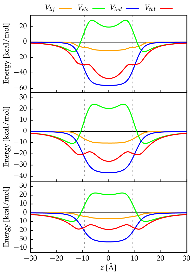
FIGURE 4.14: Potential energy profiles for (5,5), (7,7) and (9,9) CNTs from top to bottom. The dashed vertical lines show the position of the nanotube openings.
