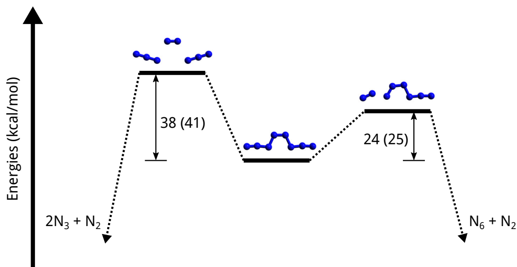
FIGURE 4.24: Potential energy surface showing the N_8 decomposition pathways in gas phase. Molecules and numbers depicted correspond to the EZE conformer, while the values in parenthesis refer to the EEE conformer.
