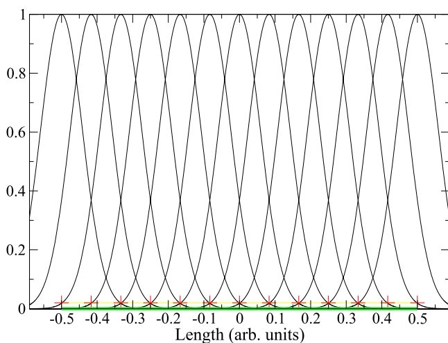
FIG. 1. Example of the tiling of a segment of length L = 1 with gaussians to describe 1 electron ( g = 12 ). Continuous lines (black): the gaussian functions; plus symbols (red): positions of the fractional positive point charges.
