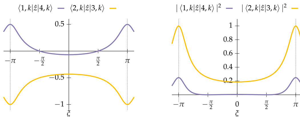
FIGURE 3.5: Nonvanishing integrals (left) and squared integrals (right) in b and b^2 units, respectively, contributing to the axial component of the TPS.
