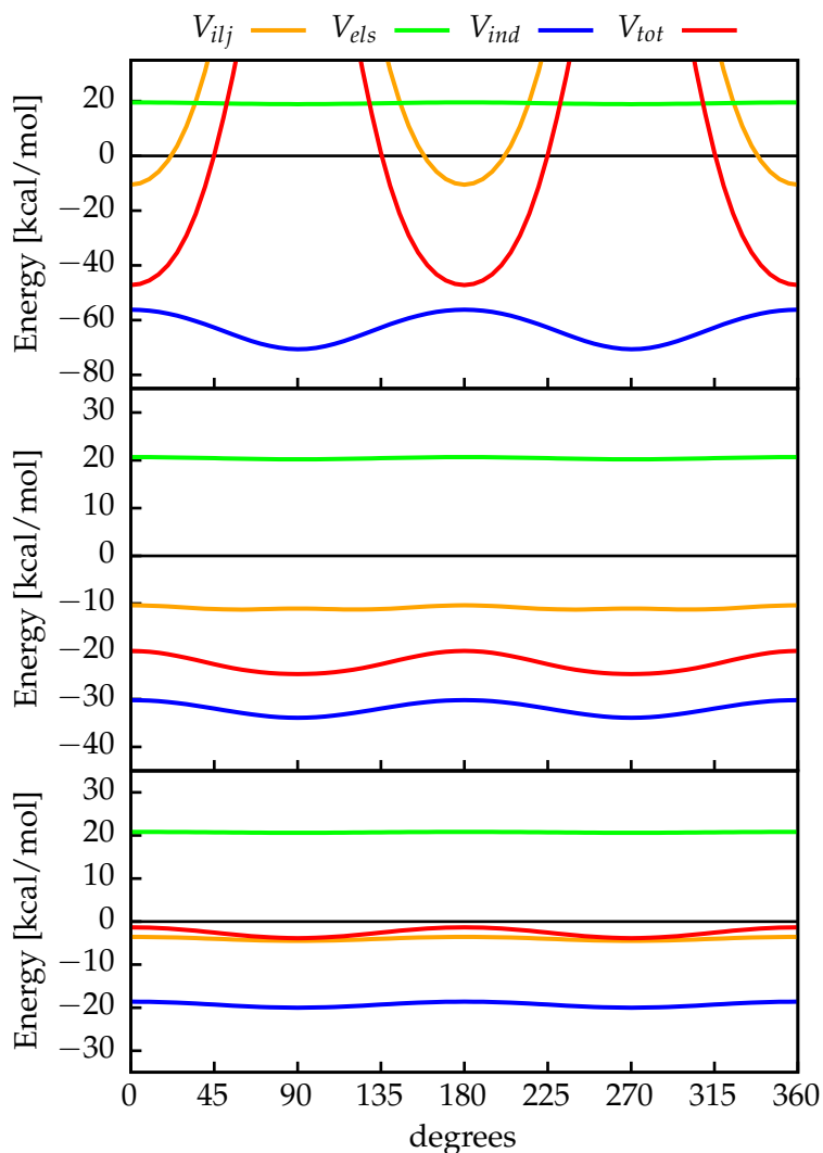
FIGURE 4.15: Potential energy profiles for (5,5), (7,7) and (9,9) CNTs from top to bottom.
