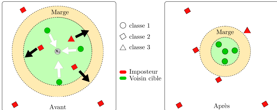
FIGURE 5.8 – Illustration de la méthode LMNN [177]
