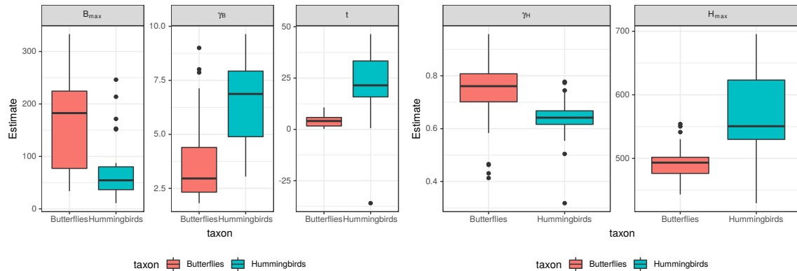
Figure 2: Both hummingbirds and butterflies display a large diversity of hues and brightness, as well as angle dependency in hue and brightness. The butterflies species we measured tend to have multilayer structure parallel to the sample surface (no tilt), which is not the case for hummingbird. The outlier for tilt in hummingbirds is the back of Aglaeactis cupripennis .
