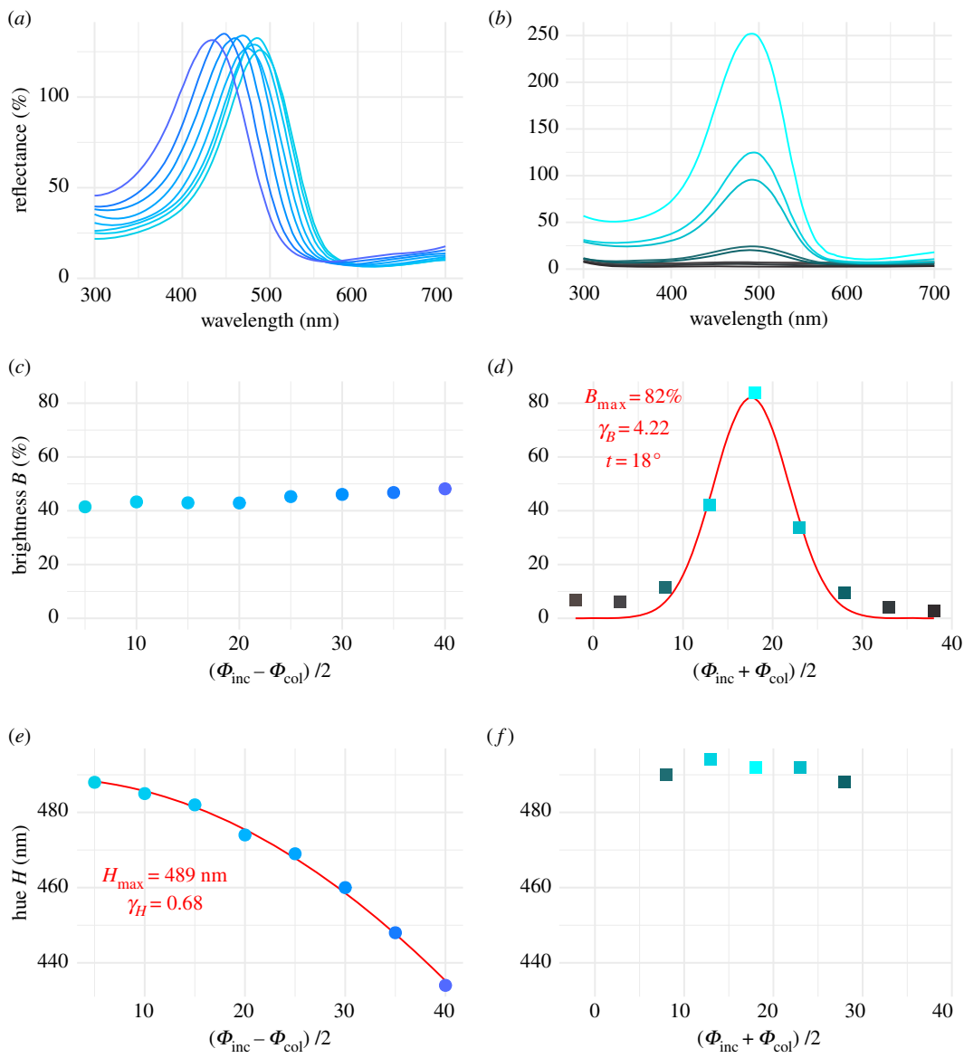
Figure 4. Spectra (a,b) and corresponding values of brightness (c,d) and hue (e,f) at different angle configurations for the breast patch of the hummingbird Heliomaster furcifer along the \Phi_{inc} - \Phi_{col} = \text{const.} (a,c,e; data points with round shape) and \Phi_{inc} + \Phi_{col} = \text{const.} (b,d,f; data points with square shape) lines. Colours correspond to the conversion of the spectra in human vision using the CIE10 visual system. As expected, brightness is constant when \Phi_{inc} - \Phi_{col} = \text{const.} and has a Gaussian shape when \Phi_{inc} + \Phi_{col} = \text{const.} Conversely, hue has a cosine shape when \Phi_{inc} - \Phi_{col} = \text{const.} and is constant when \Phi_{inc} + \Phi_{col} = \text{const.} The red lines correspond to the fit of the functions after parameter estimation, with the values of the parameters. The R script to produce this figure is available in electronic supplementary material.
