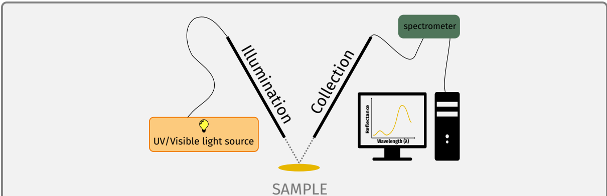
Figure 1.4: Drawing of a set-up to measure spectral reflectance from a sample: the light is brought from a lamp to the sample via an optical fibre (illumination fibre). The light reflected by the sample is then collected by a second optical fibre (collection fibre) which brings it to the spectrophotometer.
