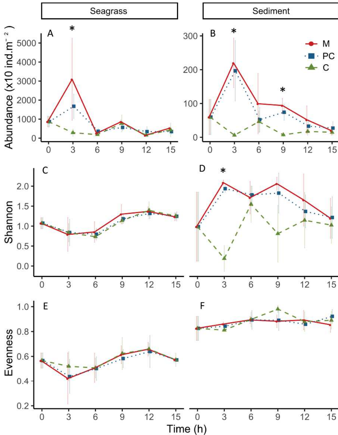
Fig. 4: Total abundance (A and B, note the different scales for the two habitats), Shannon diversity index (C and D) and Pielou's equitability index (Evenness) in the seagrass meadow (A, C and E) and sediment (B, D and F) habitats. Dots represent the average, whereas the vertical bars are standard deviations, for each treatment (M, PC and C). Asterisks indicate significant differences between treatments at \alpha = 0.05 .
