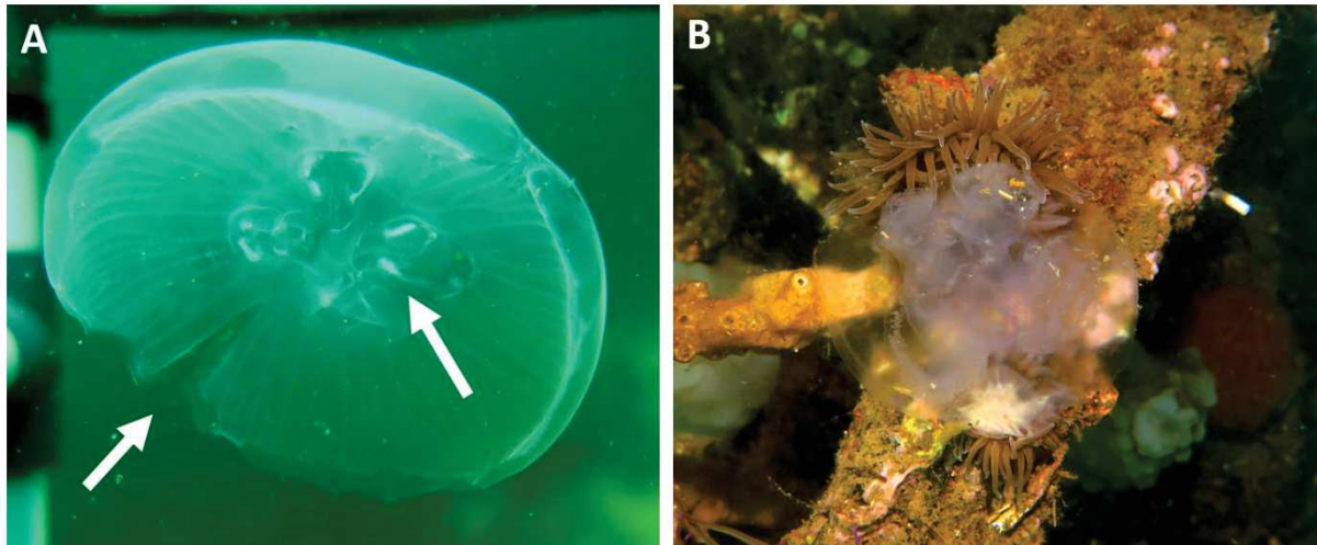
Fig. 3: A. coerulea medusae consumed by pelagic and benthic predators in the Thau lagoon. A) Medusae after being bitten by bogues. The arrows show the bites of the fish on the umbrella margins and gonads. B) Medusae consumed by anemones.
