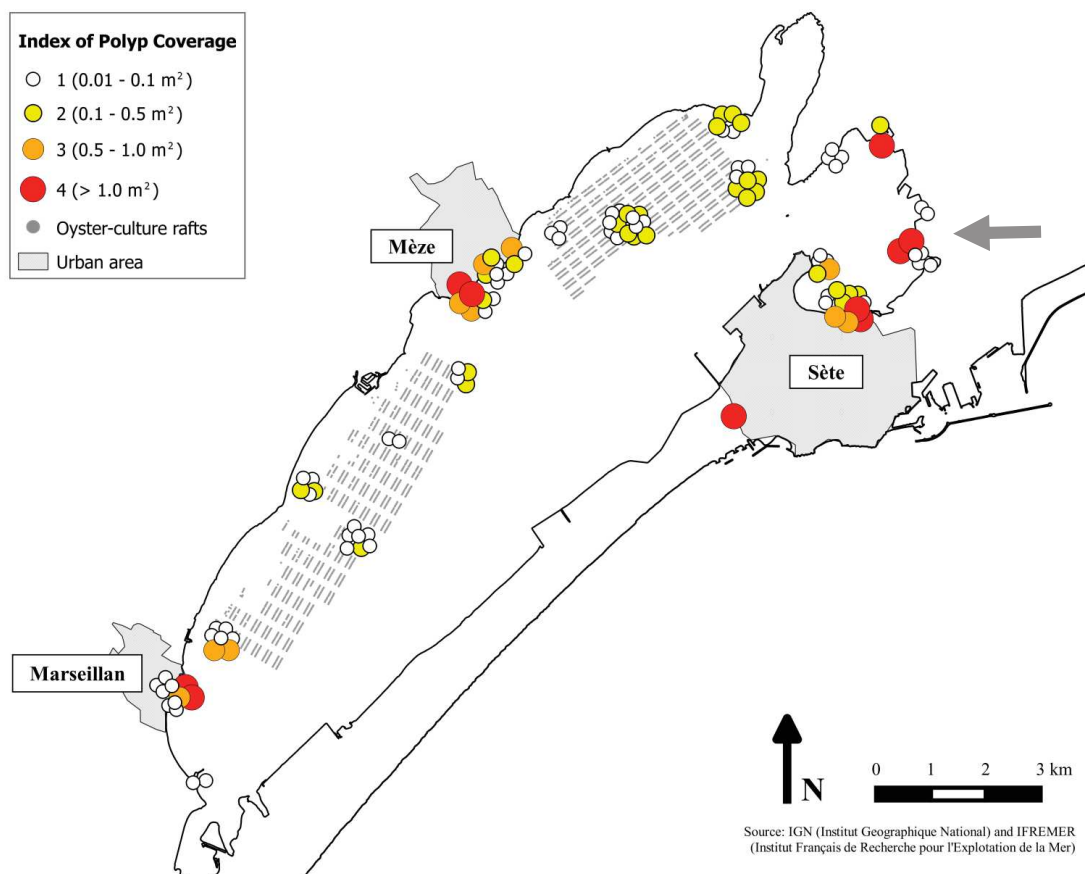
Fig. 7: Distribution of the sub-populations of A. coerulea scyphistomae in the Thau lagoon. A sub-population was defined as one or several patches of scyphistomae, covering the same continuous substrate type. The size of each sub-population was visually estimated according to a semi-quantitative index system (Index of Polyp Coverage, Marques et al. 2015b). The biggest aggregation ever observed in the lagoon was found on the underside of a submerged boat, near an old industrial concrete pontoon (grey arrow).
