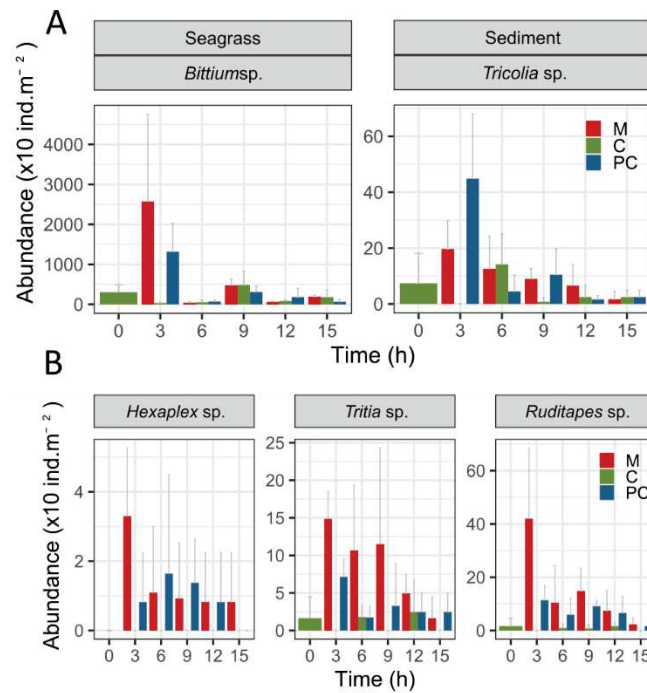
Fig. 7: Abundance of the taxa that showed significant differences (after ManyGLM) between treatments at 3h in both habitats (A) and between treatments over the whole study period on the sediment habitat (B). Note the different scales.
