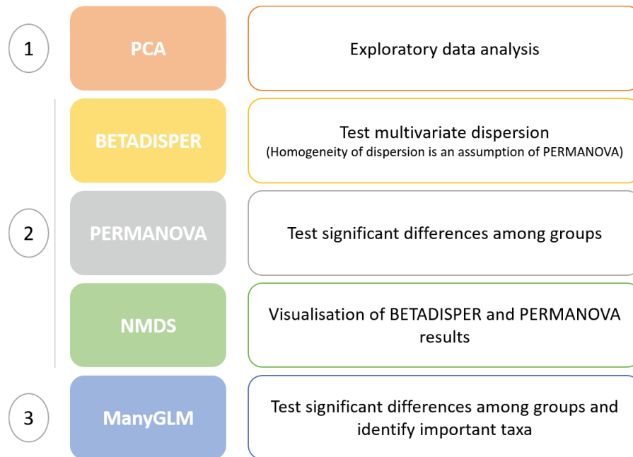
Fig. 1 Schematic representation of the analysis used to assess changes in the community composition and their specific objectives.
