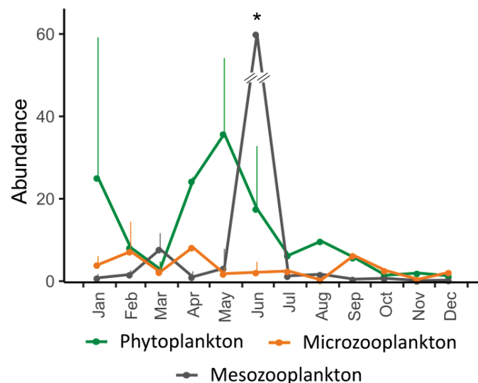
Fig. 3 : Temporal variability of the abundance of phytoplankton ( \times 10^3 cell.L -1 ), microzooplankton ( \times 10^3 cell.L -1 ) and mesozooplankton ( \times 10^3 ind.m -3 ) collected in the Thau lagoon during the study period. All values represent monthly means \pm SD. In June 2017 (*), the mean and SD of the abundance of mesozooplankton were 90\,895 \pm 107\,072 ind.m -3 .
