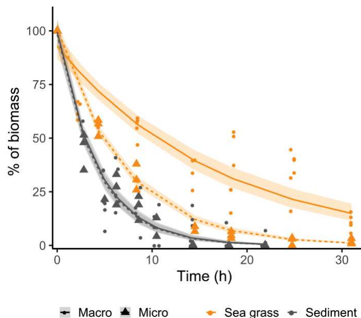
Fig. 2: Degradation of A. coerulea in both habitats for each accessibility scenario. Exponential decay models were fitted (lines) to the non-averaged data of biomass (in % of the initial wet weight), with 95% confidence intervals (shadow areas).
