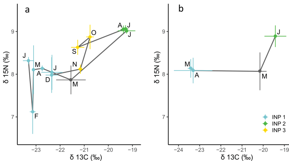
Fig. 6 : Time trajectory of the evolution of the isotope signature, averaged by month, from scyphistomae (a) and medusae (b). Letters represent months (from January 2017 to January 2018). Coloured points represent isotopic niche periods defined after cluster analysis: INP 1 is from January to April 2017, December 2017 and January 2018; INP 2 is from June to August 2017 and INP 3 is from September to November 2017. May represent a transitional period between the INP1 and INP2 and was therefore not included in any INP.
