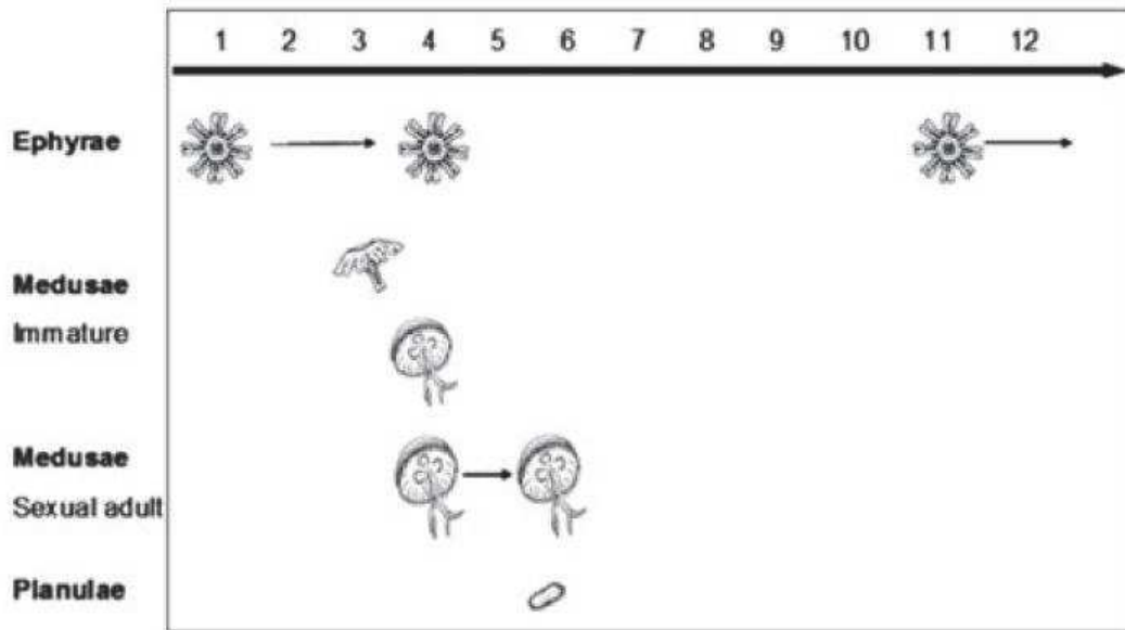
Fig. 9 Representation of the timing of occurrence of the different pelagic life stages of A. coerulea in the Thau lagoon. Numbers represent months (Bonnet et al. 2012).
