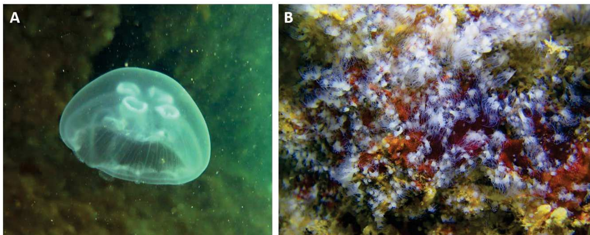
Fig. 5: Aurelia coerulea medusae (A) and scyphistomae (B). Photographs were taken in the Thau lagoon by Raquel Marques.
