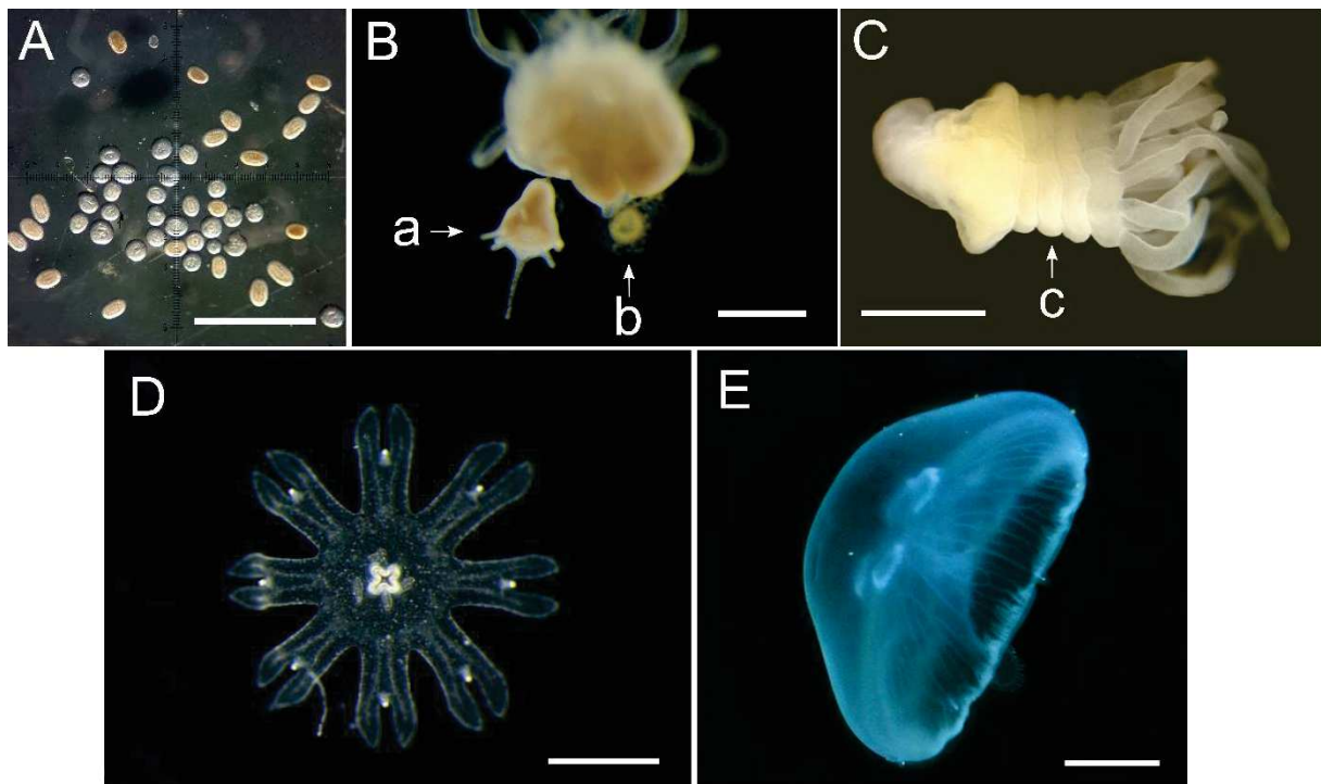
Fig. 2 The different stages of A. coerulea life cycle. A) planulae, B) scyphistomae, producing one bud (a) and one podocyst (b), C) strobila and its strobila disks (c), D) ephyrae and E) medusae. All white bars represent 1 mm, except in E where it represents 1 cm. Photographs taken by Raquel Marques.
