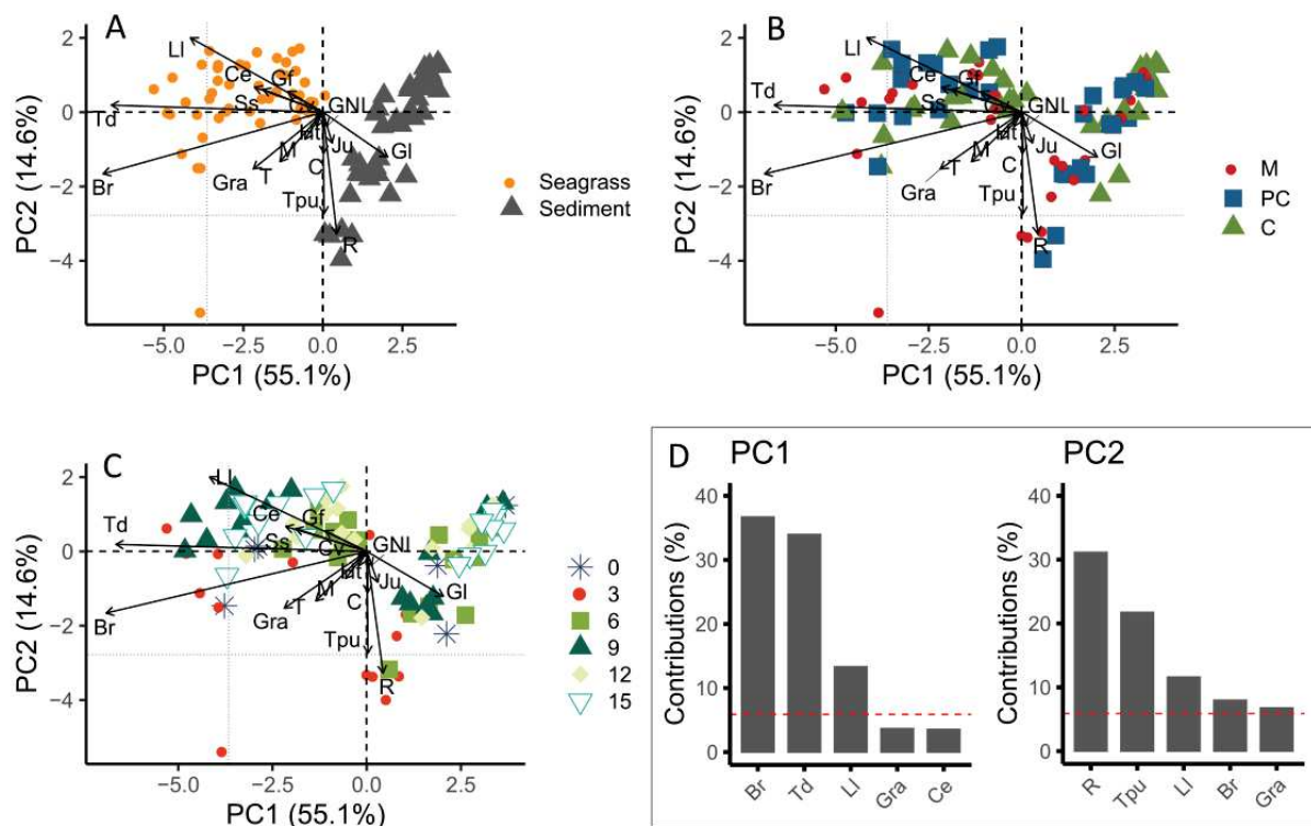
Fig. 5: Results of Principal Component Analysis (PCA). In A, B and C biplots of samples (points) and taxa (arrows) are presented. In A samples are identified according to the habitat (seagrass meadows and sediment), in B the samples are identified according to their treatment (M, PC or C) and in C the samples are identified according to sampling time (in h). Only the first two axes (PC1 and PC2) were retained since they represent the majority of the variability of the data (69.7%). Grey dotted lines are indicative thresholds to identify the samples with higher
