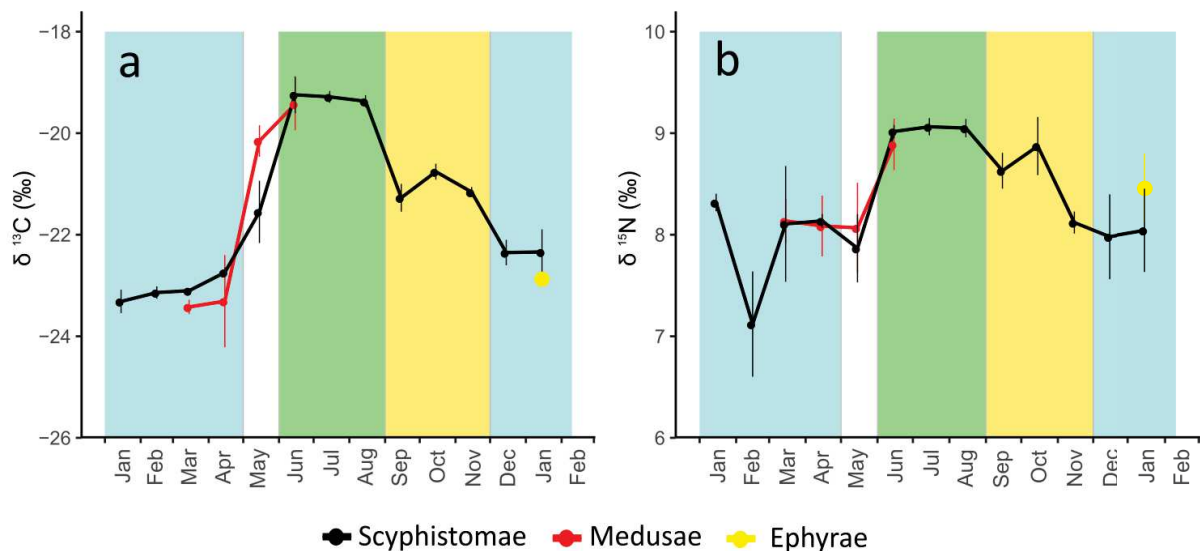
Fig. 5: Temporal variability of \delta^{13}\text{C} (a) and \delta^{15}\text{N} (b) of scyphistomae, medusae and ephyrae. All values represent monthly means \pm SD. Background colours represent the different isotopic niche periods (blue: INP 1, green: INP 2, yellow: INP 3; see Fig.6). May represents a transitional period and not included in any INP.
