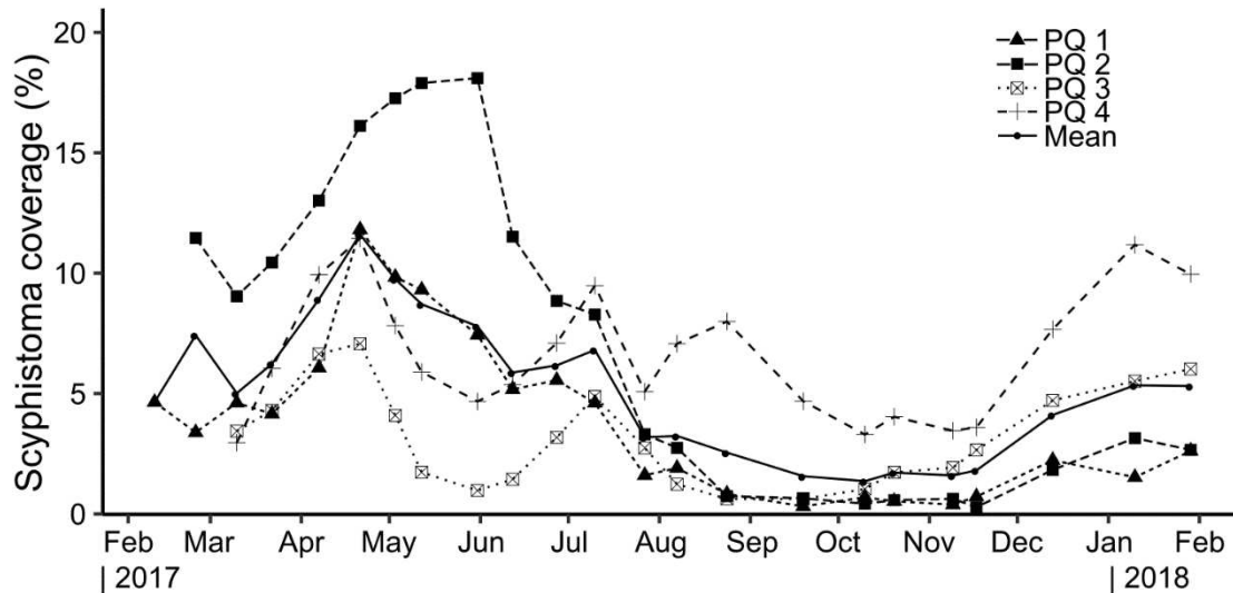
Fig. 5 Variation of A. coerulea scyphistoma coverage in each photoquadrats (PQ) and the mean of all photoquadrats, during the study period
