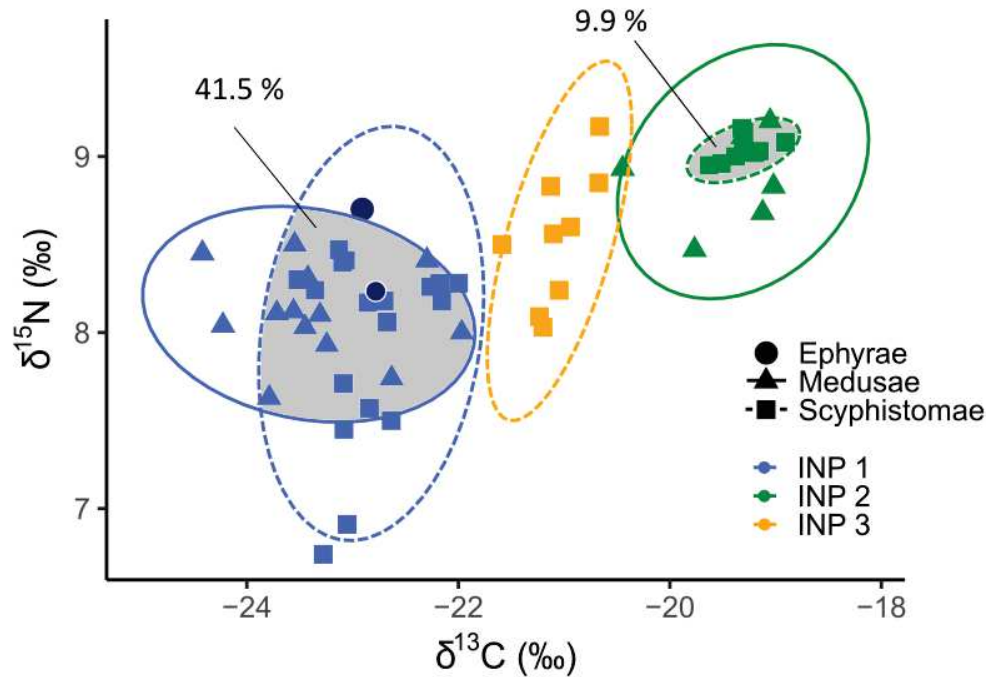
Fig. 9: Biplot of isotope values of A. coerulea ephyrae, medusae and scyphistomae. Ellipses indicate their isotopic niche in Thau lagoon, during the different isotopic niche periods (as 95% confidence ellipse of the bivariate means). Grey areas and associated values on the graph indicate the percentage of overlap, when observed.
