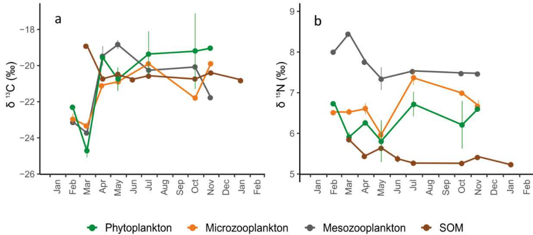
Fig. 7: Monthly variability of the \delta^{13}\text{C} (a) and \delta^{15}\text{N} (b) of the sources of OM collected in this study.
