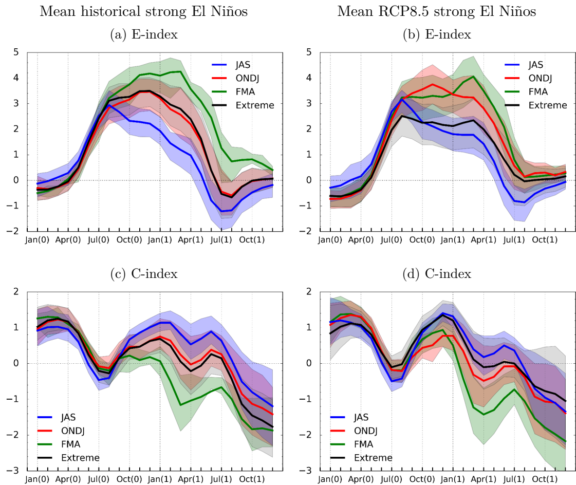
Figure 5.6 – Temporal evolution of (top) the E-index and (bottom) the C-index of strong El Niño events, for the composite events of (left) the 42-members of the historical simulation and (right) the 40-members of the RCP8.5 simulation. Composites consist of strong events whose E-peak occurs in (blue) July-August-September (JAS), (red) October-November-December-January (ONDJ), (green) in February-March-April (FMA). In black lines are the composite event according the definition of extreme events by Cai et al. (2014) . The shadow corresponds to events of the strong regime between the 25th et 75th percentiles.
