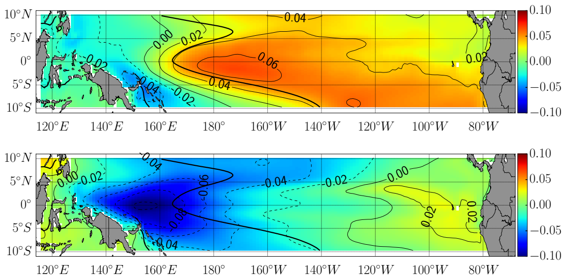
Figure 4.6 – Regressed spatial patterns of the equatorial SSTA onto the (top) ENSO-like and (bottom) ENSO-induced TPDV modes. The TPDV modes are defined from an EOF analyse of the decadal equatorial subsurface temperature anomalies averaged between 5°S-5°N for the CESM-LE PI-control simulation (1801 years). The black line is the mean 28°C isotherm, a proxy of the warm pool. The decadal equatorial subsurface temperature anomalies, de-seasoned and linearly detrended, are computed by applying a 31 yr running-mean filter.
