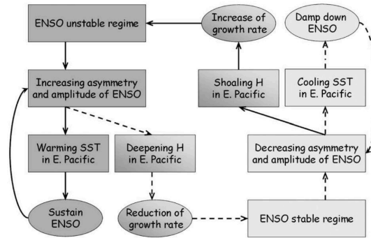
Figure 1.25 – Schematic diagram showing the interactive two-way feedback mechanism of decadal variability in the tropical Pacific. The figure is reprinted from Choi et al. (2009).
