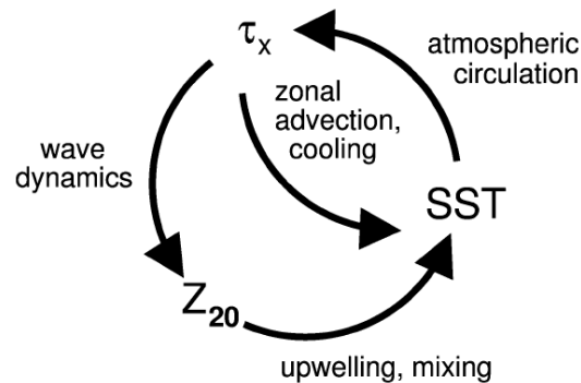
Figure 1.12 – Main positive feedbacks in ENSO as a cycle. Z_{20} denotes the thermocline depth through the depth of the isotherm 20^\circ\text{C} and \tau_x denotes the zonal wind stress (Reprinted from Zelle et al. (2004) ).
