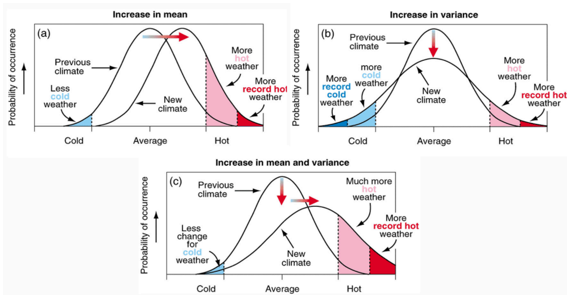
Figure 2.15 – Schematic representations of the PDF of a normally distributed climate variable such as temperatures. Shaded areas correspond to the probability of occurrence of extreme events, that is events in the tails of the distribution, that occur infrequently. Changes in the probability of occurrence of extreme events are affected by changes (a) in the mean, (b) in the variance, and (c) in both the mean and the variance. The figure is reprinted from IPCC Third Assessment Report (AR3, see https://www.ipcc.ch/report/ar3/wg1/the-climate-system-an-overview/ ).
