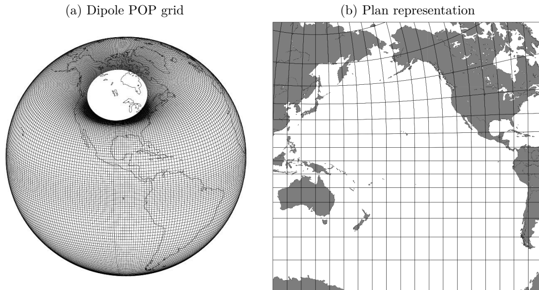
Figure 2.5 – Representation of the Arakawa B-grid used by POP ocean model. 2.5a shows the orthogonal curvilinear mesh-grid with the displaced pole (from Smith et al. (2010)). 2.5b shows the projection of the mesh-grid over the Pacific ocean onto plan coordinate (drawn by Charles Baillon).
