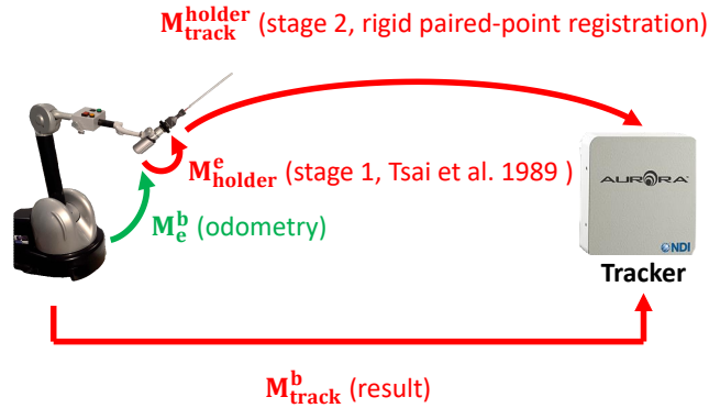
(b) Second approach: calibration method by [Tsai and Lenz, 1989] to estimate {}^eM_{holder} , then paired-point registration to estimate {}^{holder}M_{track} and {}^bM_{track}
