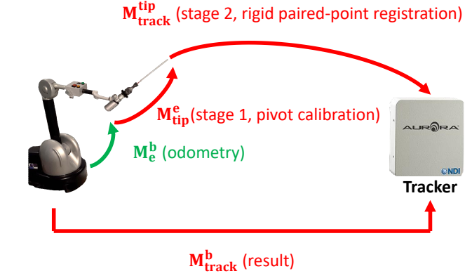
(a) First approach: pivot-point calibration to estimate {}^eM_{tip} , then tracker measurements to obtain {}^{tip}M_{track} , and paired-point registration to estimate {}^bM_{track}
