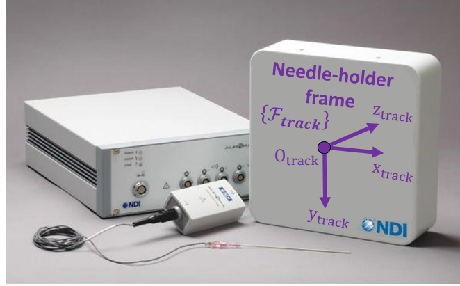
(a) The Aurora electromagnetic needle tracker [NDI, 2019a], its direct Cartesian coordinate frame \{F_{track}\} and instrumented needle [NDI, 2019d]
