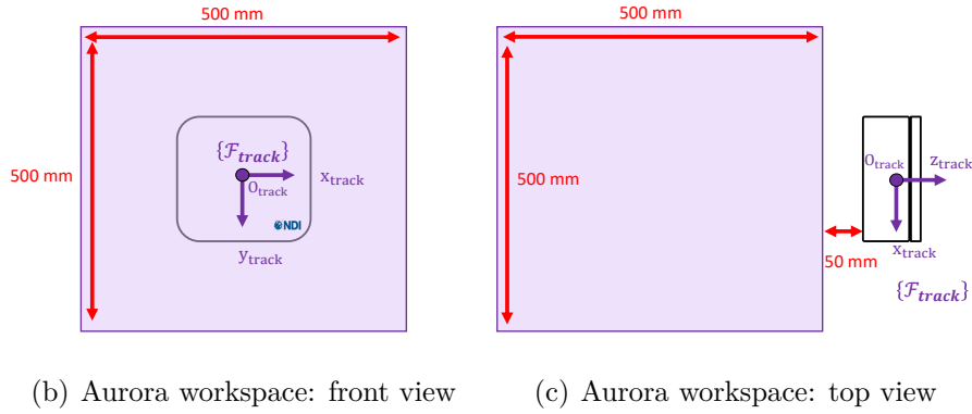
Figure 3.5 – The Aurora tracker and instrumented needle. The workspace of the tracker is a 500 \times 500 \times 500 \text{ mm}^3 cube located 50 mm away from the tracker.
