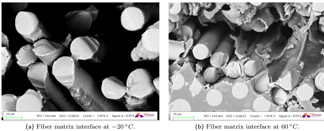
Fig. 14: SEM-BSE observations of the fiber / matrix interface at both -20^{\circ}\text{C} and 60^{\circ}\text{C} .
