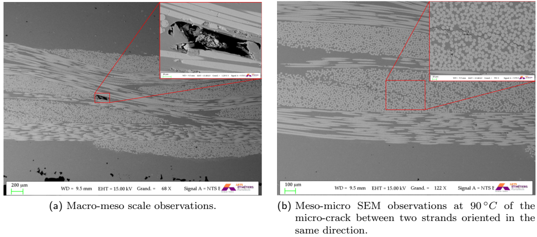
Fig. 11: Macro-meso and meso-micro SEM-BSE observations at 90°C.
