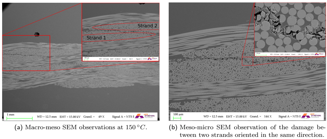
Fig. 12: Macro-meso and meso-micro SEM-BSE observations at 150°C.
