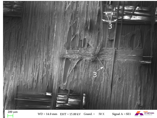
(d) Macroscopic SEM observations of the created surfaces at 60^{\circ}C . Items 3 shows fiber pull-outs.
