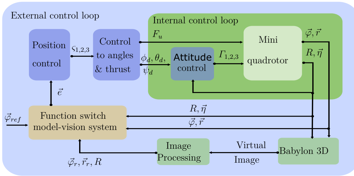
Figure 5.4 – Quadrotor system navigation strategy: Simulation scheme.
