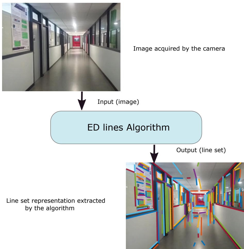
Figure 4.5 – The EdLines algorithm is taken as a function where the input is the image acquired by the camera, and the output is a lines set. Each line has as information the initial and final point.
