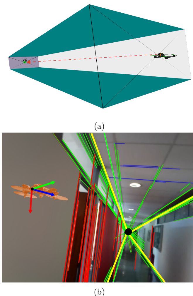
Figure 4.1 – Quadrotor flying into a corridor, the head-direction is given by a vanishing point, and the pose of the quadrotor is obtained geometrically using principal lines which are estimated using data from the corner borders.
