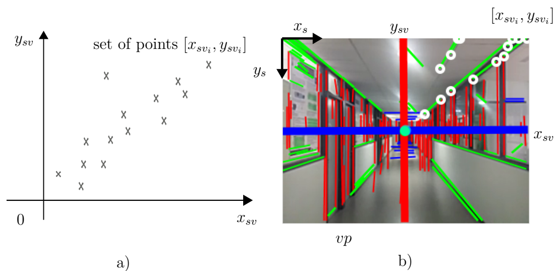
Figure 4.11 – a) Set of points to estimate a line in a coordinate system, b) set of point (x_{sv_i}, y_{sv_i}) of the frame image plane, vanishing point vp , and vertical line y_{sv} and horizontal line x_{sv} .
