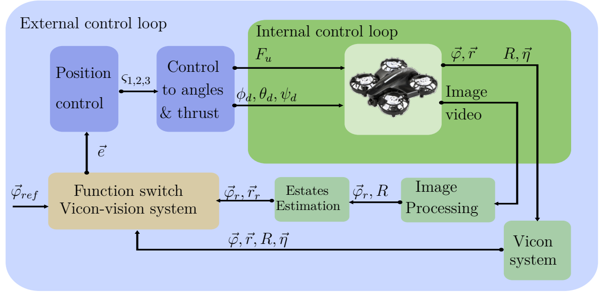
Figure 5.6 – Quadrotor system stabilization strategy: Real video scheme.
