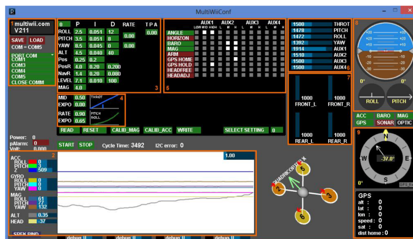
Figure 6.12 – Multiwii GUI.
