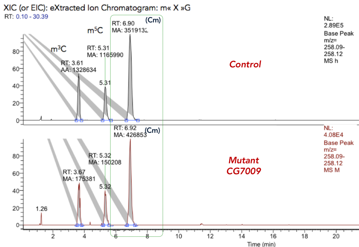
Figure 36. Cm 32 formation in D. melanogaster tRNA Phe seems independent of CG7009. LC-MS analysis on the Cm 32 abundance in tRNA Phe extracted from heterozygotes CG7009 e02001 / TM6, Tb, Sb (upper panel) or trans-heterozygotes CG7009 e02001 / Def3340 (lower panel).
