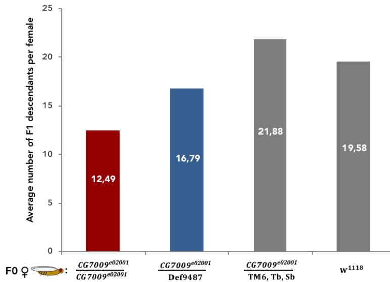
Figure 20. Effect of CG7009 mutation on the fertility in females. A. Rationale for the experiment on the semi-sterility in females from Bloomington stock 18008 (allele CG7009 e02001 ). The experiment consisted in comparing the total number of descendants arising from the cross of homozygous females CG7009 e02001 / CG7009 e02001 with males w 1118 (red panel, upper cross) and the total number of descendants arising from the cross of trans-heterozygous females CG7009 e02001 / Def9487 with males w 1118 (red panel, lower cross). As control the total number of descendants arising from the cross of w 1118 flies (blue panel, upper cross) of females w 1118 and trans-heterozygous males CG7009 e02001 / Def9487 were to be determined. B. The result is represented as an average of the descendants per female from the following crosses: 2 crosses between 3 males w 1118 and 8 females CG7009 e02001 / CG7009 e02001 (red graph); 2 crosses between 3 males w 1118 and 8 females CG7009 e02001 / Def9487 (blue graph); 1 control cross between 3 males w 1118 and 8 females CG7009 e02001 / TM6, Tb, Sb (first grey graph); and 1 control cross between 3 males w 1118 and 8 females w 1118 (second grey graph). The number of descendants was counted for 4 flips of parents in the indicated crossings and determined first as an average result at each flip by taking into account the dead parents. The final results represent another average value determined from the number of descendants per female for each flip and cross.
