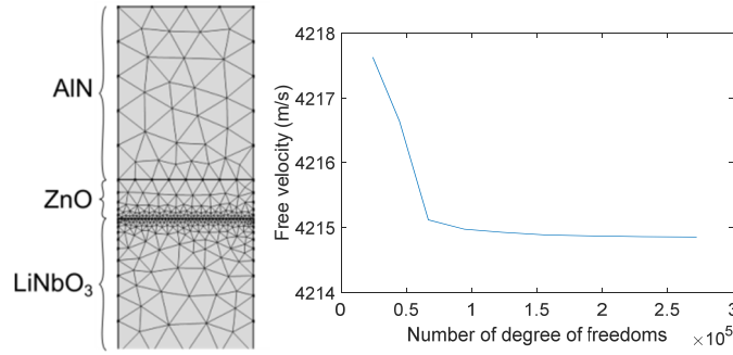
Figure 2.26 Convergence study, for the unit-cell model used to compute the properties of the package-less sensor. (Left) The FE mesh used for the convergence study. The pictured mesh has a low number of elements (18252 DOFs) for the sake of representation. (Right) Convergence of the free velocity vs. number of degrees of freedom.
