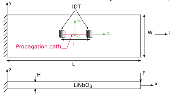
Figure 2.3 Schematic of the structure studied by Nalamwar et al. [62]. (X, Y, Z) is the coordinate system of the geometry, (Xc, Yc, Zc) is the crystal orientation coordinate system ; L is the length of the beam (33 mm); W is the width of the beam (5 mm); H is the thickness of the beam (1.97 mm); l is the length between the IDTs (5.08 mm); F is the bending force (1, 5, 10, 50 N).
