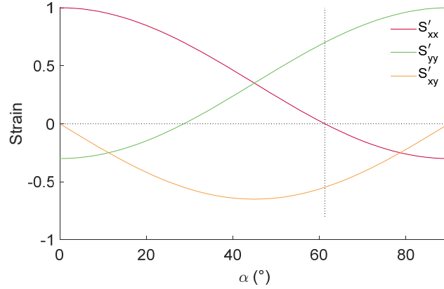
Figure C.1 Evolution of the in-plane strains versus the rotation angle \alpha .
