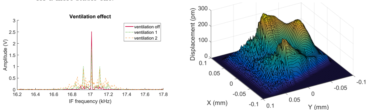
Figure 4.21 Influence of external vibration on the setup. (Left) Graph showing the effect of the ventilation on the IF. The graph shows the Fourier Transform of the IF signal from which the amplitude of the vibration is computed. The ventilation of the flow box has two settings for high and low aspiration. When the ventilation is turned off, the IF peak at 17015 Hz appears clearly. When the ventilation is activated on the first setting, noise starts to appear around the IF peak and weakens it. These effects are even more significant on the second setting of the ventilation. (Right) Picture showing the influence of the table isolation. The picture was obtained by turning off the air pressure supply by mistake during a scan. After it is turned off, the table takes several minutes to release all the air it contains. After that, the damping is completely inefficient and external vibration disturbs the measurement.
