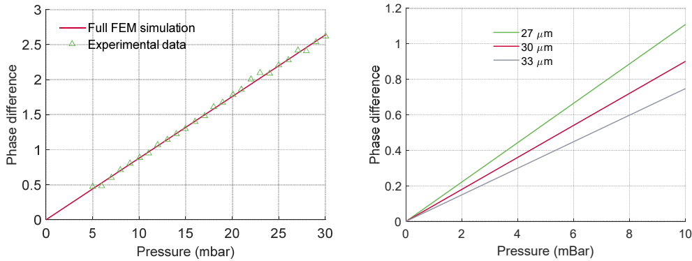
Figure 2.13 Sensitivity of the ICP sensor to pressure. (left) Computed sensitivity compared to the experimental results. (right) Sensitivity computed for different membrane thicknesses.
