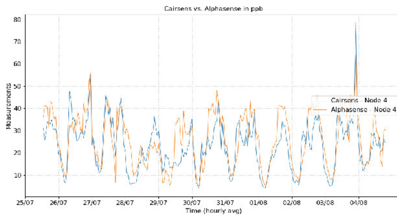
Figure 3.6: Comparison between Alphasense and Cairpol measurements.
