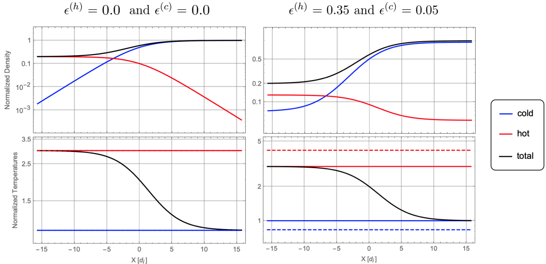
Figure 12.2: Comparison between density (top panels) and temperature (bottom panels) profiles in case \epsilon^{(h)} = \epsilon^{(c)} = 0 (left panels) and in case \epsilon^{(h)} = 0.35 , \epsilon^{(c)} = 0.05 (right panels).
