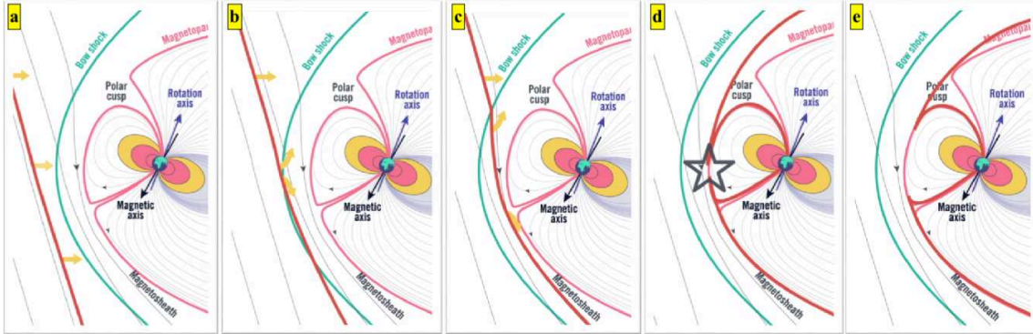
Figure 4.2: Cartoon showing a magnetic reconnection event happening at the magnetospheric sub-solar point. A solar wind magnetic field line comes from the left dragged by the solar wind (panel a). It passes the bow shock preserving its direction (panel b) and start to bend due to accumulation onto the magnetopause forefront (panel c). Suddenly, it reconnects to the Earth's magnetic field in a very localised point (star in the middle of panel d). The magnetic field topology of both solar wind and magnetosphere magnetic fields up to global scales are therefore modified (panel e). Credits: L. Rezeau.
