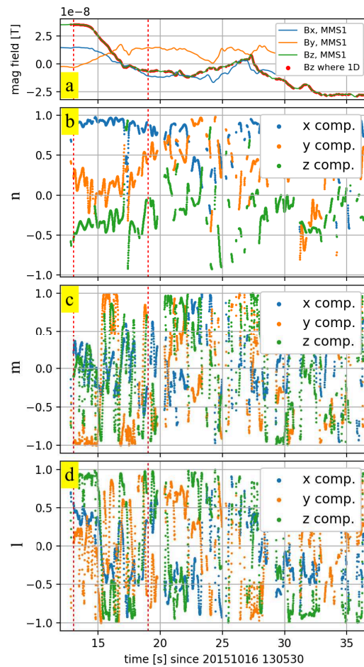
245 Figure 1. GSE components of magnetic field observed by MMS 1 (panel a, the sections in 246 red are the times when the structure is 1D), the l , m , and n components of the MP frame (pan- 247 els b, c and d) computed by means of the MDD method (Shi et al., 2005) for 16 October 2015, 248 13:05:30+60s, using burst mode data (128S/s). Note that the m and l directions oscillate rapidly 249 even during times where n is stable.
