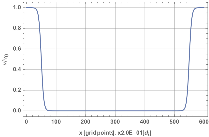
Figure 12.6: Visualisation of the spatial profile normalised non-homogeneous viscosity adopted in the 3fluid simulations to solve the boundary wave problem described in section 12.4.2.
