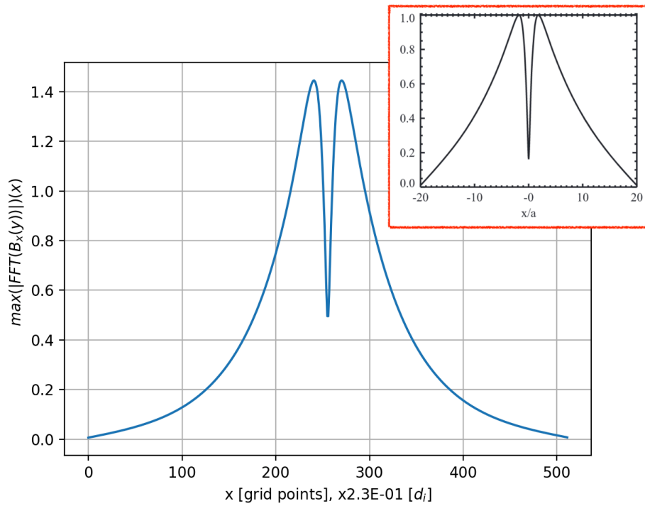
Figure 13.5: Tearing mode magnetic field eigenfunction ( \max(|FFT(B_x(y))|)(x) ) recorded at an evolved state in a 3 \rightarrow 2 fluid simulation. Inset to the figure it is shown the same profile obtained by numerical simulations adopting similar models and initialised with similar equilibria [120].
