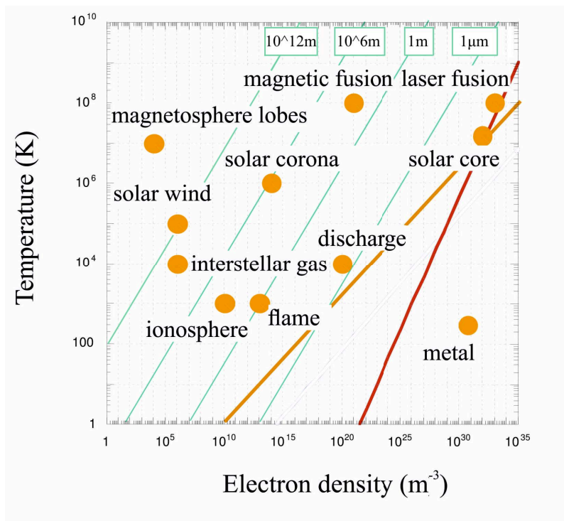
Figure 3.3: The position in the n - T parameter space of some plasmas found in nature. The green lines are four different loci defining four different mean paths. Below the red line, quantum effects have to be taken into account, above they can be neglected. Below the orange line binary interactions dominate the physics, whereas above the collective interactions are dominant. Credits: modified from [133]
