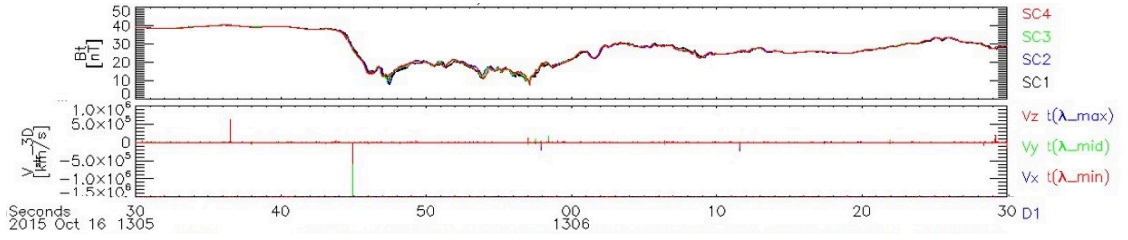
Figure 8.1: Computation of the magnetopause magnetic field structure velocity (bottom panel) during the Cr2 crossing (magnetic field shown on the top panel). The computation has been done by means of SPEDAS routines .
