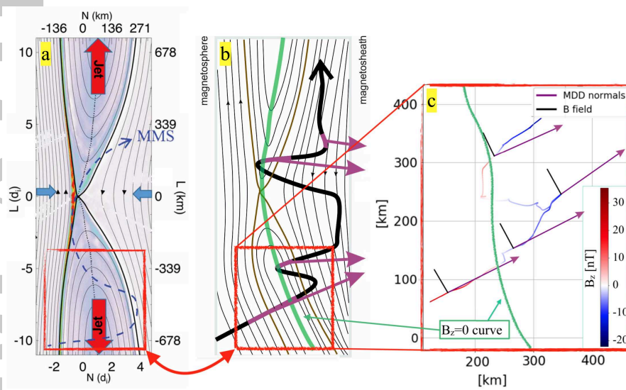
609 Figure 8. Comparison between the hand-made sketch made by (Burch et al., 2016c) (on the 610 left), a hand-made sketch suggested by the relative direction of the MDD normals with respect to 611 the local magnetic field and the Shue model (Shue et al., 1997) (central sketch) and the path ob- 612 tained automatically by our MVD technique applied on the 16/10/15, 13:05:42 UT - 13:06:04 UT 613 period (on the right). The automatic result concerns the portion of the path enclosed in the red 614 squares drawn on the hand made sketches. In both panels b and c the green curved lines joining 615 the B_z = 0 points are drawn by hand.
