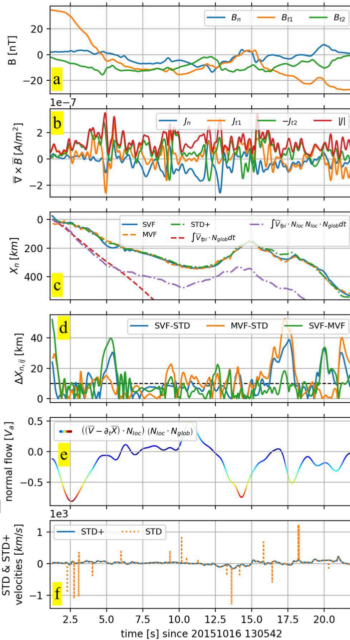
539 Figure 6. Magnetic field (panel a), curlometer current (panel b), X_N(t) coordinates (panel 540 c), \Delta X_{N,ij} differences (panel d), residual normal flow (panel e) and comparison between 541 |\partial_{t,0}(\mathbf{X}_{STD})| and |\partial_{t,0}(\mathbf{X}_{STD+})| recorded or computed during the 16 October 2015, 13:05:30+60s 542 crossing (here reduced to the 13:05:42+22s window).
