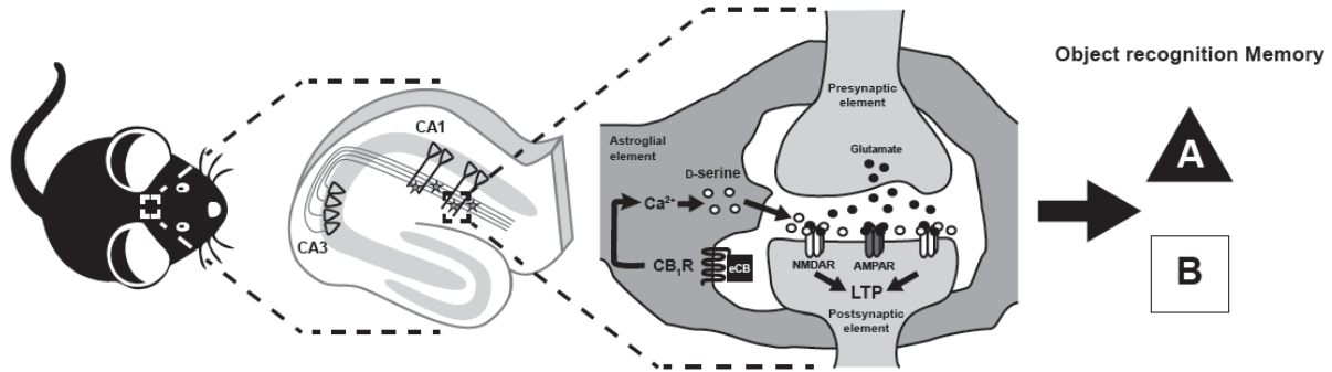
Figure S5. Schematic summary of the results. In adult mice, at the hippocampal CA3-CA1 synapse, astroglial CB1 receptors regulate cellular Ca 2+ levels, synaptic D-serine availability and thus D-serine-dependent synaptic NMDAR gating. By this means, astroglial CB1 receptors control synaptic NMDAR-dependent long-term potentiation (LTP) and object recognition memory. eCB; endocannabinoid.
