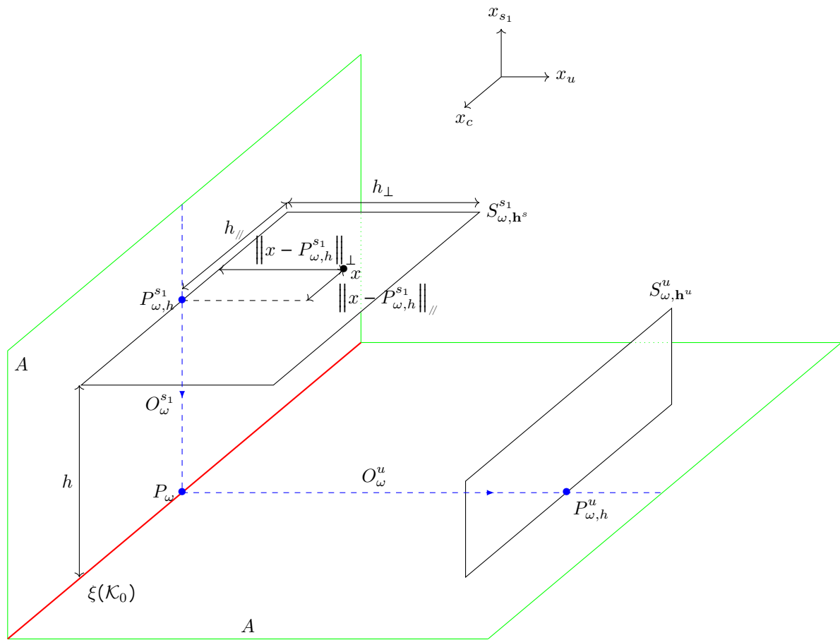
Figure 5.1 – Sections S_{\omega, \mathbf{h}}^{s_1} and S_{\omega, \mathbf{h}}^u . We omit the x_{s_2} -direction since we cannot draw in four dimensions. The Mixmaster attractor A is represented in green. The Kasner interval \xi(\mathcal{K}_0) is represented in red. The type II orbits arriving and starting at P_{\omega} are represented in blue.
