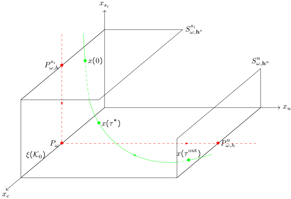
Figure 6.1 – Notations for local shadowing.
