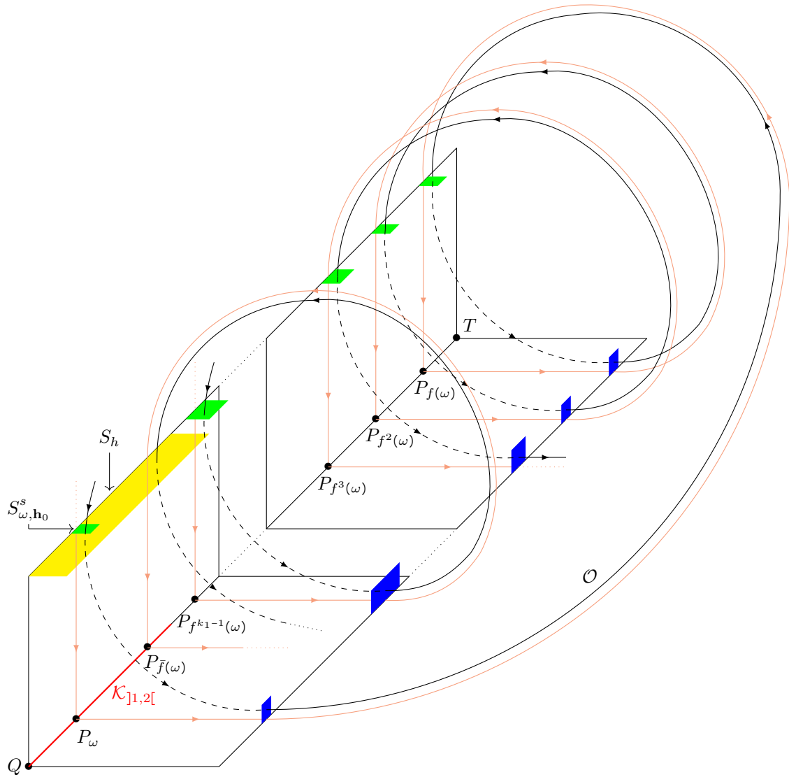
Figure 5.2 – A type IX orbit \mathcal{O} (in black) traveling close to the first era of the heteroclinic chain starting at P_\omega (in red), where \omega = [1; k_1, k_2, \dots] . The local sections S_{\omega, h_0}^s, S_{f(\omega), h_1}^s, \dots, S_{\bar{f}(\omega), h_{k_1}}^s are represented in green, while the local sections S_{\omega, h'_0}^u, S_{f(\omega), h'_1}^u, \dots, S_{\bar{f}(\omega), h'_{k_1}}^u are represented in blue. The era transition map \bar{\Phi}_{\omega, h_0} encodes the travel of the orbit \mathcal{O} between the local section S_{\omega, h_0}^s and the global section S_h (in yellow). One can decompose the era transition map into several epoch transition maps, encoding the travel of the orbit \mathcal{O} between two consecutive green sections.
