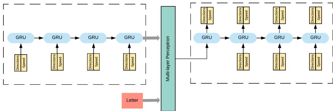
1 Training mode, using the teacher forcing methodology (Goodfellow et al., 2016; Williams and Zipser, 1989).
