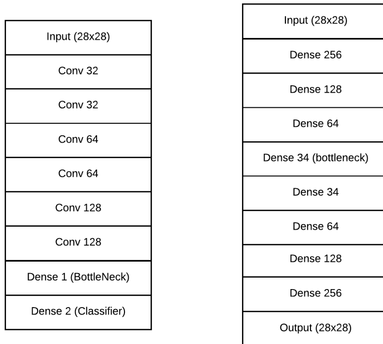
Figure 3.8: Left: architecture of the CNN letter classifier we used. Batch normalization is used after each convolution layer. The Dense 1 layer – with a size of 34 – is the embedding that is used to condition our generator. Right: the autoencoder architecture we used. The output of the first Dense 34 layer provides the latent space used to condition the generator.
