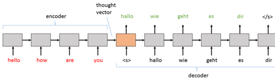
Figure 4.2: An illustration for a sequence-to-sequence architecture, used for language translation between English and German. The encoder summarize the English sentence, and the decoder use it as to bias its own output, to generate the equivalent German sentence.
