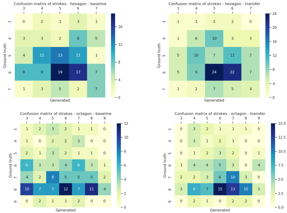
Figure 5.8: QuickDraw! Confusion matrix for strokes for both baseline (left) and transfer (right) models, on the different tasks. A small difference may appear in the total number between the baseline and the transfer confusion matrix is a result of us removing the column when it has a low/insignificant value (for aesthetic reason only, and to make the message focused).
