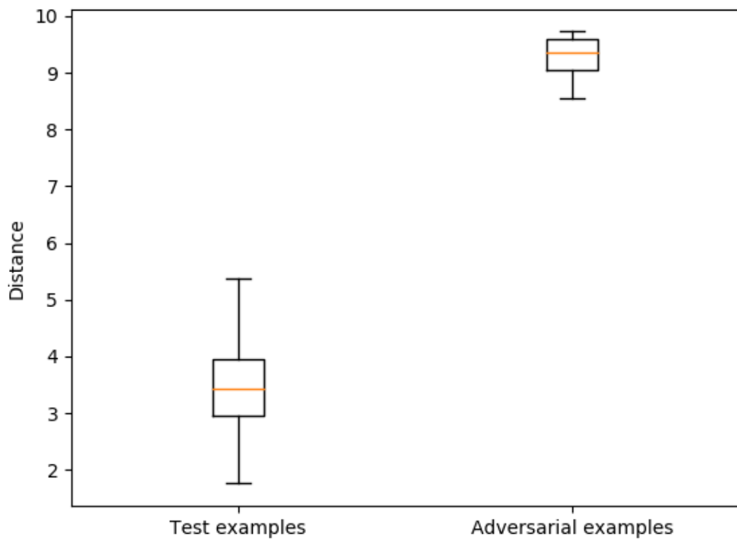
Figure C.8: KNN analysis: comparing the difference in the distance between the test data and the adversarial examples relative to the training data. We can see that the adversarial examples have a much higher distance than the test data.
