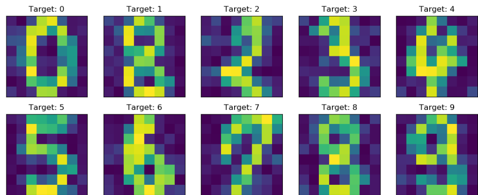
Figure C.10: KNN results after modifying the optimization objective: instead of only maximize the likelihood of the intended digit, I also added a penalty on the distance to the training data. The images are more relevant and comprehensible in this case.
