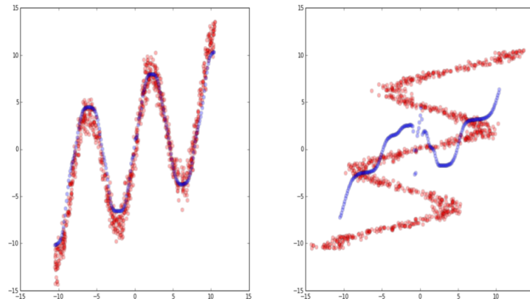
Figure 2.17: The performance of the simple linear activation function on two setups. Left: in case of one-to-one mapping between the input and the output, it performs well. Right: In case of one-to-many mapping, the function starts to average over the seen observations, leading to undesirable behavior. Source of this image is (Ha, 2015).
