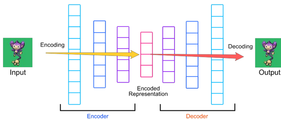
Figure 4.1: An example for the main components of an auto-encoder, used on image compression: an encoder takes the image, transfer it via a set of transformations into a bottleneck code, which is a compressed representation for that image. The decoder then takes this bottleneck code, and apply a series of transformations on it, in order to reconstruct the original input image. Source of this image is (Mohammed).
