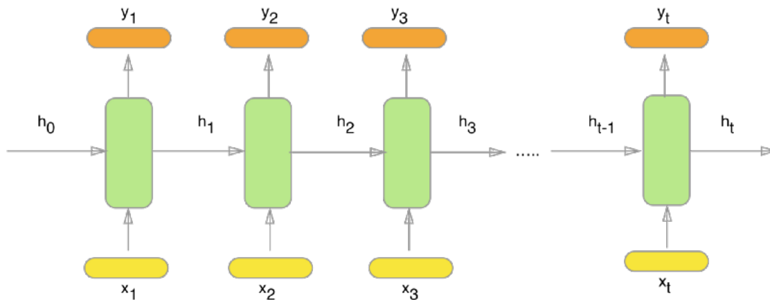
Figure 3.1: A demonstration of how RNN works: the network is applied on each token in the input ( x_1, x_2, \dots, x_t ), while update the hidden state variable every time ( h_0, h_1, \dots, h_t ). The output at each step is a function of the hidden state variable (not demonstrated here). Source of the image is from (Kostadinov, 2017).
