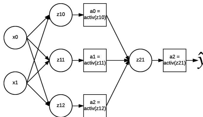
Figure 2.16: Example of a single-hidden layer neural network. The circle units is the sum of the weighted neurons connected to this unit, and the square units is the application of the activation function on that sum.
