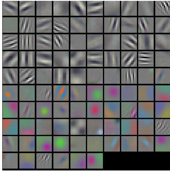
Figure 5.1: Visualization of the first convolution layer of a trained AlexNet. Note the basic shape of filters that resemble to Gabor filters widely used in image processing for decades (Fogel and Sagi, 1989; Jain and Farrokhnia, 1991). It is possible to see that those same filters will be useful in other computer vision or image-related tasks.
