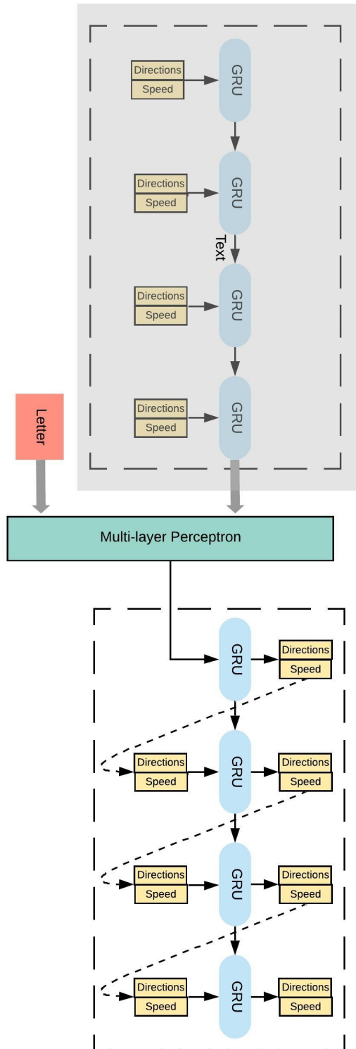
Figure 5.2: An illustration for model we use. The part identified by the gray area – the style extraction module – is what we transfer (i.e., what we freeze from the source task, and use in the target task). Since we give the model the task content/identity, the gray part is expected to focus more on the style extraction. During the exposure to the source task, all the different components of the model are being trained. During the exposure to the target task, the gray area is the trained one on the source task, with frozen parameters. The other parts will be trained.
