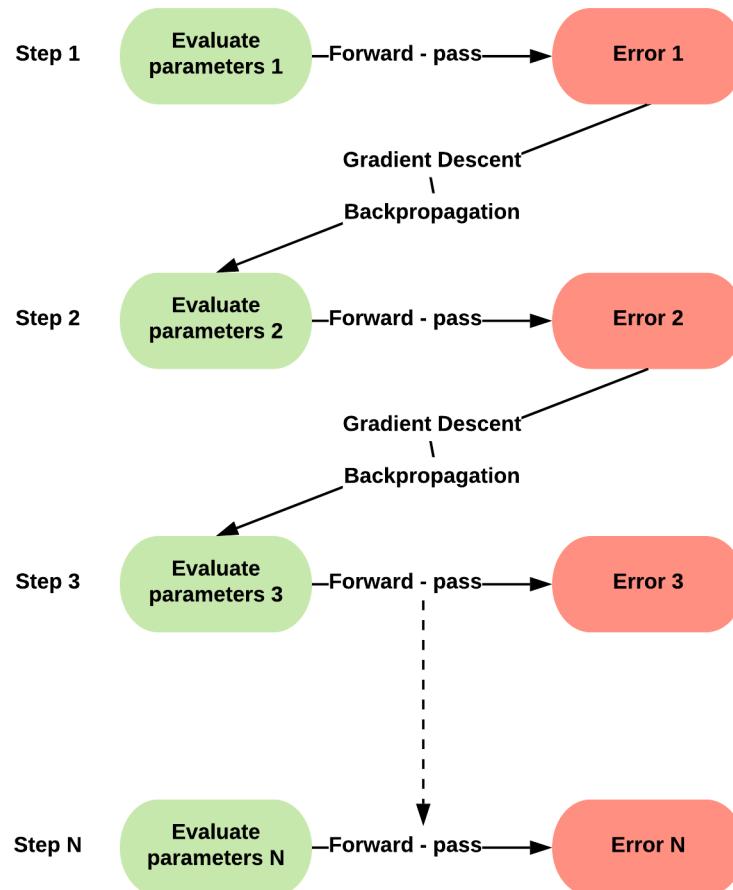
Figure 3.3: The process of gradient descent is iterative, and include 3 steps: evaluate the quality of the current parameters (forward-pass step), get the error value, use the error-value in order to update the parameters/getting new set of parameters ( Back-Propagation step). This process is repeated N times, which is decided by either not observing any update in the error, or we ran out of computational resources.
