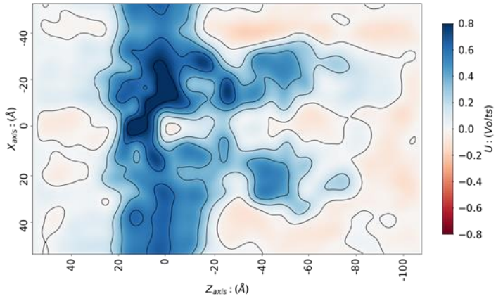
Electrostatic potential in the simulation box ( Y_{axis}=0 )
