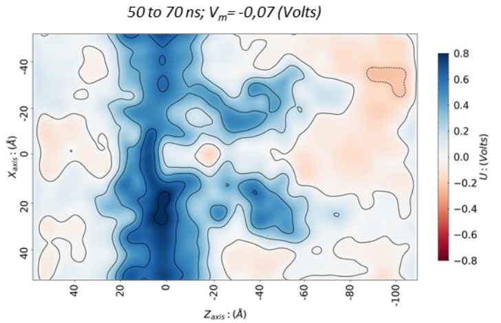
Electrostatic potential in the simulation box ( Y_{axis}=0 )
